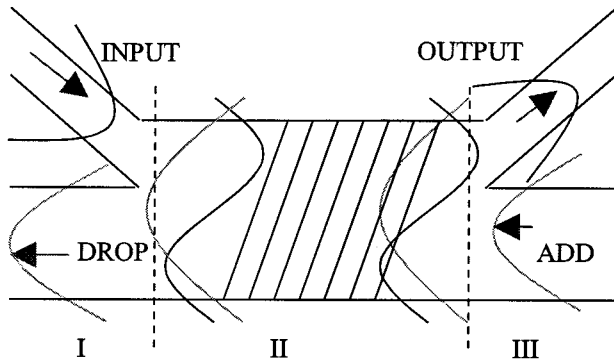
Fig. 1. Optical add-drop multiplexer: I, input Y branch; II, waist with tilted Bragg grating; III, output Y branch.
