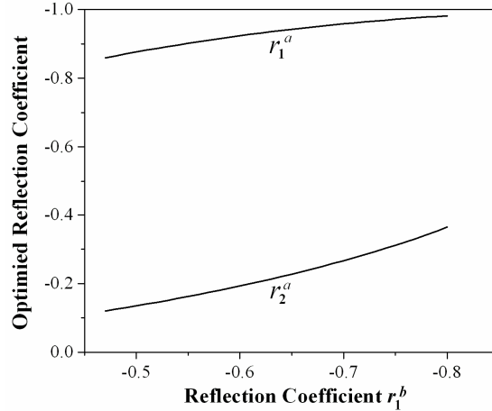
Fig. 11. Optimized reflection coefficients r_1^a and r_2^a and ripple as functions of reflection coefficient r_1^b for a 21-GTE interleaver.
