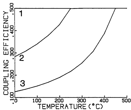
Fig. 5. Coupling efficiency of a multimode biconical fiber coupler as a function of temperature: r_2 = 5 \mu\text{m} ; z = 3500 \mu\text{m} ; L = 5000 \mu\text{m} ; t/r_2 = 0.1 ; \lambda = 0.633 \mu\text{m} ; n_0 = 1.0 ; L is the taper length; t is the thickness of the fusion section between two cases; and z is the length of the fusion section; 1, r_1 = 50 \mu\text{m} ; 2, r_1 = 100 \mu\text{m} ; 3, r_1 = 150 \mu\text{m} .
