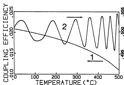
Fig. 6. Coupling efficiency of an ordinary parallel multimode uniform fiber coupler: r = 50 \mu\text{m} ; t/r = 0.005 ; 1, z = 3.5 \text{ mm} ; 2, z = 1000 \text{ mm} .
