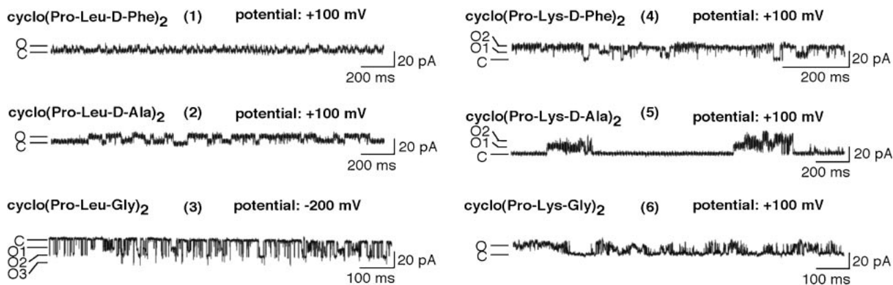
Figure 3. Representative profiles of ion conduction by peptides 1–6 . The experiment was carried out by pipette dipping patch clamp at 25 \pm 2 °C and data were filtered at 1 or 2 kHz frequency. The pipettes were filled with a 0.5 M KCl solution buffered with 5 mM HEPES (pH 7.4) containing 1 \mu M peptides. Symbols C and O (1, 2, 3, ...) denote the zero (closed) current level and open levels of channels, respectively.
