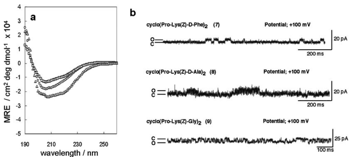
Figure 5. The biophysical properties of peptides 7–9 . (a) CD spectra of the peptides. CD spectra were collected in the presence of 2 mM DPPC SUVs. Symbols represent peptide 7 (open triangle), peptide 8 (open circle), and peptide 9 (open square), respectively. No significant changes of the spectra were observed by the side chain protection. (b) Representative patterns of ion conduction by these peptides. In peptides 7–9 , the characteristic conductance profiles of the corresponding peptides 4–6 were converted to considerably lower conductance values and different open close transitions by protecting \epsilon amino group.
