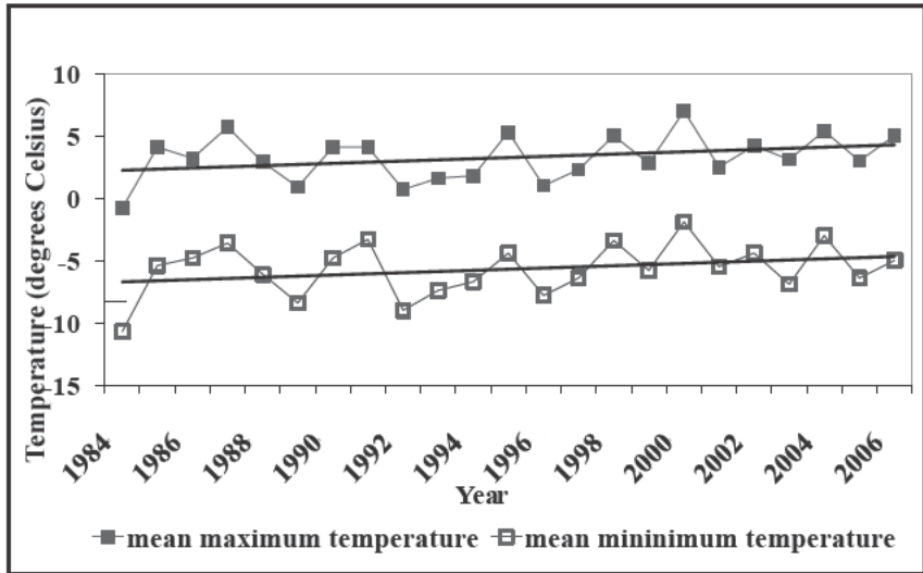
Figure 9. Short-term mean maximum and minimum temperatures for March (first boil), Kingston
