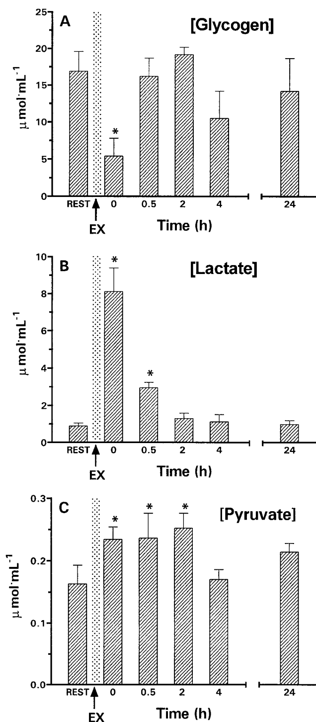
Figure 5. Changes in the whole-body concentrations of (A) glycogen, (B) lactate, and (C) pyruvate of ammocoetes following 5 min of vigorous chasing. The vertical stippled bar represents the period of exercise (EX). All data expressed as the mean \pm 1 SEM ( N = 6 at each sample period). Asterisks indicate statistically significant differences between resting and postexercise concentrations ( P < 0.05 ).
