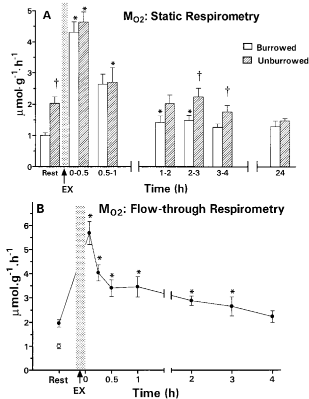
Figure 1. Changes in the oxygen consumption rates ( \text{Mo}_2 ) of ammocoetes of the sea lamprey ( Petromyzon marinus ) following 5 min of vigorous chasing as measured using (A) static respirometry or (B) flow-through respirometry. A, Open and hatched bars represent the \text{Mo}_2 of burrowed ( N = 8-21 ) and unburrowed ammocoetes ( N = 6-10 ), respectively. B, All ammocoetes ( N = 9 ) were unburrowed (filled circles), but note that the resting \text{Mo}_2 of burrowed ammocoetes is included for reference (open circle). The vertical stippled bar represents the period of exercise (EX). All data expressed as the mean \pm 1 SEM. Asterisks indicate statistically significant values from resting (control) rates, while daggers represent statistically significant differences between the \text{Mo}_2 of burrowed versus unburrowed ammocoetes during the same sample period ( P < 0.05 ).
