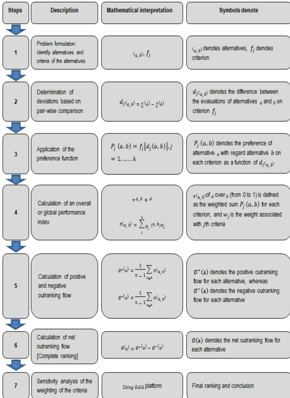
Figure 4.4: General steps of the procedure of PROMETHEE. Source: Based on Behzadian et al. (2010) and PROMETHEE 1.4 Manual (2013).
