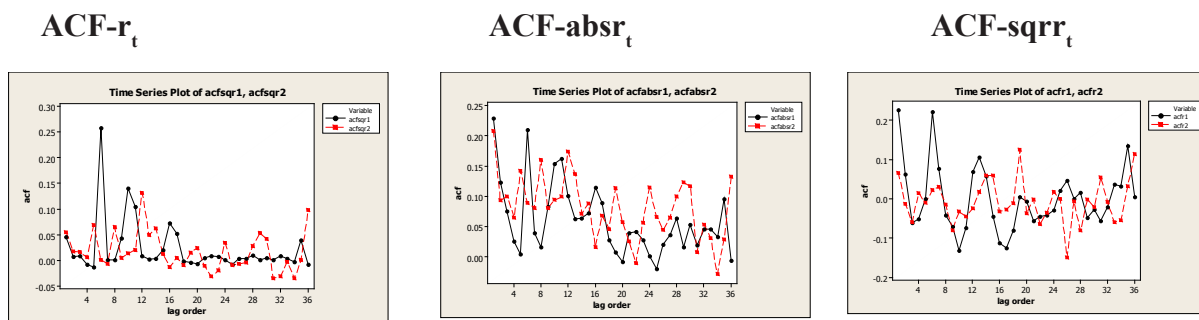
Figure -10 Autocorrelation Function of Return, Absolute Return and Squared Return Series
