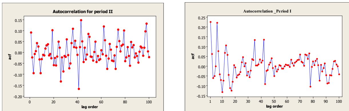
Figure 9: Autocorrelation Function of Return Series
