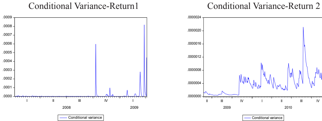
Figure 13- Conditional Variance of Return Series
