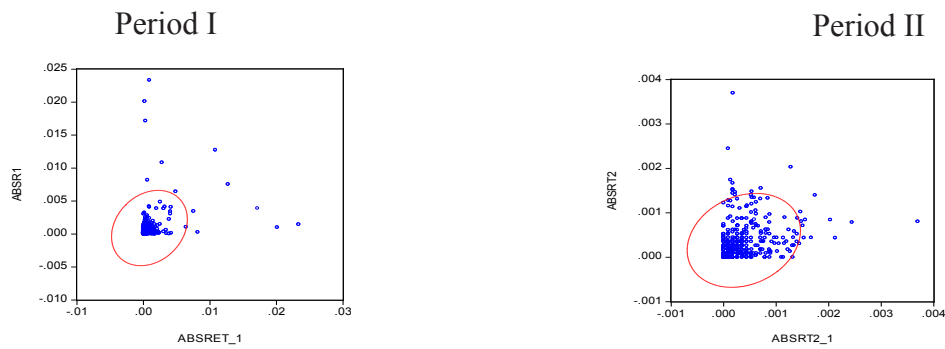
Figure 15- Scatter plot of the absolute return on day t against the return on day t-1
