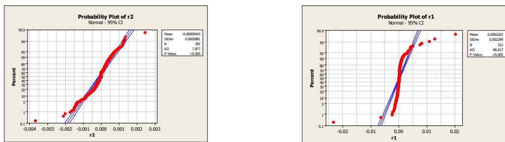
Figure 11- Probability plot of returns
