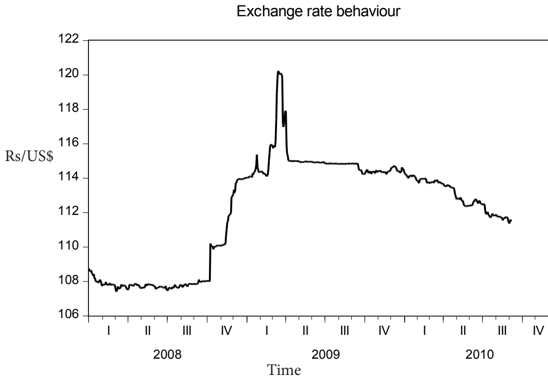
Figure 1: Exchange rate behavior in level form
