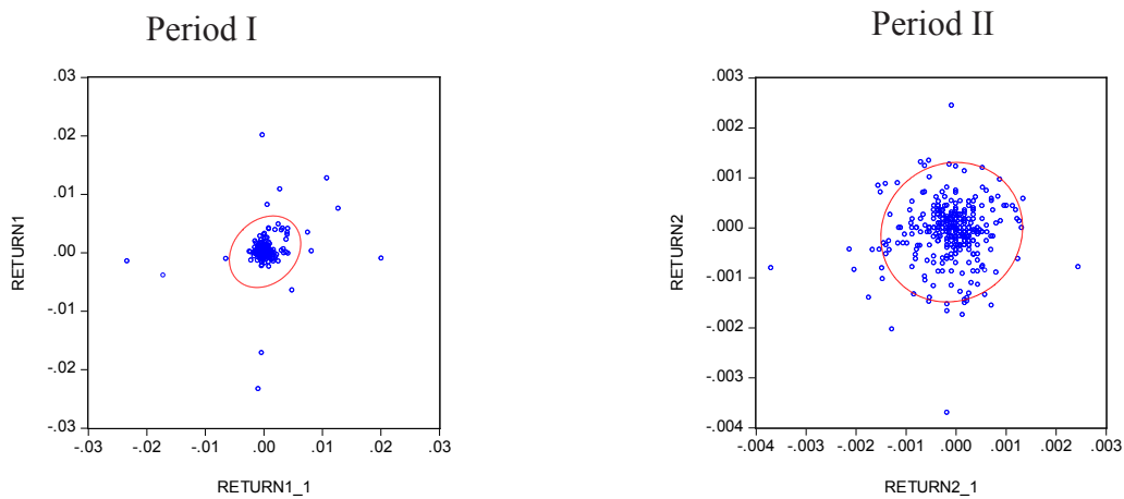
Figure 14 Scatter Plot of the Return on day t against the return on day t-1 with Confidence Ellipse
