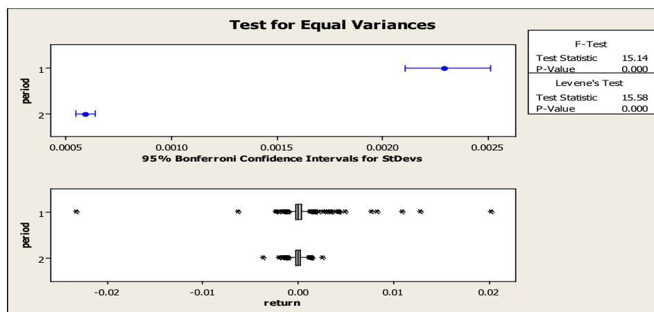
Figure 6 Variability of the Distributions
