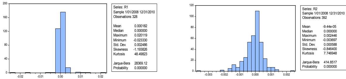
Figure 4 Descriptive Statistics of Return Distributions
