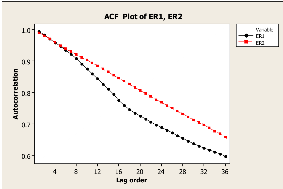
Figure 7 ACF of Exchange Rate Series
