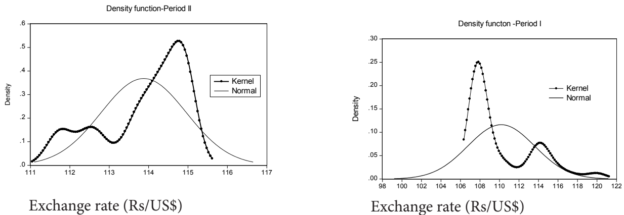
Figure- 2 Density function of exchange rates, ER1 and ER2
