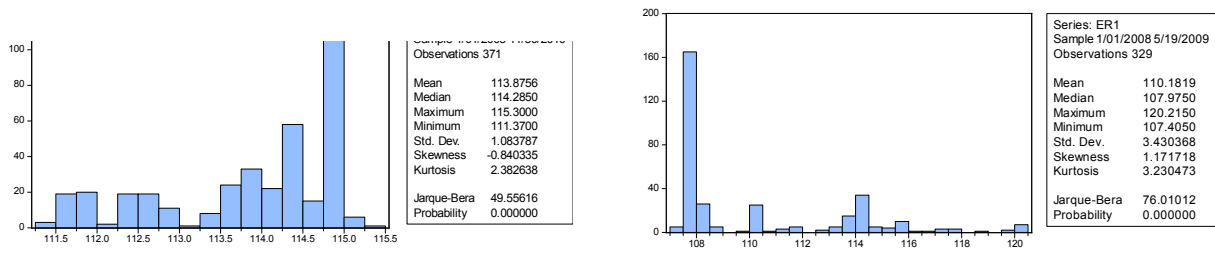
Figure-3 Summary statistics of exchange rate distributions
