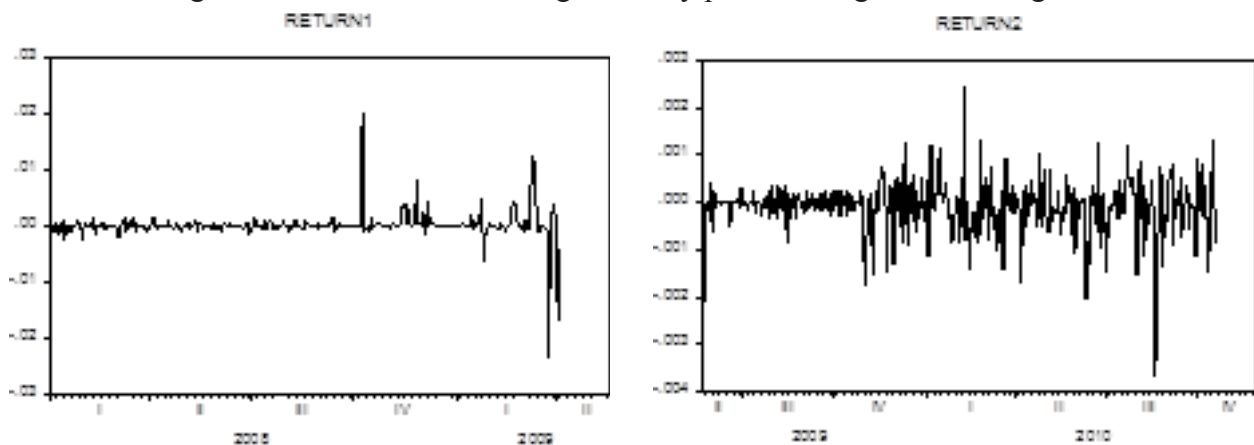
Figure-4 Exchange rate behavior in return
