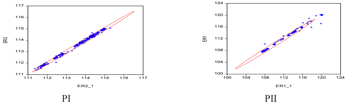
Figure 8: Confidence ellipse
