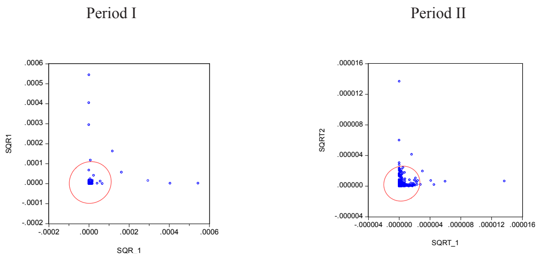
Figure 15- Scatter plot of the squared return on day t against the return on day t-1
