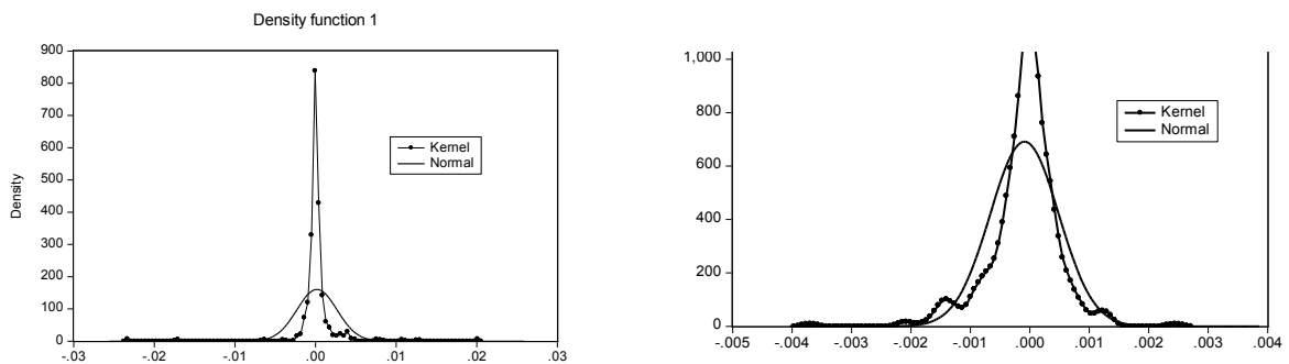
Figure 5 Comparison of Empirical Return (kernel) Density Functions
