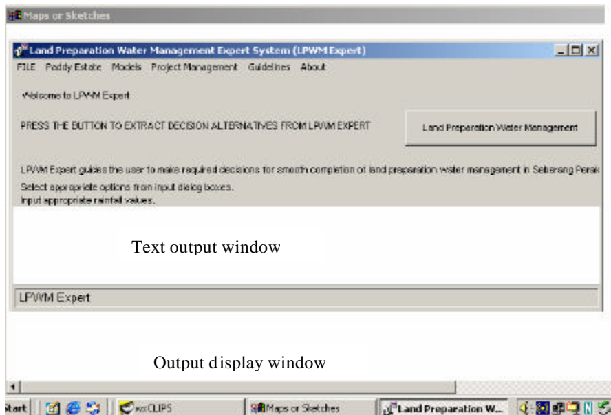
Fig 3. User interface of LPWM Expert
