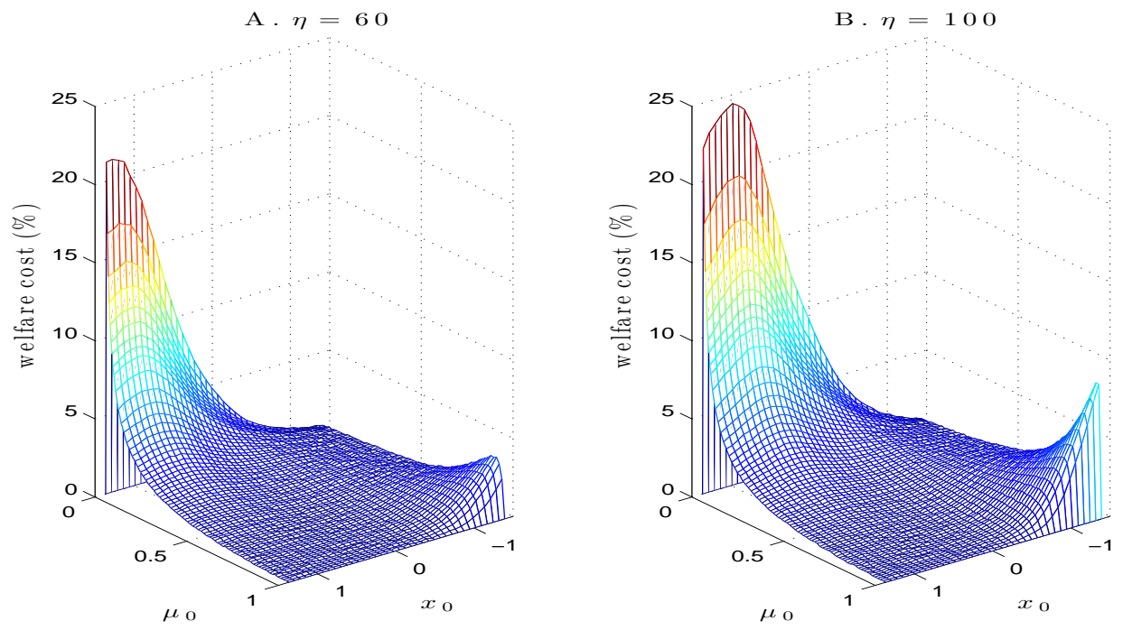
Figure 7: Welfare cost. This figure plots the conditional welfare costs of an ambiguity averse investor with horizon T = 40 years if he follows the Bayesian strategy. The conditional welfare cost is a function of the belief of the IID model \mu_0 and the demeaned dividend yield x_0 . We set \gamma = 5 .
