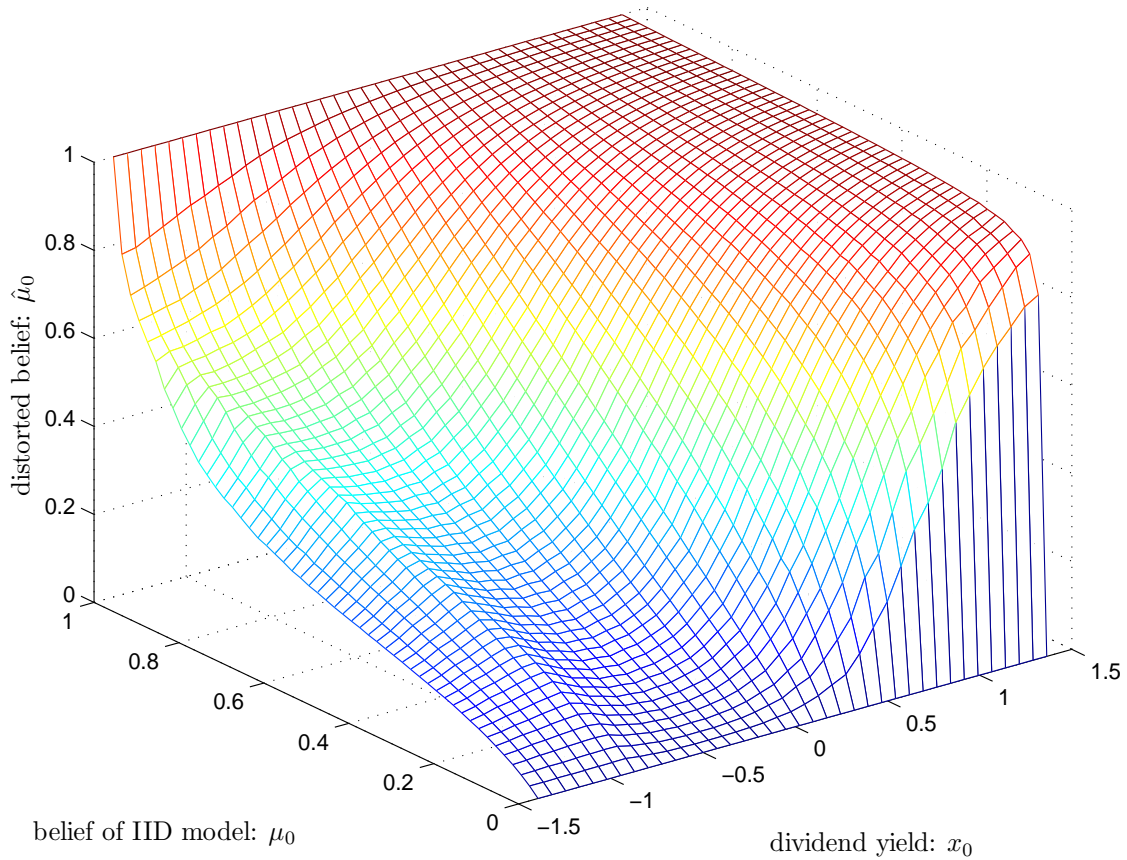
Figure 3: Distorted beliefs of the IID model. This figure plots the distorted belief of the IID model as a function of the Bayesian belief of the IID model \mu_0 and the demeaned dividend yield x_0 for an ambiguity averse investor with horizon T = 40 years.
