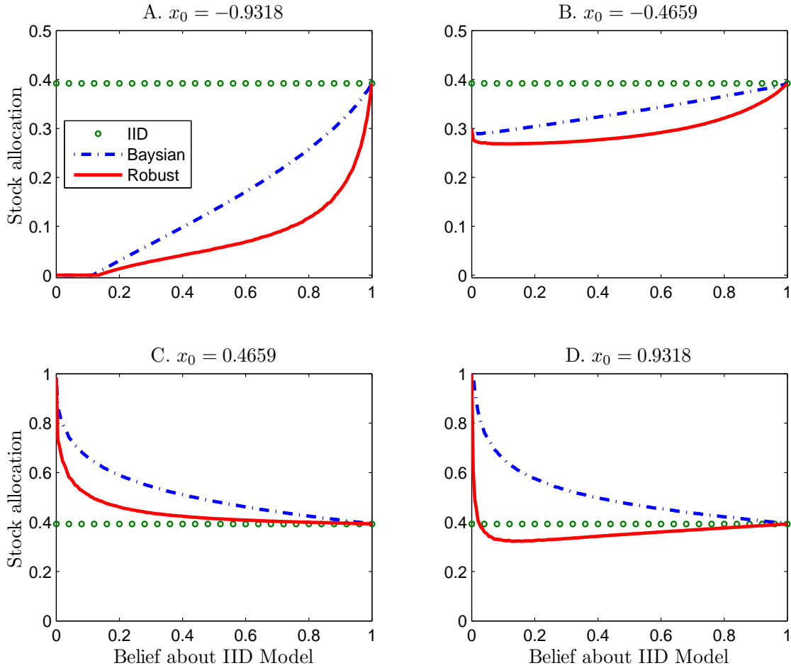
Figure 5: Alternative investment strategies: uncertainty effect. This figure plots the portfolio weights on the stock for three alternative investment strategies as functions of the initial beliefs about the IID model \mu_0 for four different initial values of the demeaned log dividend yield x_0 . The standard deviation of the stationary distribution of x_t is 0.4659. We set the risk aversion parameter \gamma = 5 and the investment horizon T = 40 . Other parameter values are estimated using annual data as reported in Table 2.
