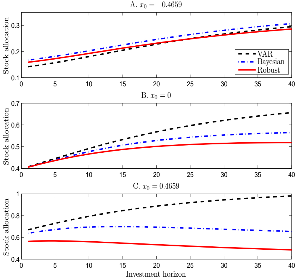
Figure 6: Alternative investment strategies: horizon effect. This figure plots the portfolio weights on the stock for three alternative investment strategies as functions of the investment horizon. The standard deviation of the stationary distribution of x_t is 0.4659. We set the risk aversion parameter \gamma = 5 and the initial belief \mu_0 = 0.1 . Other parameter values are estimated using annual data as reported in Table 2.
