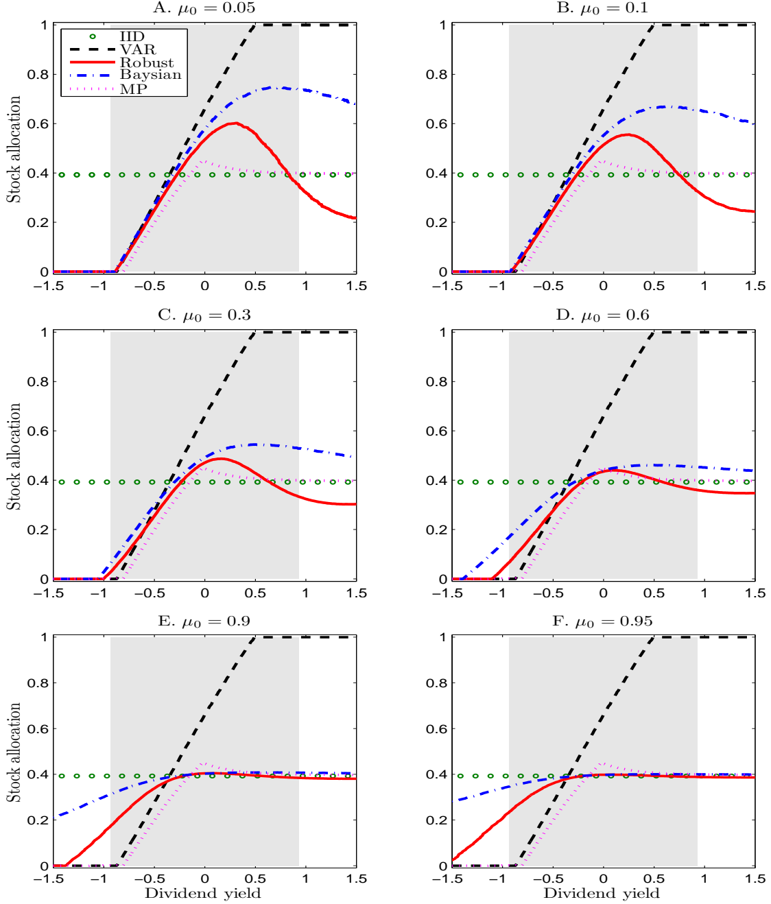
Figure 4: Alternative investment strategies: market-timing effect. This figure plots the initial portfolio weights on the stock for five alternative investment strategies as functions of the initial observation of the demeaned log dividend yield x_0 for different initial beliefs about the IID model \mu_0 . We set the risk aversion parameter \gamma = 5 and the investment horizon T = 40 . Other parameter values are estimated using annual data as reported in Table 2. The standard deviation of the stationary distribution of x_t is 0.4659. The shaded area denotes the region where log dividend yield is within 2 standard deviations from the mean.
