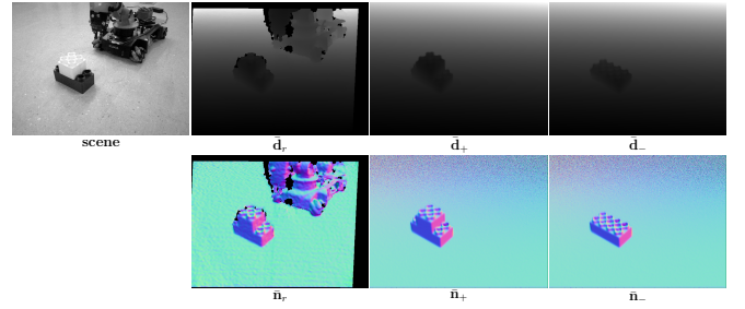
Fig. 6: Depth and surface normal means. The grayscale scene image shows the assembly scene after the assembly robot attached the new block (bright block) to the work-in-progress block (dark block). The depth \bar{\mathbf{d}}_r and surface normal \bar{\mathbf{n}}_r means are estimated from a set of real depth images \mathcal{D}_r . Once the current pose estimate \mathcal{P} = \{\bar{\mathbf{X}}_0, \Sigma_0\} is calculated from ICP, virtual PGNMs are estimated. Here only mean depth ( \bar{\mathbf{d}}_+ , \bar{\mathbf{d}}_- ) and normal ( \bar{\mathbf{n}}_+ , \bar{\mathbf{n}}_- ) are shown. Note artificially added depth noises which is more noticeable in normal mean images.
