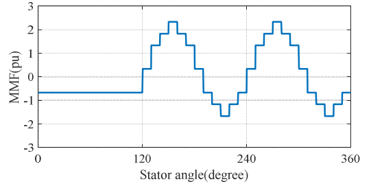
Fig. 32. MMF in open circuit condition.
