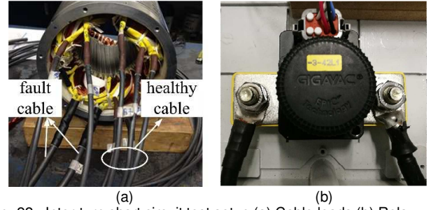
Fig. 22. Inter-turn short circuit test setup (a) Cable leads (b) Relay.
