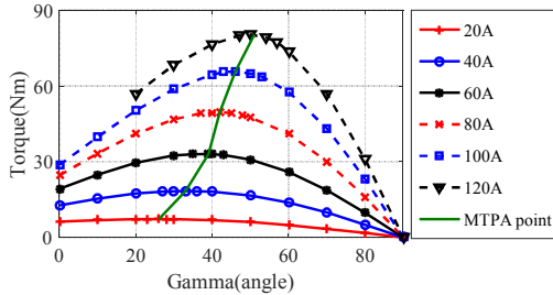
Fig. 11. Torque variations with current magnitude and gamma angle.
