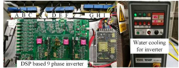
Fig. 4. DSP based 9-phase inverter.
