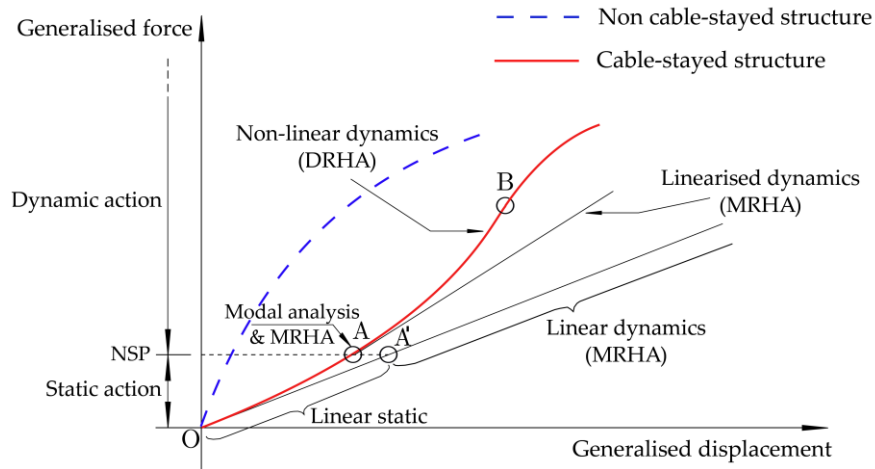
Figure 1. Qualitative difference between the load-displacement response of classical cable-stayed bridges and structures without cable-system.
