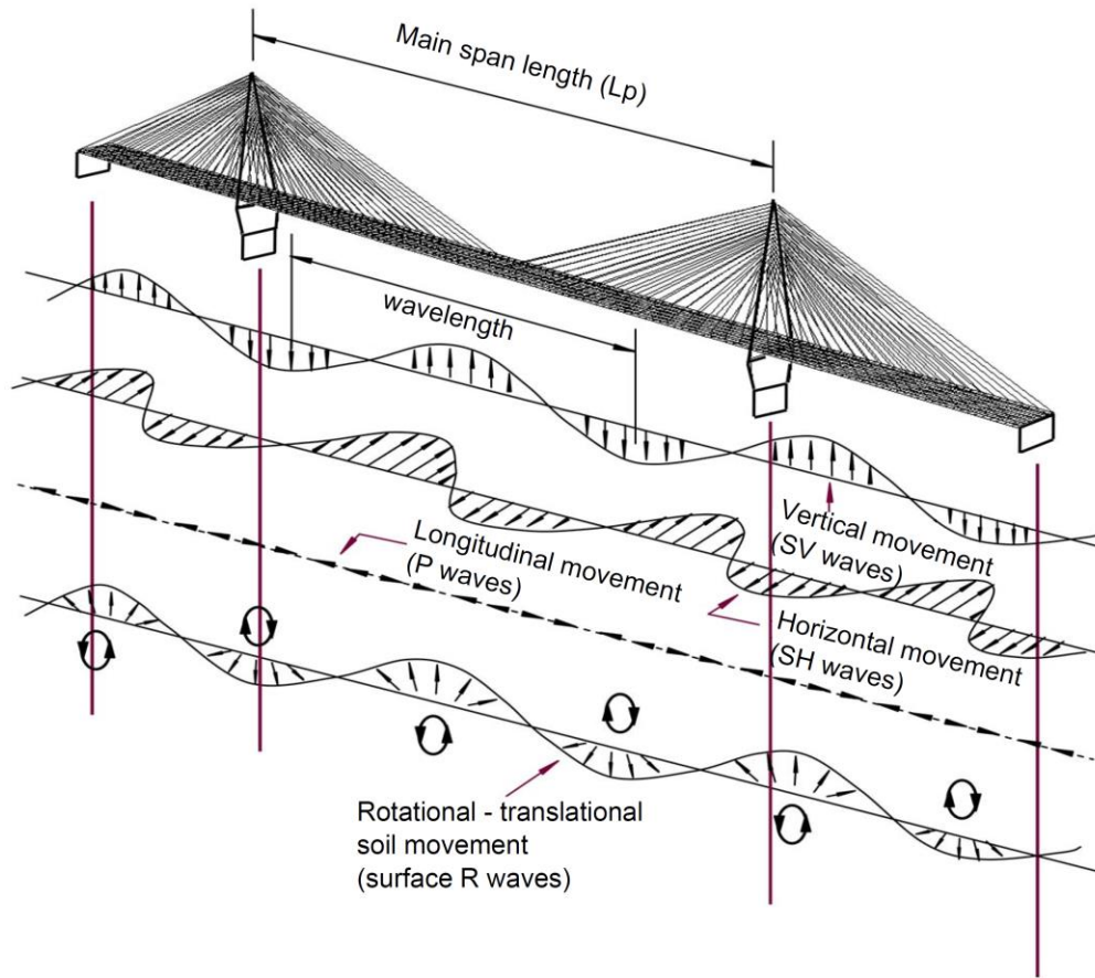
Figure 2. Different types of seismic waves exciting the supports of a long cable-stayed bridge. Adapted from from [2] [51].
