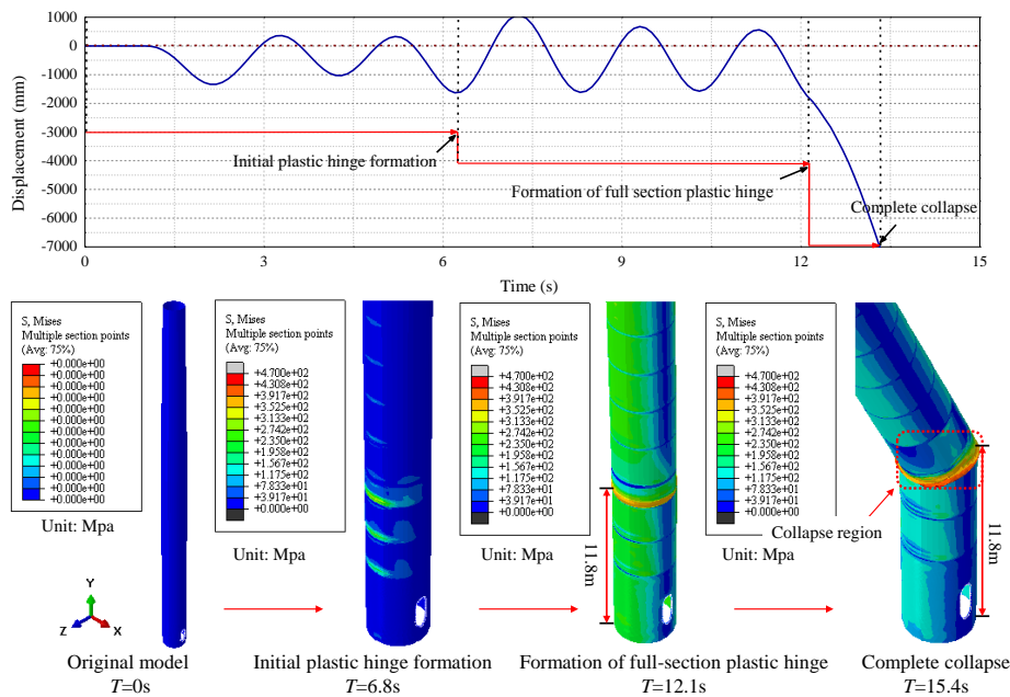
Fig. 12 Top displacement time history and the corresponding von Mises stress (MPa) distribution of FE model for the loading case of V_{hub}=55 m/s, 90^\circ inflow direction
