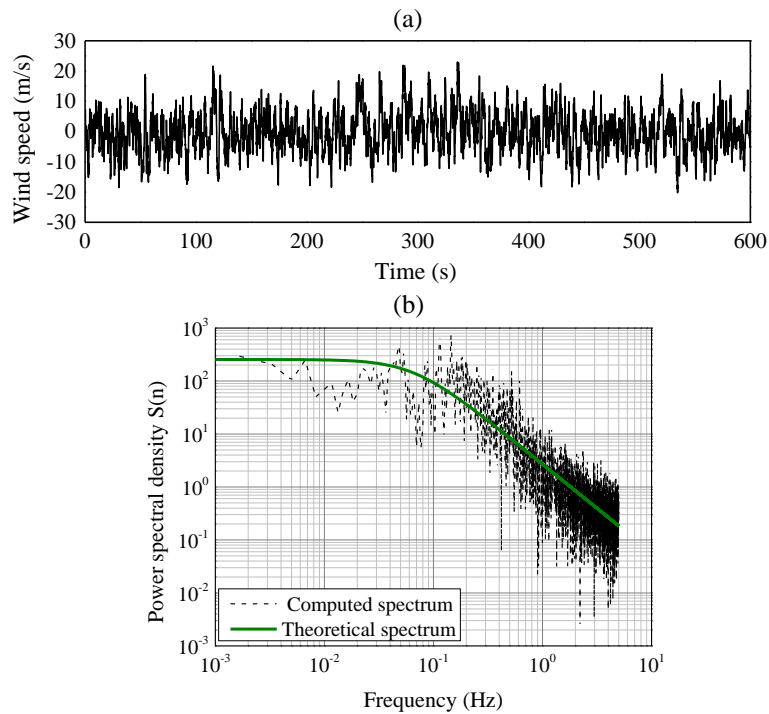
Fig. 4 Wind velocity simulation results: (a) wind velocity time-history and (b) computed and theoretical (Von Karman) wind spectra
