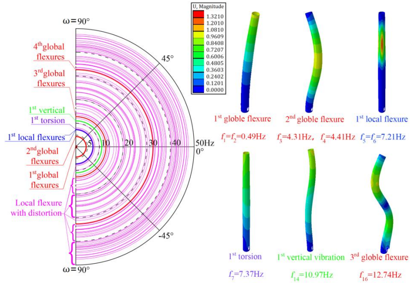
Fig. 3 Polar plot of the first 100 frequencies f (Hz) against the nacelle orientation ( ^\circ ) with several typical vibration mode shapes (the left side of the polar plot is not included because it is symmetric)
