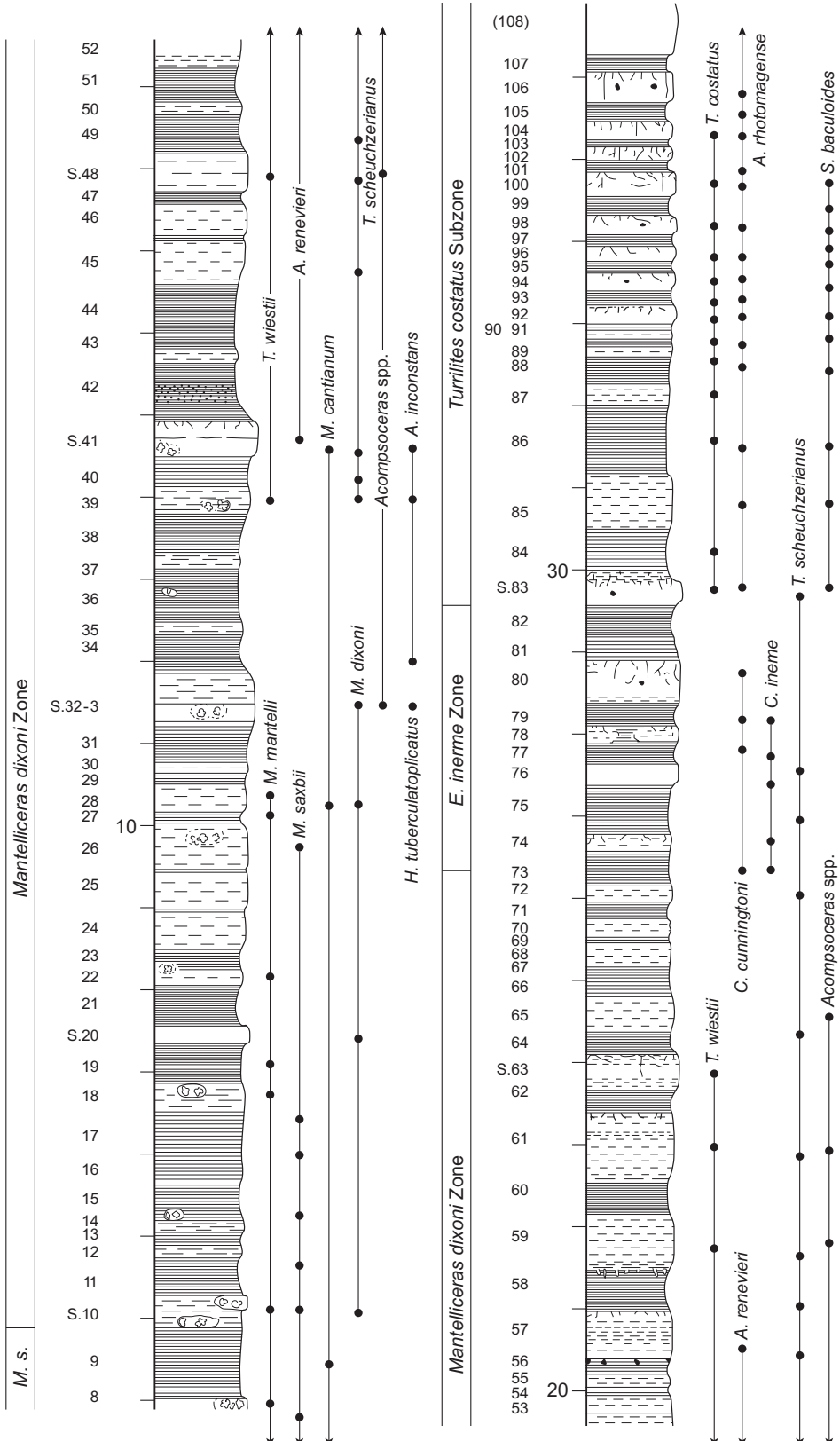
Text-fig. 9. The succession, and selected ammonite occurrences across the Lower-Middle Cenomanian boundary in the Southam Grey Pit Brought to you by | University of Portsmouth Download Date | 12/19/17 11:11 AM
