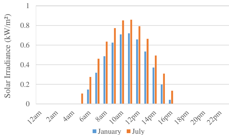
Figure 8. Variation in theoretical hourly solar irradiance on a surface sloped at the angle of latitude for Jarreng on indicative days in January and July
