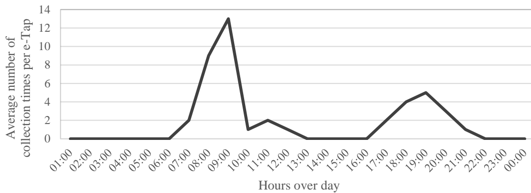
Figure 7. Hourly withdrawal variability of 28 e-Taps over one day in Jarreng
