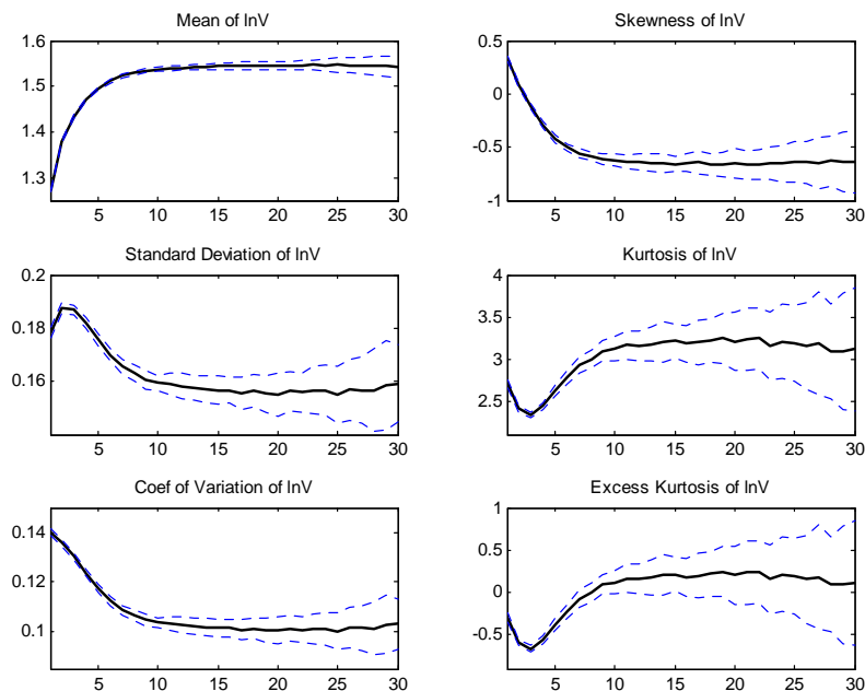
Figure 6b: Moments of cross-sectional log firms value, by age
