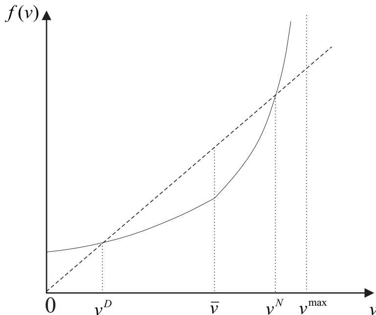
Figure 2: Co-existence of Default and No-Default Equilibria
