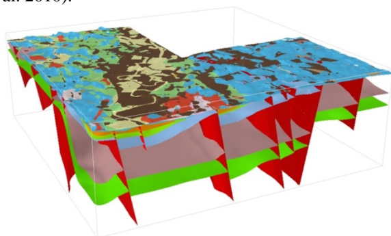
Figure 2. Bedrock and superficial deposits 3D model of south-east Glasgow looking north-west down the River Clyde. Model dimensions 10 x 10 km x 1 km deep, x3 vertical exaggeration.
