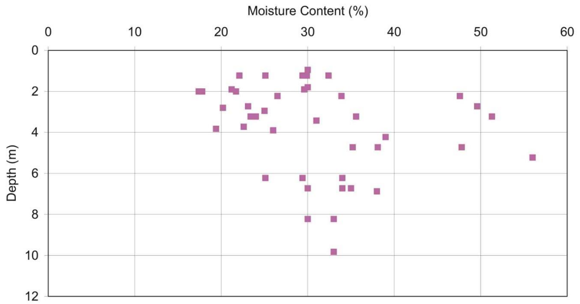
NS66SW: Moisture content profile: Gourock Formation
