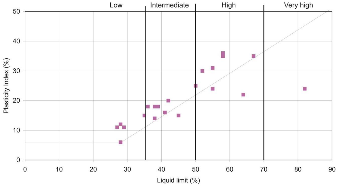
NS66SW: Plasticity chart: Gourock Formation
