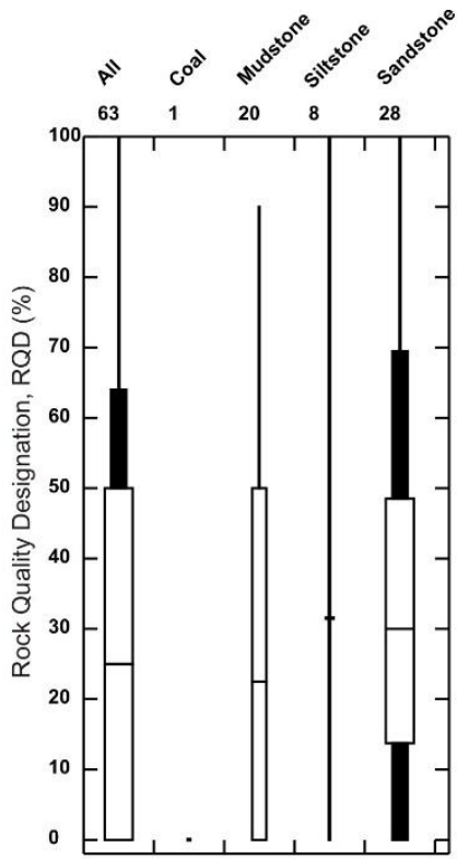
Extended Whisker plot for Passage Formation Rock Quality Designation (RQD) by lithology
