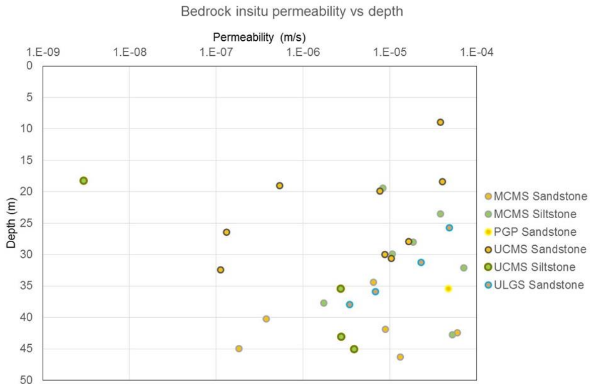
Figure 53 In situ permeability values vs depth for the Clyde Gateway area
