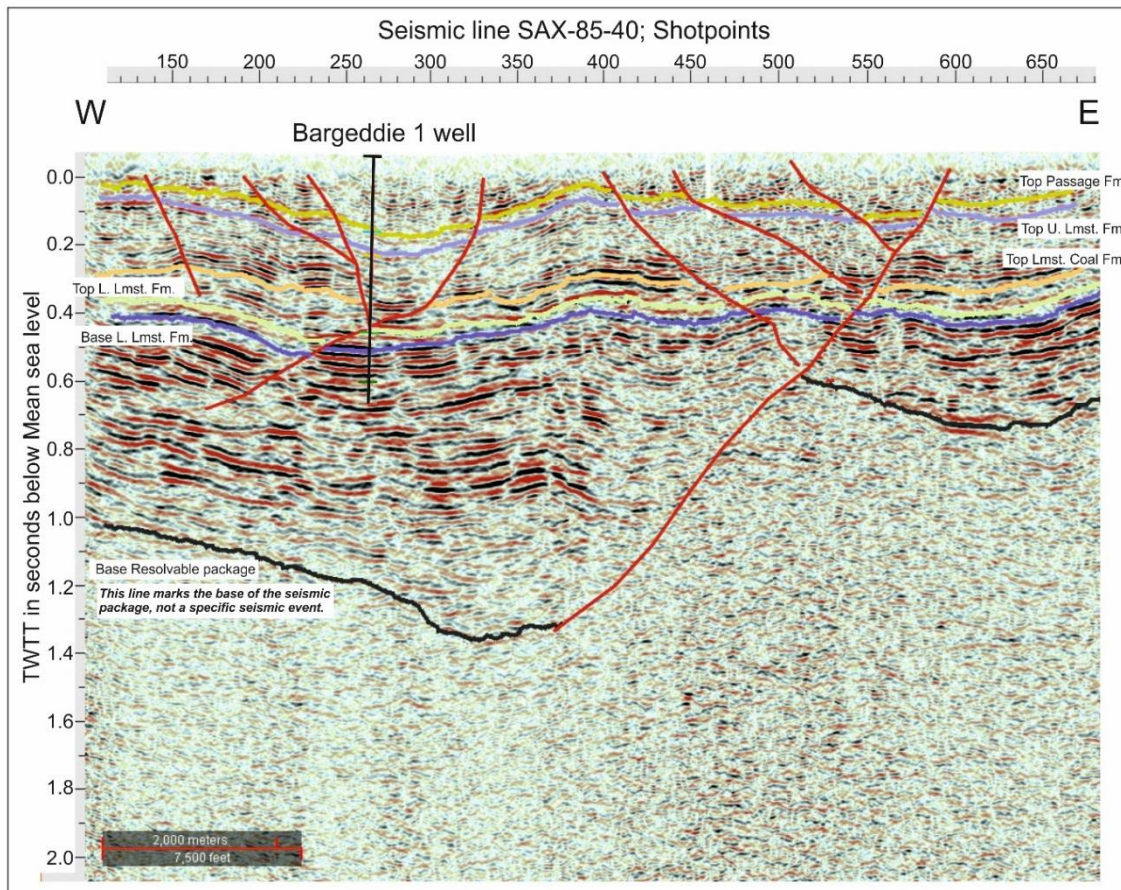
Figure 11 Detail from seismic profile SAX-85-40 showing location of Bargeddie 1 exploration well and interpreted seismic events. Seismic data reproduced with permission of UKOGL.
