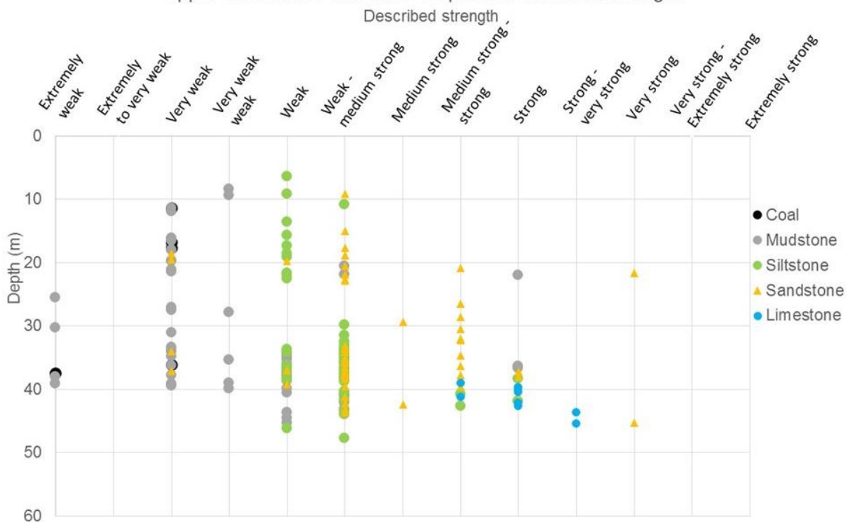
Upper Limestone Formation - Depth and described strength
