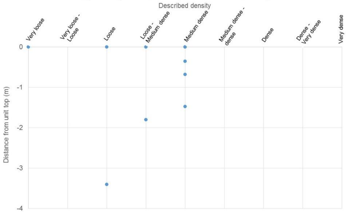
Clyde Valley Formation - Depth and described density
