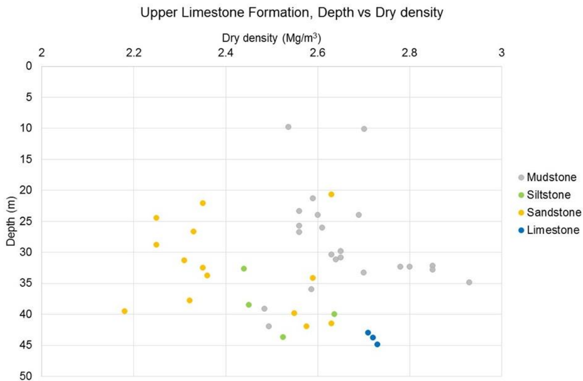
Figure 58. Upper Limestone Formation, the dry density at depth below ground level
