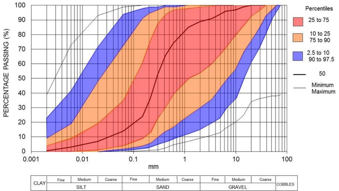
Particle size distribution - Gourock Formation 403 samples
