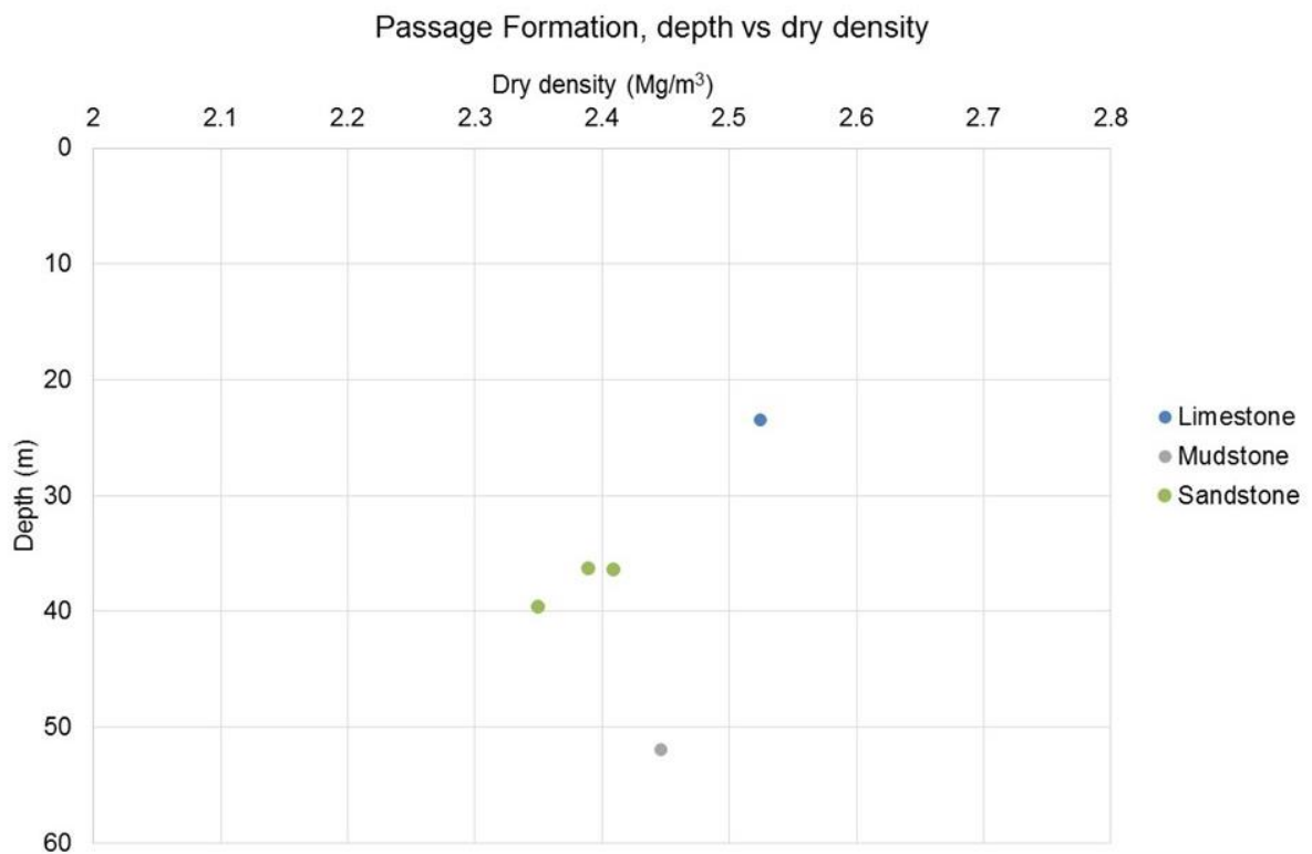
Figure 57. Passage Formation, the dry density at depth below ground level
