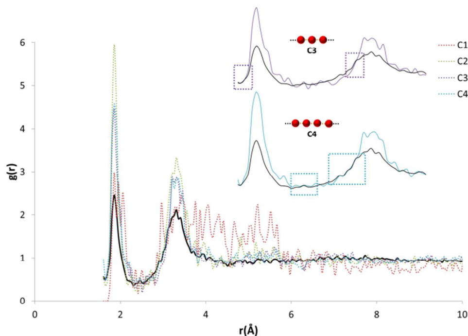
Fig 5 – An example of the initial overlay analysis of motif RDFs with the original HW-OW RDF. Discrete features for both the C3 (purple) and C4 motif (blue) appear to be present in the original function. Other discrete chain motifs are also represented here, as indicated by the legend (top right).
