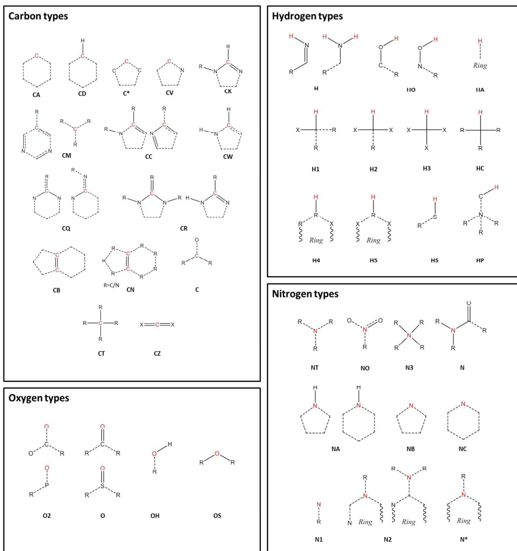
Fig. 1 – Schematic representations of AMBER atom types. The red colour represents the atom being typed. The code below each schematic refers to the code assigned by the AMBER routine. R groups represent any atom, and X groups represent either N or O. Dotted lines represent undefined bond order, and solid lines represent conventional nomenclature of bonds.
