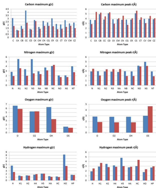
Fig. 6 – The maximum peak (defined by g(r) ) for each RDF pair profile (each atom type with HW and OW) was determined. These bar graphs show the g(r) value for the maximum peak of each atom type with OW (blue bars) and HW (red bars) on the left, with the distance at which these peaks were found plotted on the bar graphs on the right.
