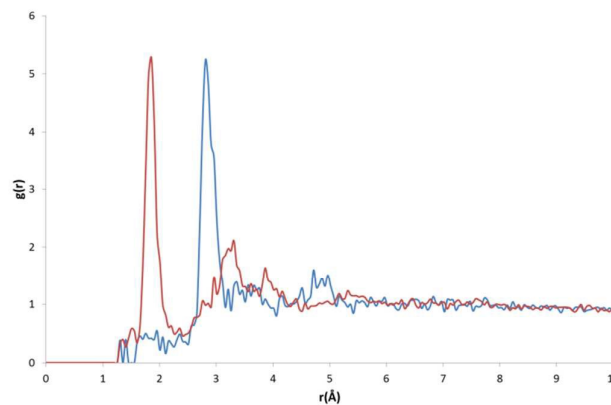
Fig. 10 – RDFs for the O2 atom type with OW (blue) and HW (red)
