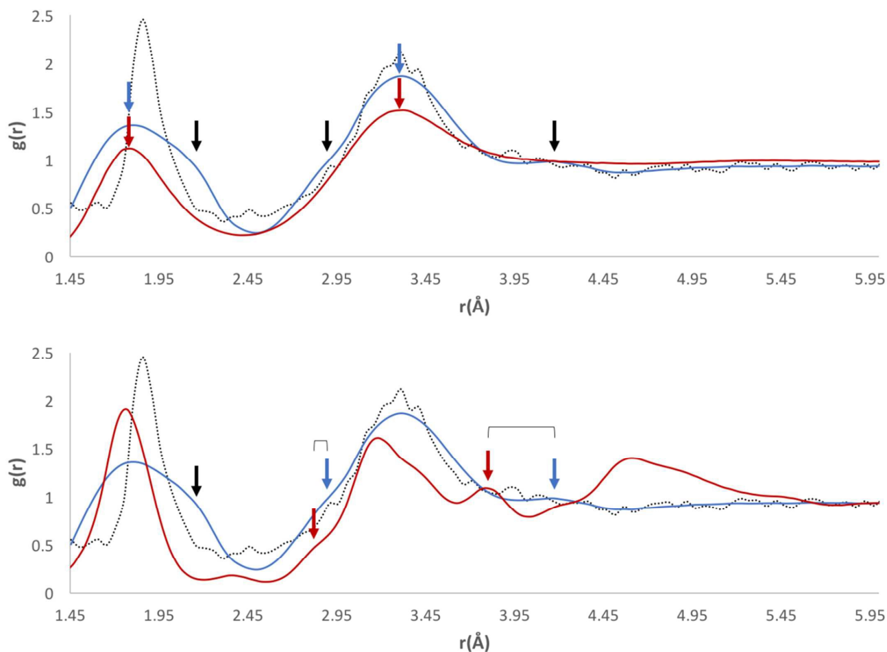
Fig. 3 – A comparison of the short-range interactions in our RDF for OW + HW pairs (original data shown as dotted black lines, smoothed data shown in blue) with Soper's RDF of water at 298K (shown in red on the top plot) and ice at 220K (shown in red on the bottom plot). The black arrows on both plots represent peaks or features in our RDF which cannot be explained by the comparative Soper plot. The blue and red arrows indicate comparable peaks, with their colour corresponding to the same coloured plot line.
