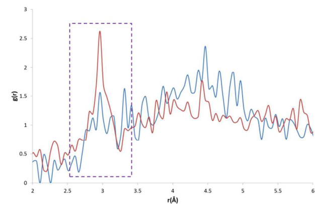
Fig. 8 – CC-HW RDF (blue) and CK-HW RDF (red) with a much larger peak apparent at \sim 3 \text{ \AA} in the CK-HW profile (outlined in purple).
