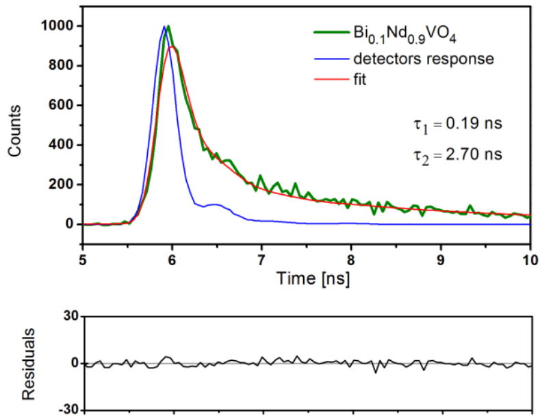
Fig. 37 The green line shows the time-domain intensity decay of \text{Bi}_{0.1}\text{Nd}_{0.9}\text{VO}_4 powder. \lambda_{\text{em}} = 522 nm. The red line is the fitting curve and the blue line is the response of the detector. The residuals represent the difference between the fitted curve (red line) and the measured data. The goodness of the fit, \chi^2 , is 2.051.
