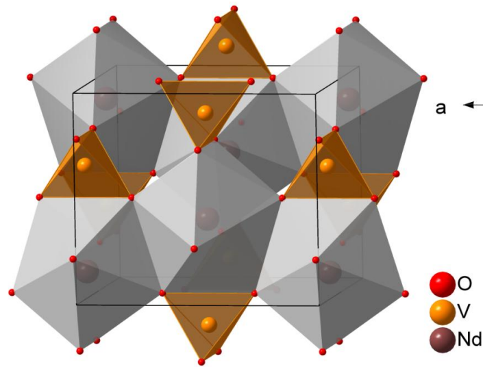
Fig. 9 The zircon structure adopted by \text{NdVO}_4 at ambient conditions.
