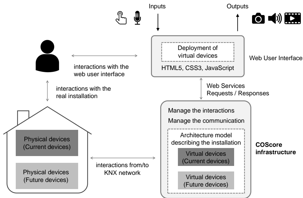
Figure 1: Schema of the approach for emulating home automation installation
