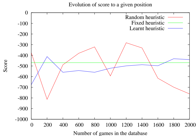
Fig. 7. Evolution of the heuristic as the size of the database grows
