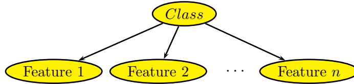
Fig. 2. Structure of a Naive Bayes classifier
