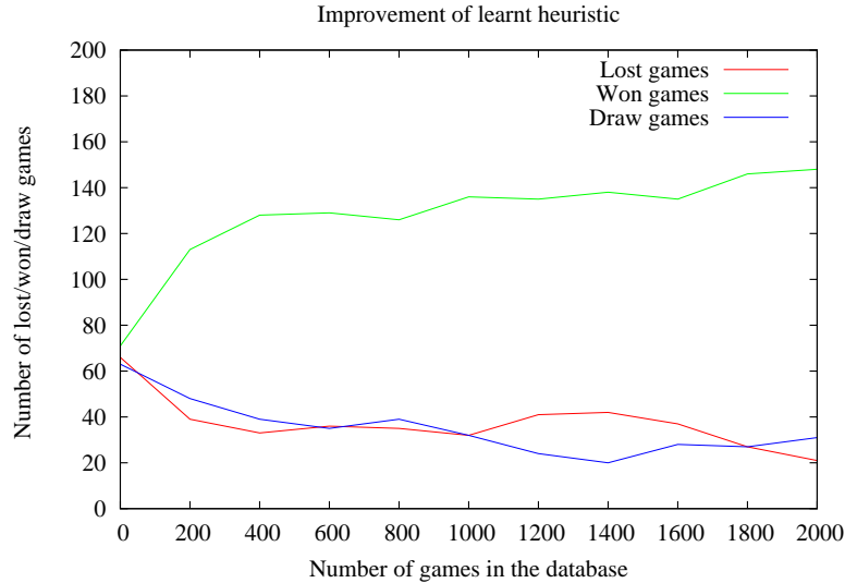
Fig. 5. Evolution of the results of playing the learnt heuristic against the random one
