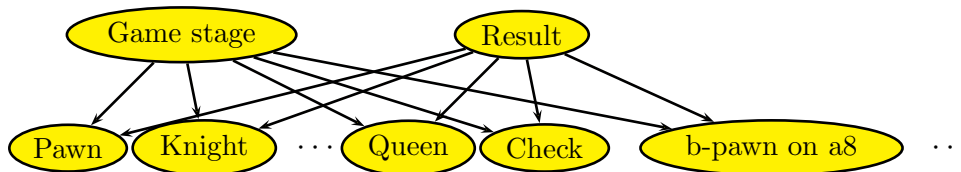
Fig. 3. Structure of the network used to learn the heuristic
