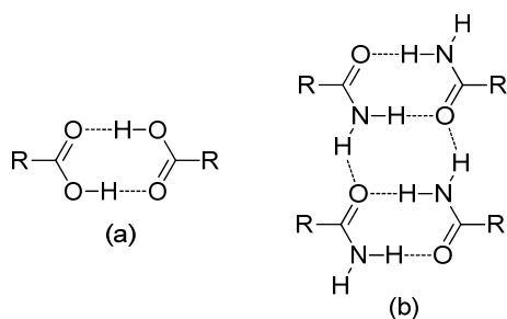
Scheme 1. (a) Hydrogen-bonded R_2^2(8) dimer in carboxylic acids; (b) Hydrogen-bonded infinite C(4) R_4^2(8) ribbons in amides
