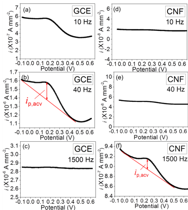
Figure 1. Comparison of AC voltammograms (ACVs) measured at 10, 40 and 1500 Hz of H 2 N-(CH 2 ) 4 -CO-Ala-Ala-Asn-Leu-NHCH 2 -Fc immobilized on a macro-GCE (a–c) and on a VACNF NEA (d–f). All the measurements were done in 500 \mu L of 50 mM MES (pH 5.0) and 250 mM NaCl. Sinusoidal waves with the fixed amplitude of 25 mV were superimposed on a DC staircase ramp from -0.05 to +0.65 V at a scan rate of 10 mV \cdot s -1 . The measured average AC current at each point was normalized by the 7.1 mm 2 geometric surface area defined by the 3-mm i.d. O-ring. The actual CNF surface area is \sim 100 times less.
