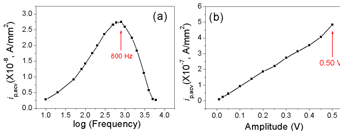
Figure S6. (a) Background-corrected ACV peak current density i_{p,acv} (normalized to the 7.1 \text{ mm}^2 geometric electrode area) of \text{H}_2\text{N}-(\text{CH}_2)_4\text{-CO-Leu-Arg-Phe-Gly-NH-CH}_2\text{-Fc} immobilized on a VACNF NEA plotted against the logarithm of the frequency. (b) Background-corrected ACV peak current density i_{p,acv} (normalized to the 7.1 \text{ mm}^2 geometric electrode area) of \text{H}_2\text{N}-(\text{CH}_2)_4\text{-CO-Leu-Arg-Phe-Gly-NH-CH}_2\text{-Fc} immobilized on a VACNF NEA plotted against the amplitude. All the measurements were done in 250 \mu\text{L} of 25 \text{ mM} MES (pH 5.0). Note: The real CNF surface area is \sim 100 times less than the geometric surface area defined by the O-ring.
