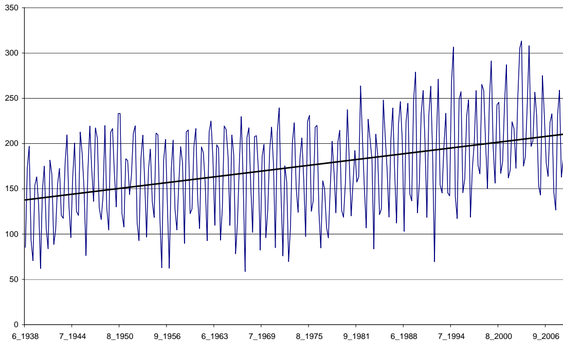
Figure 3b. Evolution of HDD index in summer months
