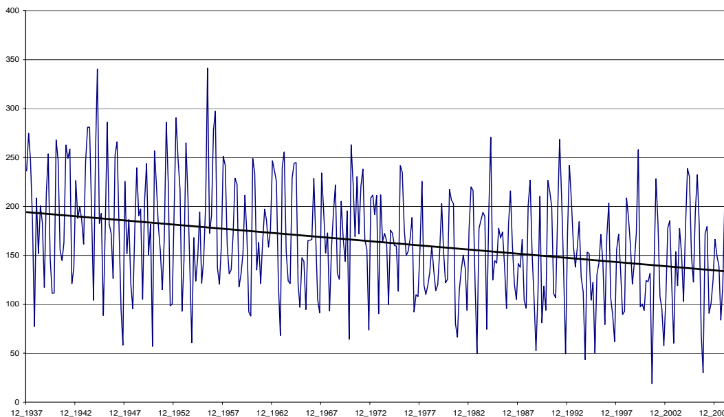
Figure 3a. Evolution of CDD index in winter months
