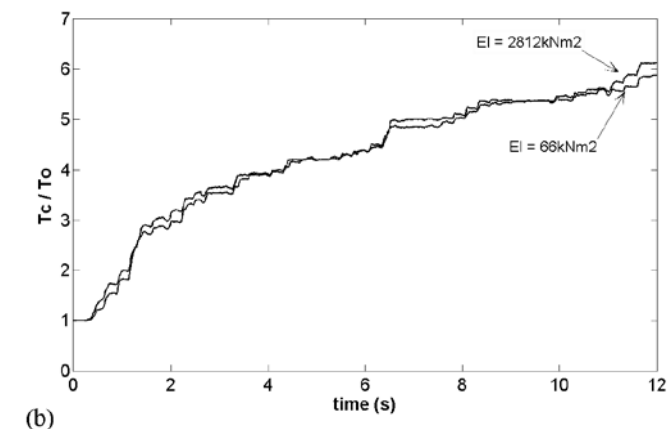
Fig. 10 Influence of facing panel stiffness (hinged toe): (a) connection load histories at the bottom reinforcement layer; (b) connection load normalized by the load at the end of construction ( T_o )
