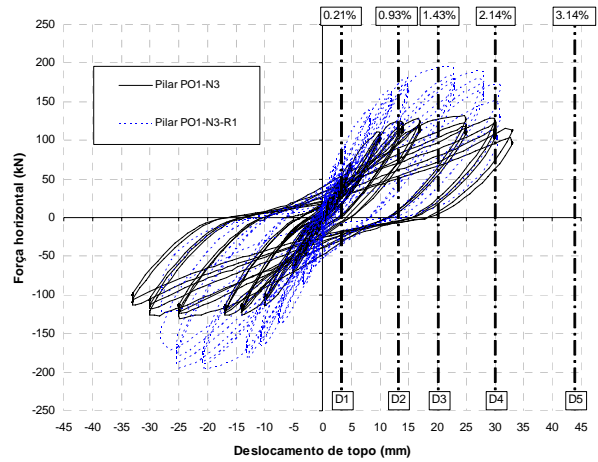
c) Comparison before and after retrofit
