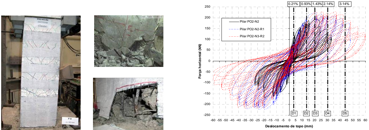
a) Final damage - west b) Final damage – inside / base c) Comparison before and after retrofit Figure 12 Experimental results of pier PO2-N3-R2.
