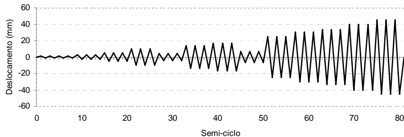
Figure 3 Top-displacements during the tests
