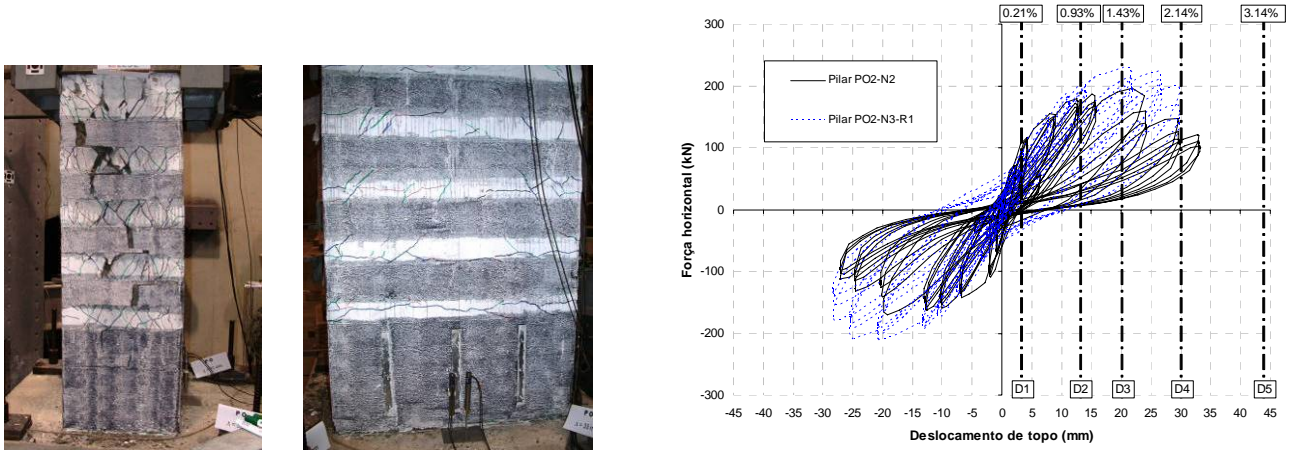
a) Final damage - west b) Final damage – south c) Comparison before and after retrofit Figure 11 Experimental results of pier PO2-N3-R1.
