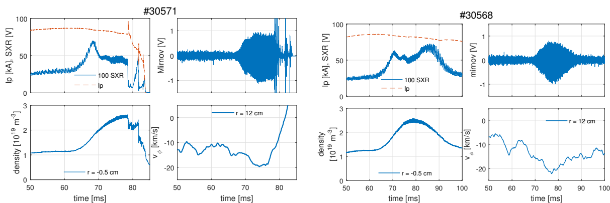
Figure 2: Plasma current, soft X-rays (SXR), line-averaged electron density, Mirnov signal and toroidal velocity for discharges with (#30571) and without disruption (#30568)
