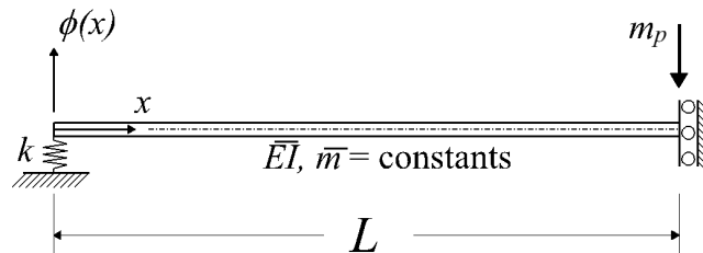
Figure 3. Scheme of the simply supported beam
