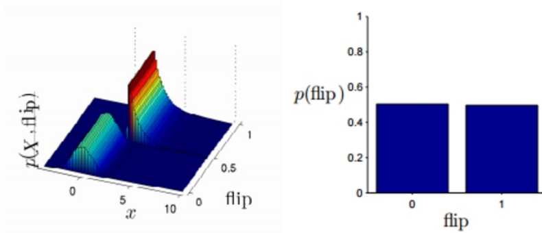
Figure 2.3: Implied distributions over variables [DL13]
