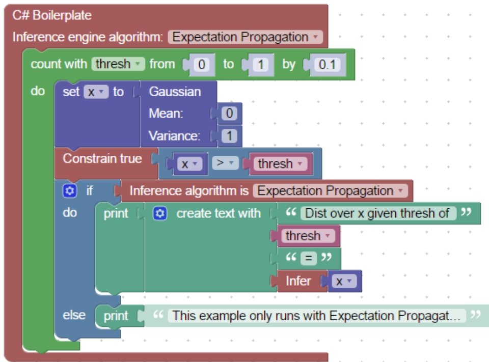
Figure 5.2: Truncated Gaussian PP
