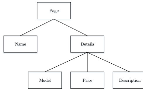
Figure 2.8: Sample EC tree of a generic product HTML page [Liu11].
