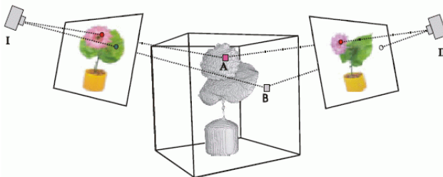
Figure 2. Color consistency ([14]): both projections of voxel A have the same color, so it is consistent; projections of voxel B have different colors, so it is inconsistent and, consequently, should not belong to the object's surface.
