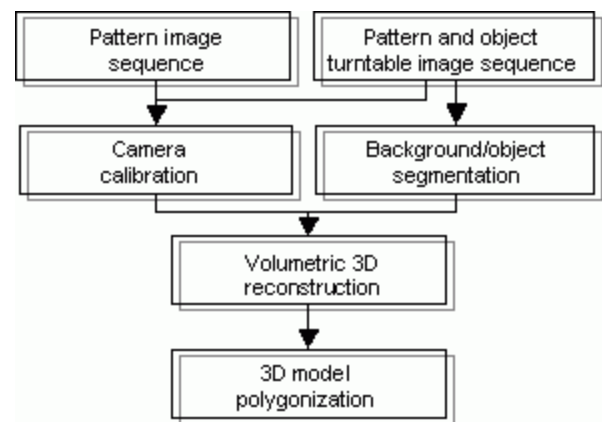
Figure 3. Methodology followed to obtain the 3D reconstruction of objects from uncalibrated images.
