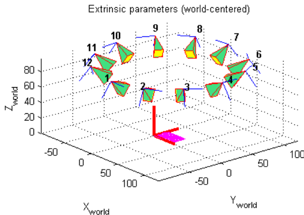
Figure 7. Extrinsic parameters representation for the image sequence of the torso case.
