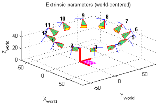
Figure 7. Extrinsic parameters representation for the image sequence of the hand case.
