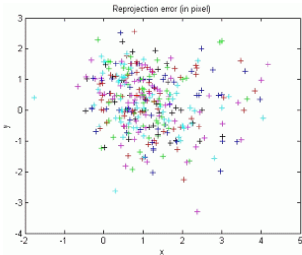
Figure 9. Reprojection errors for the image sequence of the hand case.
