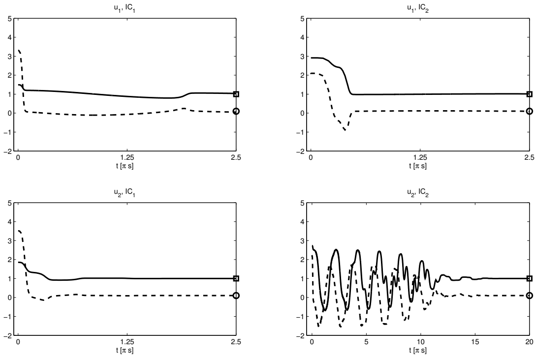
Fig. 2. Time-evolution of the estimated parameterization produced by the HNN for two different sets of initial conditions IC and two different forces u , where IC_1 = \{x_i(0) = 0 \text{ [m]}, \dot{x}_i(0) = 0 \text{ [\frac{m}{s}]} \} , IC_2 = \{x_i(0) = 0 \text{ [m]}, \dot{x}_1(0) = 1, \dot{x}_2(0) = 2 \text{ [\frac{m}{s}]} \} , and u_1(t) = 1 + e^{-t} \text{ [N]} , u_2(t) = \cos(\pi t) \text{ [N]} . The solid and dashed lines represent respectively the estimated values for k and b ; the square and the circle represent respectively the actual values of k and b . Mind the different time interval used in the last simulation.
