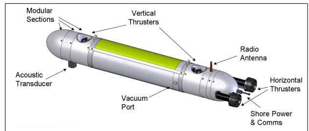
Fig. 2. MARES Solidworks® model.
