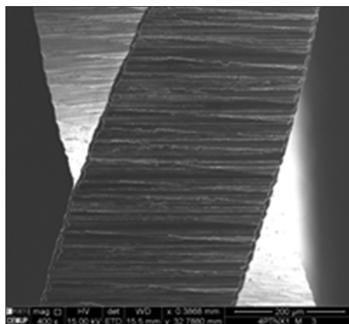
Figure 5: Middle view of 4 ProTaper next X1 files after usage.
