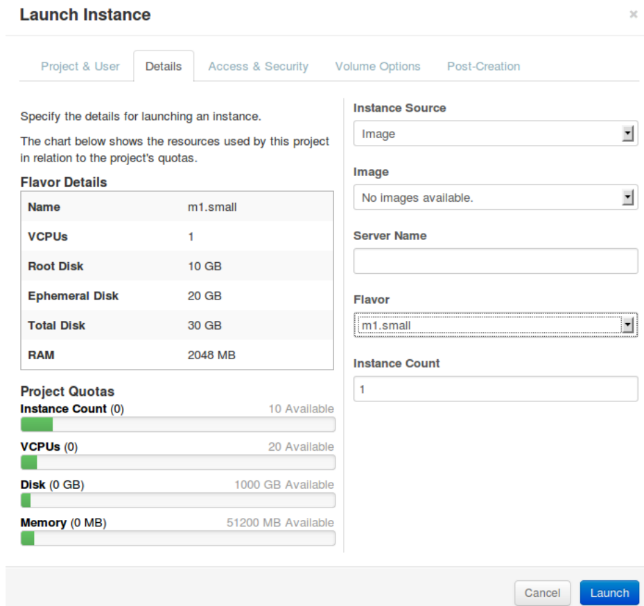
Figure 2.5: Launching an instance in Horizon .
