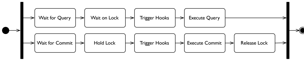
Figure 6.5: Activity diagram of the main loop.
