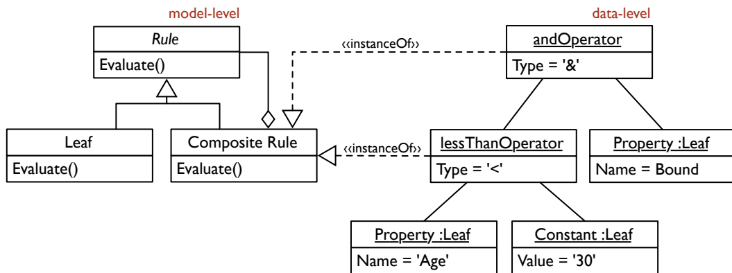
Figure 3.7: A class and objects diagram of the COMPOSITE pattern, forming the structure of the part-whole hierarchy of a AST for the expression Age < 30 ∧ Bound.
