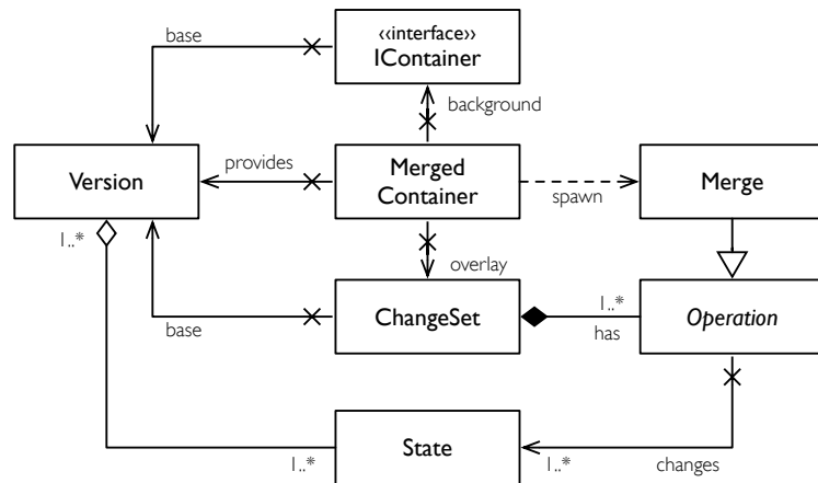
Figure 6.18: Merging mechanism used to validate and apply operations, which are stored in a Changeset.
