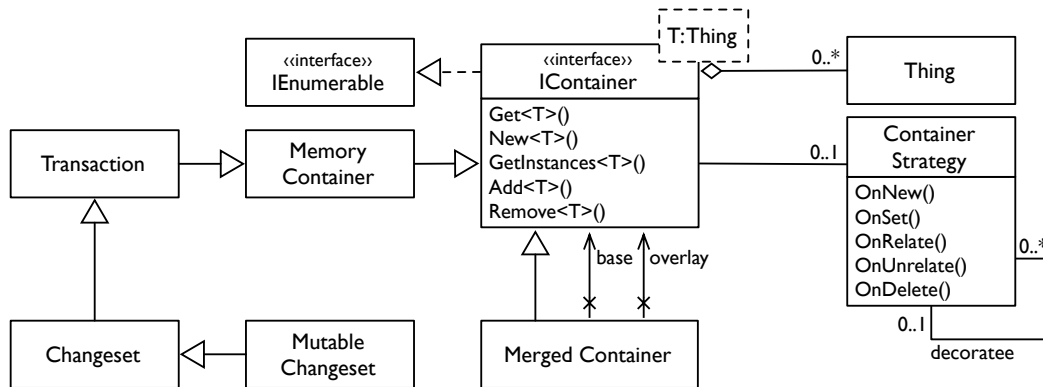
Figure 6.15: Class diagram of the warehousing design.
