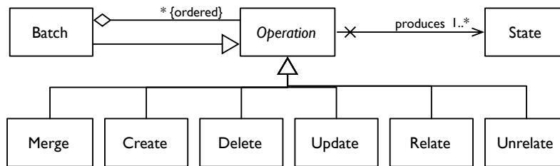
Figure 6.17: Data and meta-data are manipulated through operations, similarly to the COMMAND pattern. Each operations applies (or creates) Things to produce new States.
