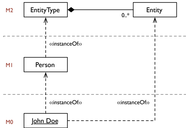
Figure 3.2: The meta layers of an AOM, when compared to MOF.
