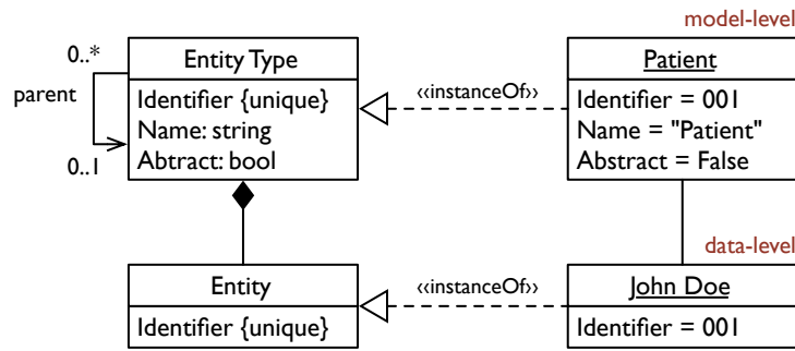
Figure 3.3: A class diagram of the TYPE-OBJECT pattern.
