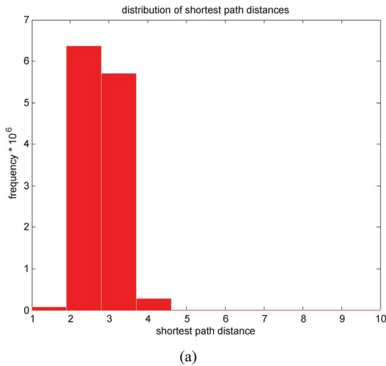
Figure 1. Structure of shortest paths in the yeast PPI network. (a) Distribution of shortest-path distances in the largest connected component of the yeast PPI network; (b) an example subgraph with a hub. doi:10.1371/journal.pone.0076339.g001
