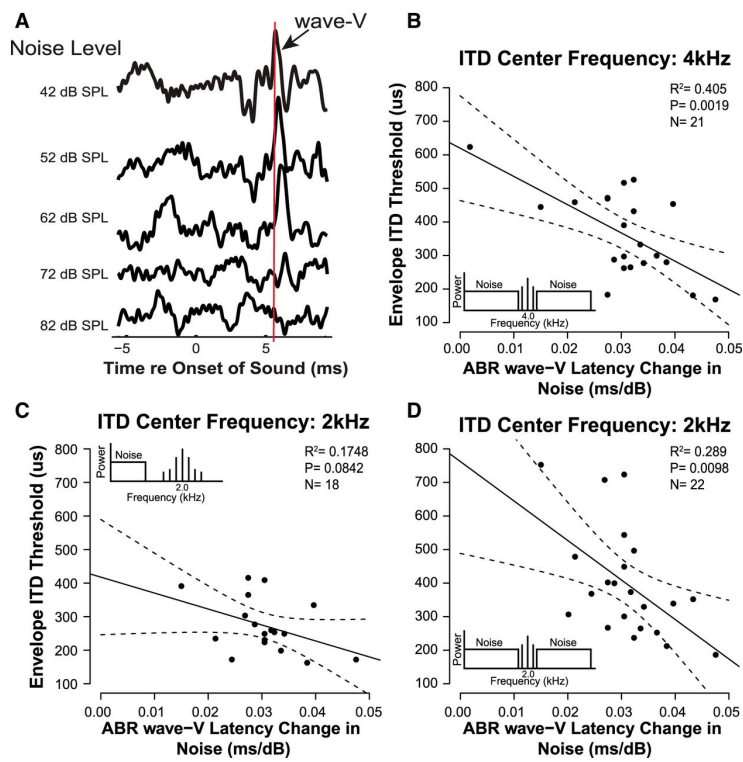
Figure 2-12: Latencies in increasing noise correlate with performance on ITD detection. Figure reprinted from Mehraei et al. (2016).
