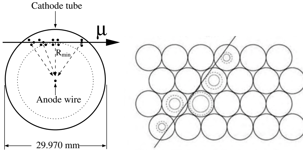
Figure 4.15: (Left) Cross-section of single MDT tube with muon track passing through. Ionized electrons (black dots) collect on the anode wire due to the applied electric field. (Right) Muon track reconstructed from array of MDT tubes.
