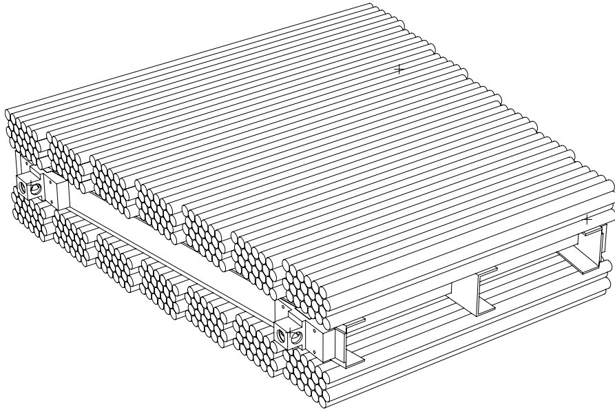
Figure 4.16: Schematic of a single MDT chamber.
