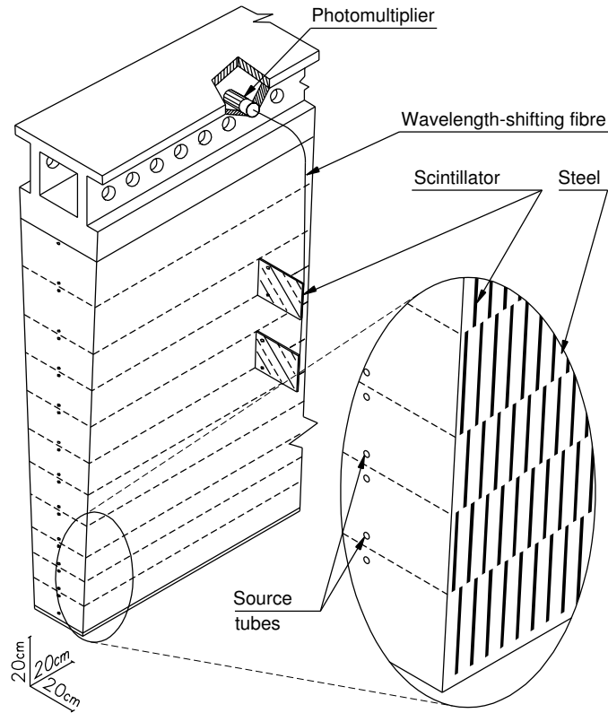
Figure 4.9: A diagram of one tile HCAL module covering 5.625^\circ in azimuth. The radial direction when positioned in the detector corresponds to the vertical direction in the image.
