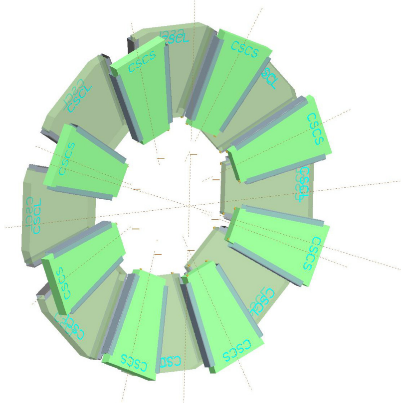
Figure 4.17: Diagram showing the arrangement of the CSCs in the end-cap.
