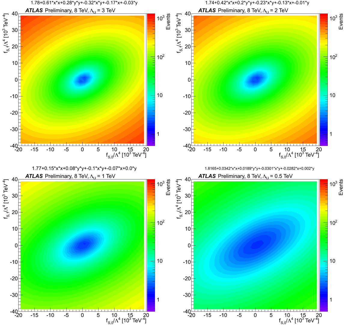
Figure 5.41: Unitarized aQGC signal yield prediction in the 0 SFOS region as a function of f_{S,0}/\Lambda^4 and f_{S,1}/\Lambda^4 using the functional form in Eq. (5.57). The predictions are shown with four different unitarization scales, \Lambda_U , at 3 TeV (Top Left), 2 TeV (Top Right), 1 TeV (Bottom Left), and 0.5 TeV (Bottom Right). The functional form is shown above the plot.
