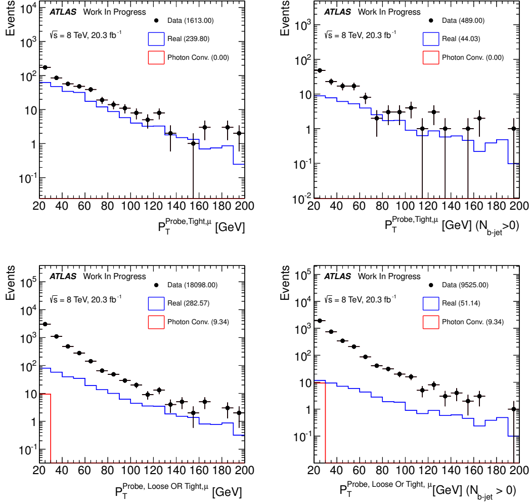
Figure 5.15: Transverse momentum distributions of tight probe muons (top) and loose OR tight probe muons (bottom) passing signal selection criteria in the same-sign \mu - \mu control region without any additional requirement on b -jets in the event (left) and at least one b -jet (right). The amount observed in data (black points) corresponds to N_T^{\text{Data},i} + N_L^{\text{Data},i} (bottom) and N_T^{\text{Data},i} (top) following the notation in Eq. 5.43. Meanwhile, the contribution determined in MC to come from real leptons (blue line) and from photon conversion (red line) are shown separately; they are not stacked. The real lepton contribution corresponds to N_T^{\text{Real},i} + N_L^{\text{Real},i} (bottom) and N_T^{\text{Real},i} (top) and the photon conversion contribution corresponds to N_T^{\text{PC},i} + N_L^{\text{PC},i} (bottom) and N_T^{\text{PC},i} (top) again using the notation in Eq. 5.42. The photon conversion is observed to be negligible for muons.
