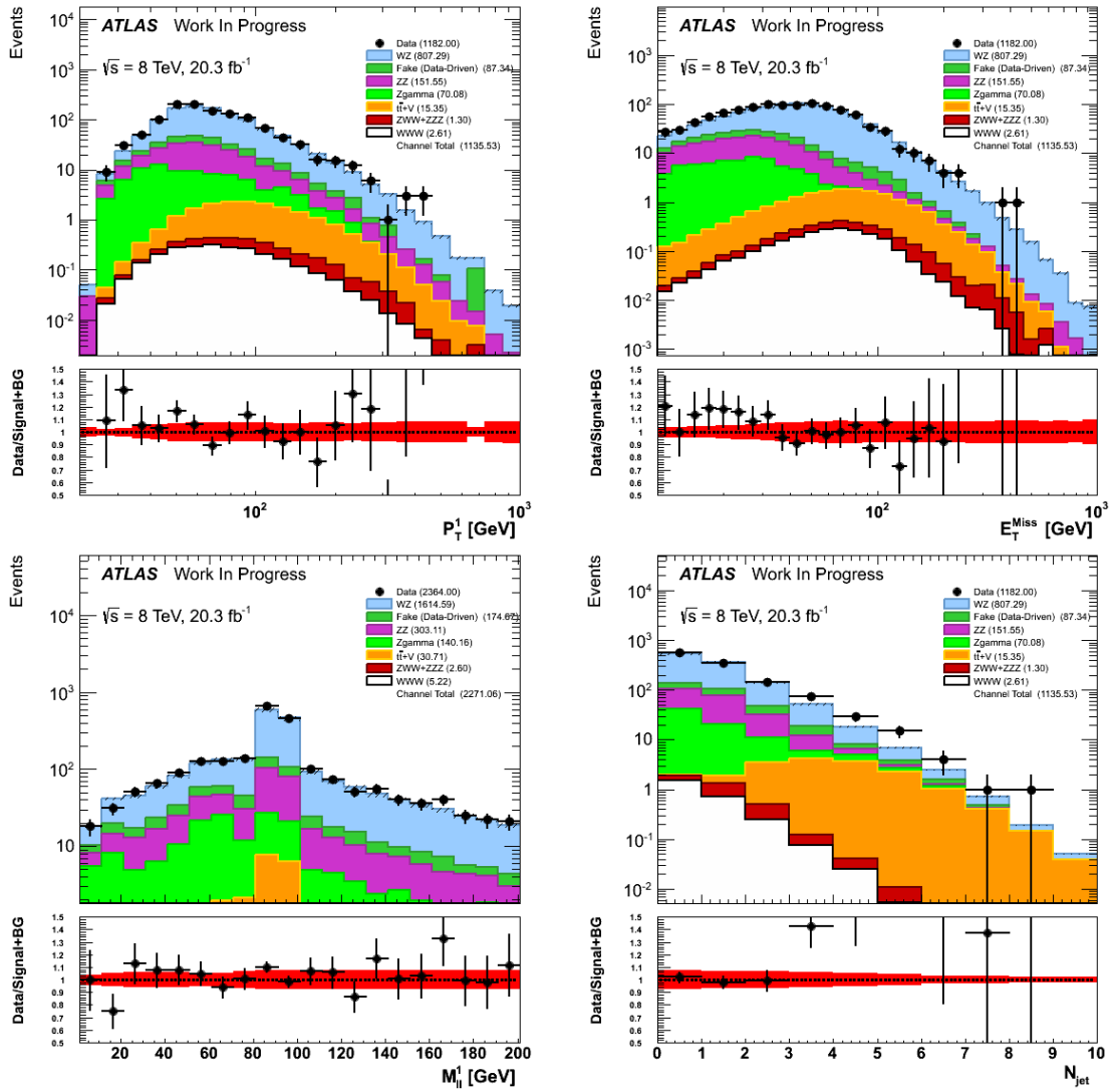
Figure 5.5: WZ control region with 3 lepton pre-selection plus 2 SFOS requirement. Distributions show leading lepton p_T , E_T^{\text{miss}} , leading di-lepton mass ( m_{ll} ), and the jet multiplicity ( N_{\text{jet}} ). The systematic band shows the uncertainty on the WZ k-factor.
