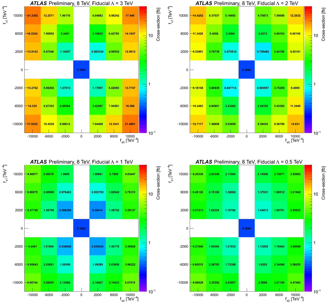
Figure 5.38: Fiducial cross-sections for unitarized aQGC signal samples as a function of f_{S,0}/\Lambda^4 vs f_{S,1}/\Lambda^4 . Four different unitarization scales, \Lambda_U , are shown: 3 TeV (Top Left), 2 TeV (Top Right), 1 TeV (Bottom Left), and 0.5 TeV (Bottom Right). The fiducial SM cross-section is shown at f_{S,0}/\Lambda^4 = f_{S,1}/\Lambda^4 = 0 for comparison. Regions that are white have not been evaluated.
