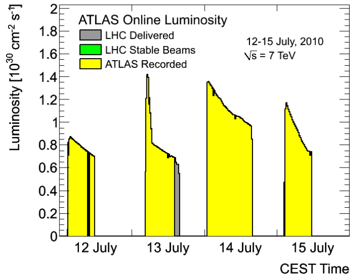
Figure 3.1: Instantaneous luminosity as a function of time as recorded by ATLAS for several runs in 2010.
