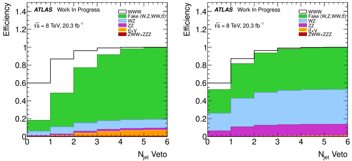
Figure 5.23: Signal and background efficiencies for the selection, N_{\text{Jet}} \leq X , as a function of the N_{\text{Jet}} selection threshold, X , in both the 0 SFOS (left) and pre-selection (right) regions.
