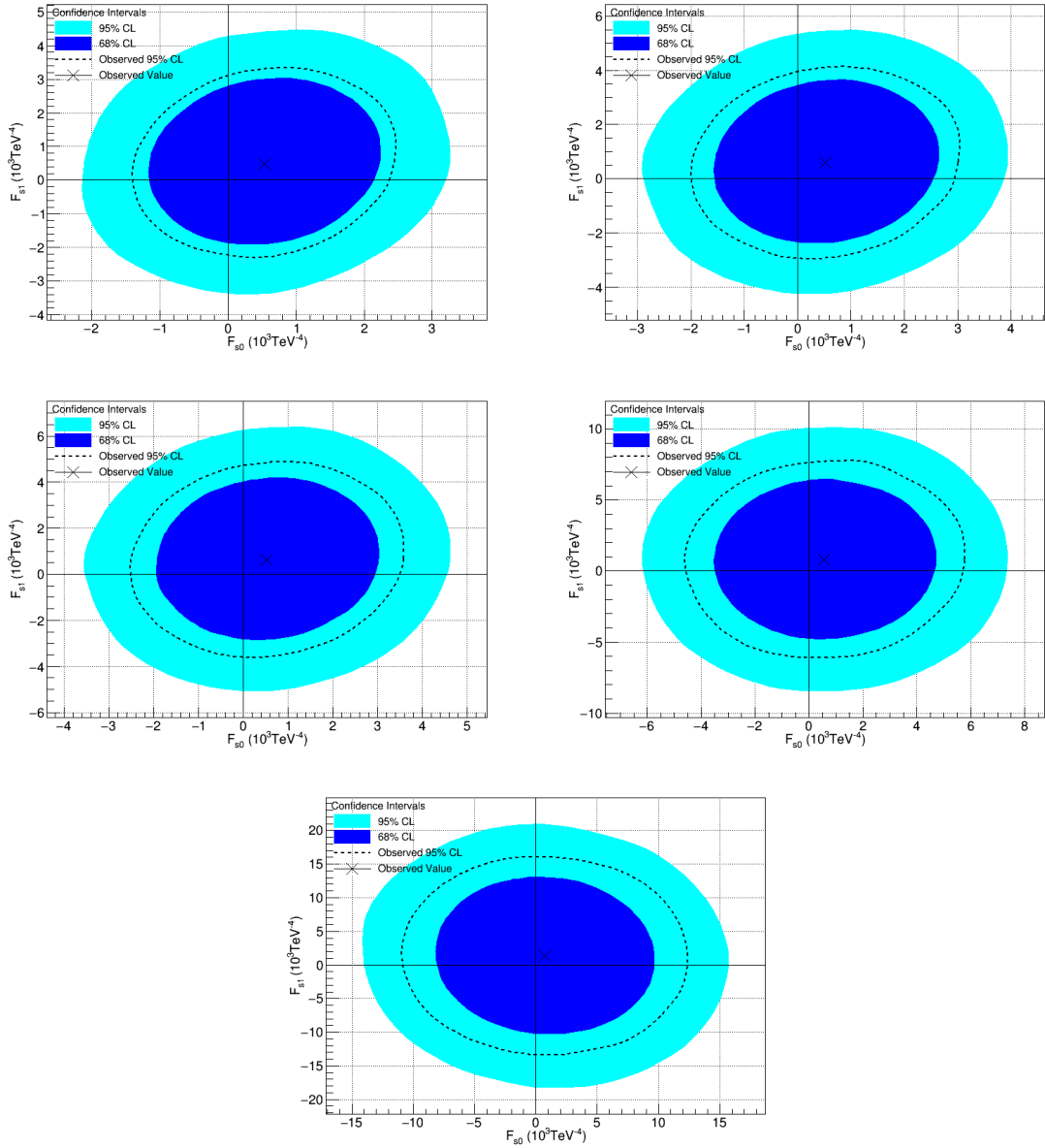
Figure 5.42: Two-dimensional limits as a function of f_{S,0}/\Lambda^4 vs f_{S,1}/\Lambda^4 at 95% CL for the non-unitarized case (Top Left) and three different choices of the unitarization scale, \Lambda_U : 3 TeV (Top Right), 2 TeV (Middle Left), 1 TeV (Middle Right), and 0.5 TeV (Bottom Center).
