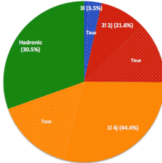
Figure 2.9: Pie chart showing the different decay modes contributing to the total cross-section for the WWW process. The dotted areas indicate the portion of each decay mode which is due to the production of tau leptons.
