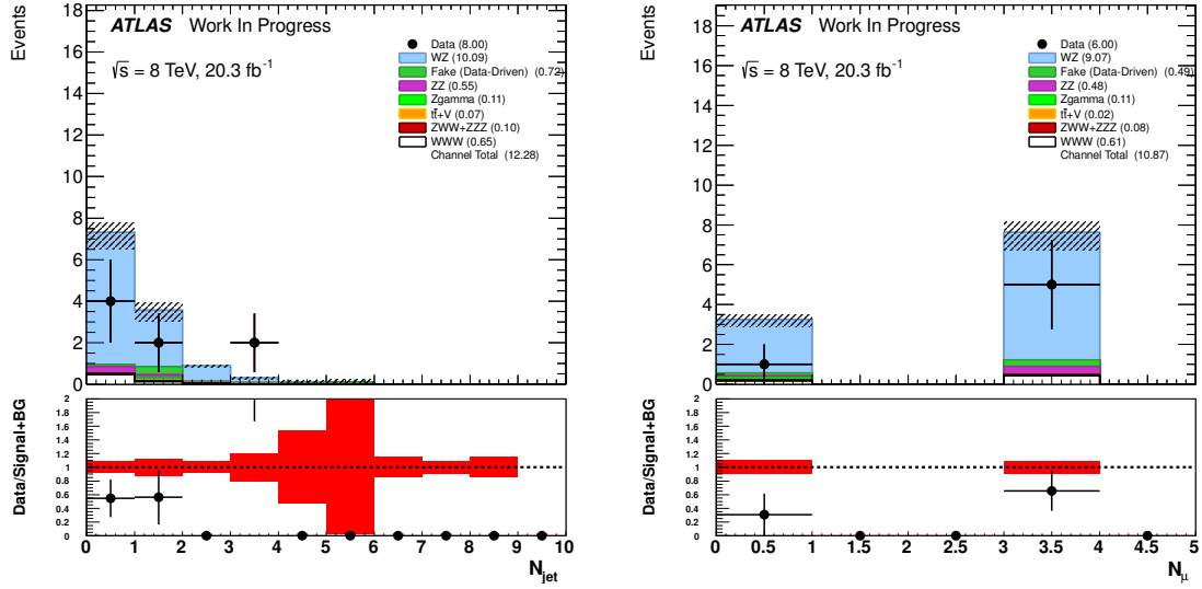
Figure 5.33: Distributions showing data compared to the signal plus background estimate in the 2 SFOS region at each stage of the selection before the cuts are applied to the given distribution. Referring to Table 5.22, the left plot is shown before cut number 6 is applied. The right plot is shown after all cuts have been applied.
