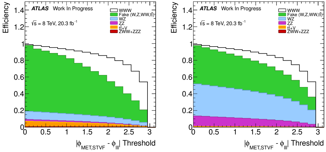
Figure 5.25: Signal and background efficiencies for the selection, |\Delta\varphi(lll, E_T^{\text{Miss}})| > X , as a function of the \Delta\varphi(lll, E_T^{\text{Miss}}) selection threshold, X , in both the 0 SFOS (left) and pre-selection (right) regions.
