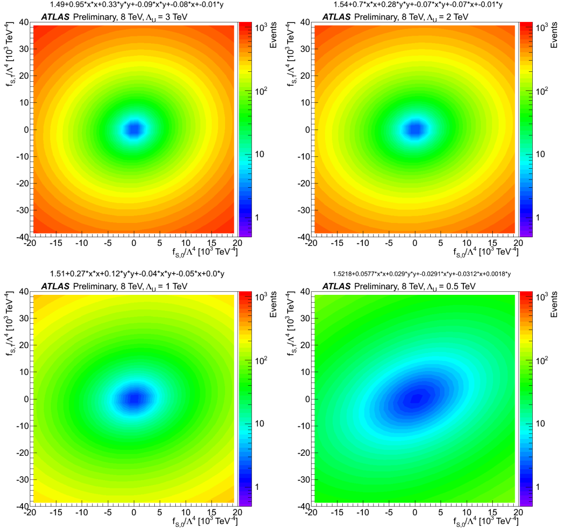
Figure 6.3: Unitarized aQGC signal yield prediction in the \mu\mu semi-leptonic signal region as a function of f_{S,0}/\Lambda^4 and f_{S,1}/\Lambda^4 using the functional form in Eq. (5.57). The predictions are shown with four different unitarization scales, \Lambda_U , at 3 TeV (Top Left), 2 TeV (Top Right), 1 TeV (Bottom Left), and 0.5 TeV (Bottom Right). The functional form is shown above the plot.
