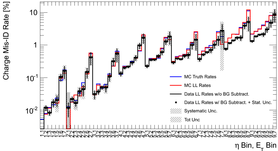
Figure 5.9: Summary of electron charge mis-identification rates using the likelihood method in data with background subtraction (black points) and without background subtraction (black line), the MC truth method (blue line), and the likelihood method in MC (red). Systematic uncertainties are extracted as described in the text and are shown in the gray hashed band pointing from bottom left to top right. The systematic uncertainties are combined with the statistical uncertainties on the black points to arrive at a total uncertainty on the rates, shown in the hashed band pointing from bottom right to top left.
