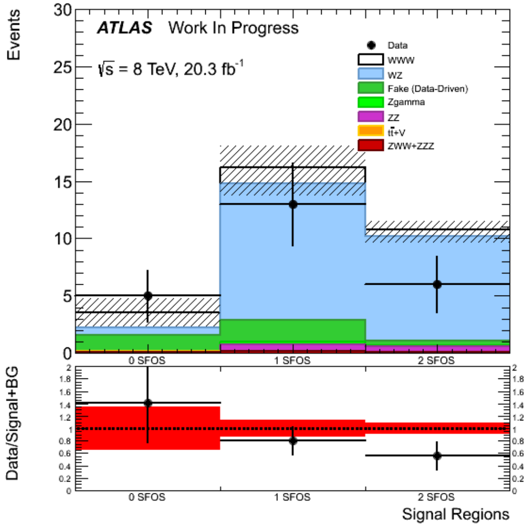
Figure 5.27: Yields after full selection in the 0, 1 and 2 SFOS regions. The most important systematic uncertainties are shown, namely from the fake estimates and the uncertainties on the WZ and ZZ k-factors.
