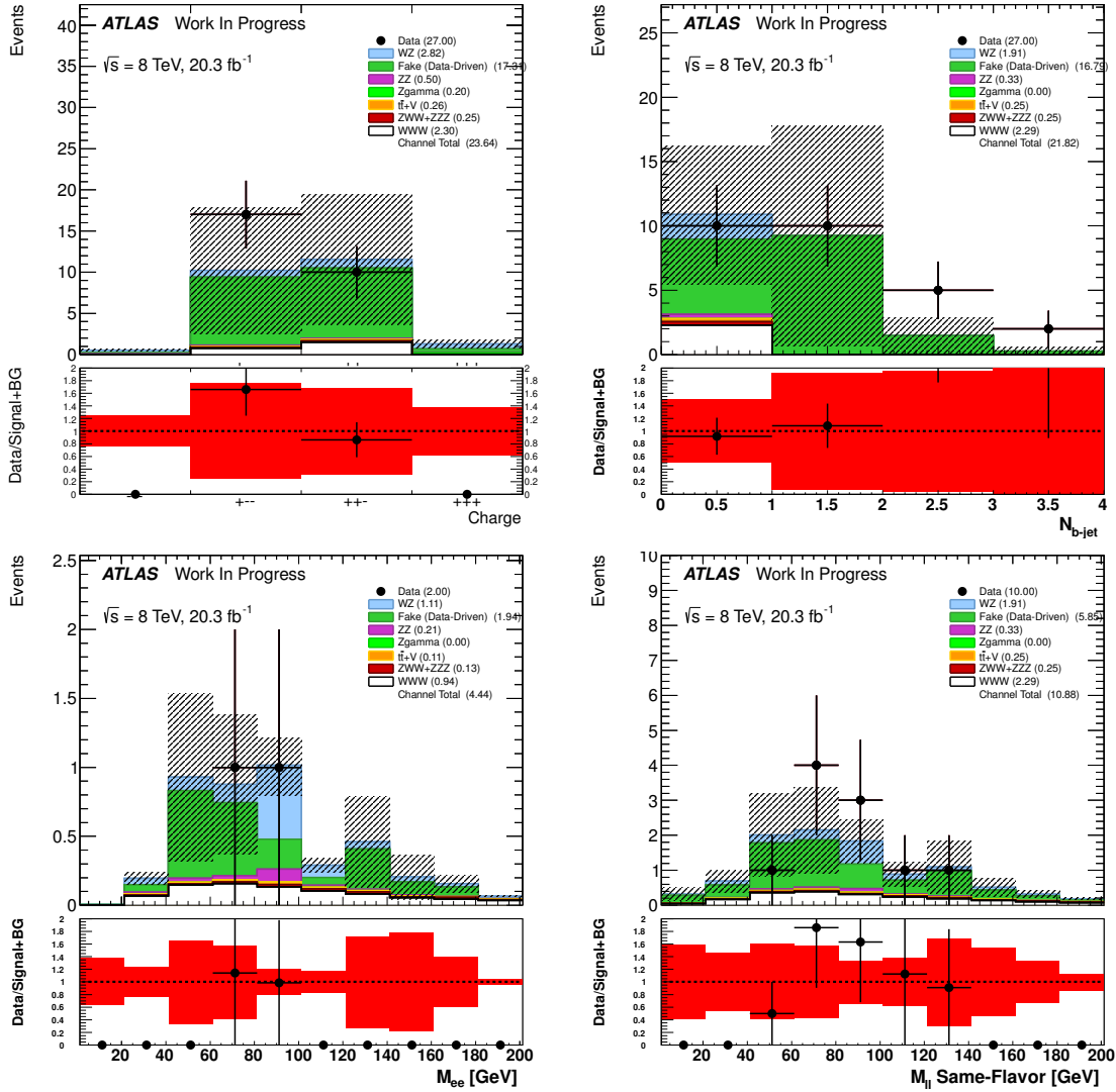
Figure 5.28: Distributions showing data compared to the signal plus background estimate in the 0 SFOS region at each stage of the selection before the cuts are applied to the given distribution. Plots should be read clockwise starting from the top left. Referring to Table 5.18, the top left plot is shown before cut number 2 is applied, followed by cuts number 3, 4, and 5.
