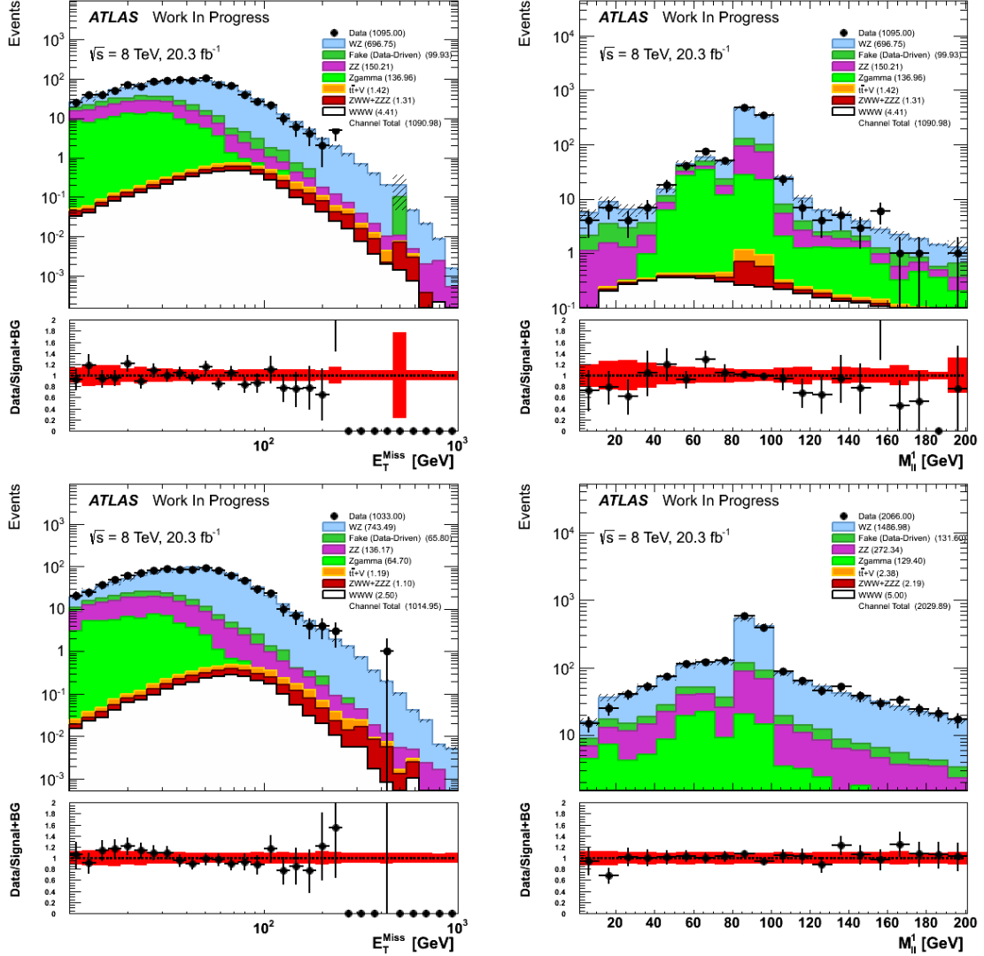
Figure 5.21: Plots of the E_T^{\text{miss}} (left) and m_{\text{SFOS}} (right) distributions in the 1 SFOS (top) and 2 SFOS (bottom) regions after pre-selection plus the b -veto requirement.
