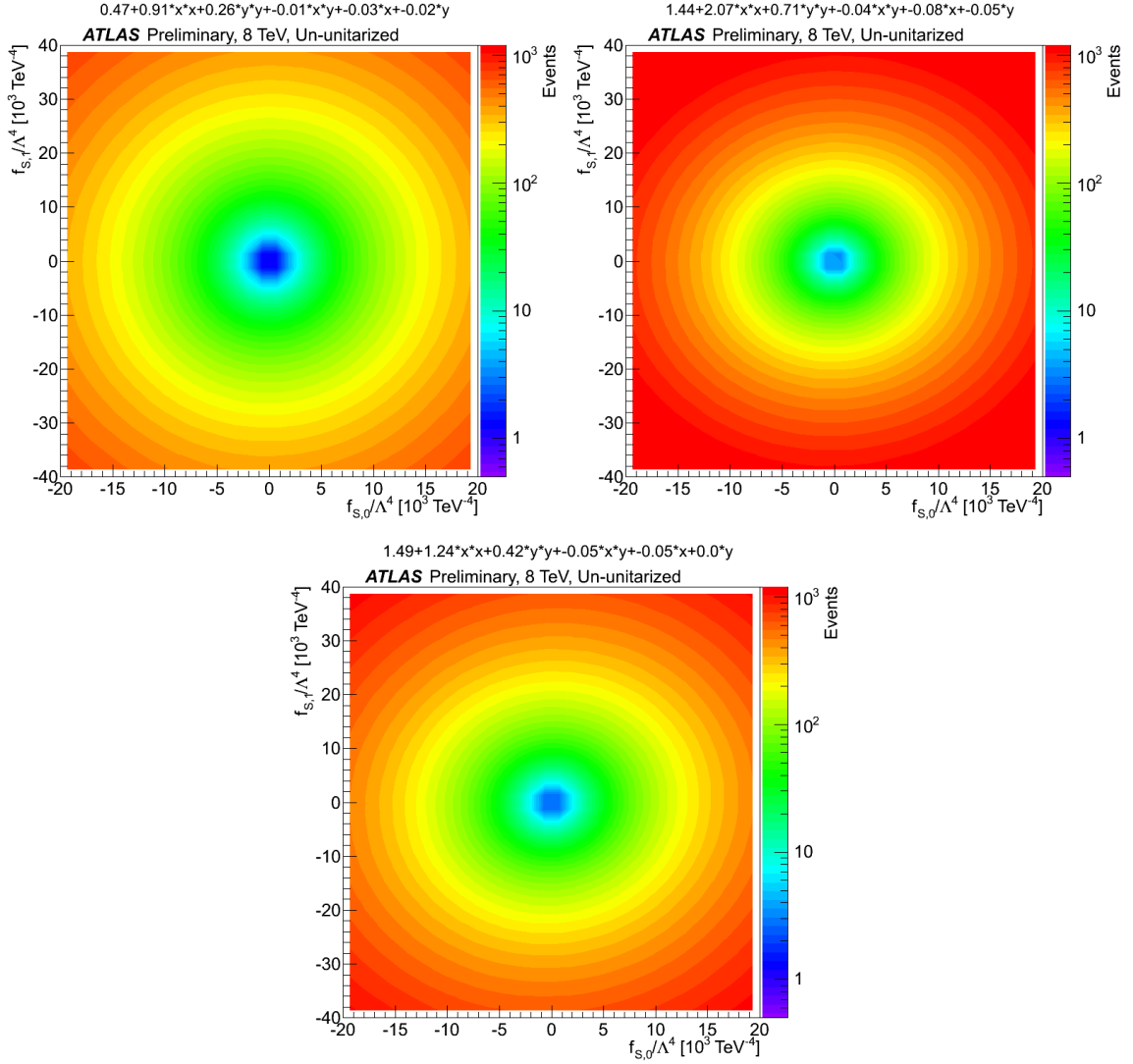
Figure 6.2: Non-unitarized aQGC signal yield predictions in the ee (Top Left), e\mu (Top Right), and \mu\mu (Bottom Middle) semi-leptonic signal regions as a function of f_{S,0}/\Lambda^4 and f_{S,1}/\Lambda^4 using the functional form in Eq. (5.57). The functional form is shown above the plot.
