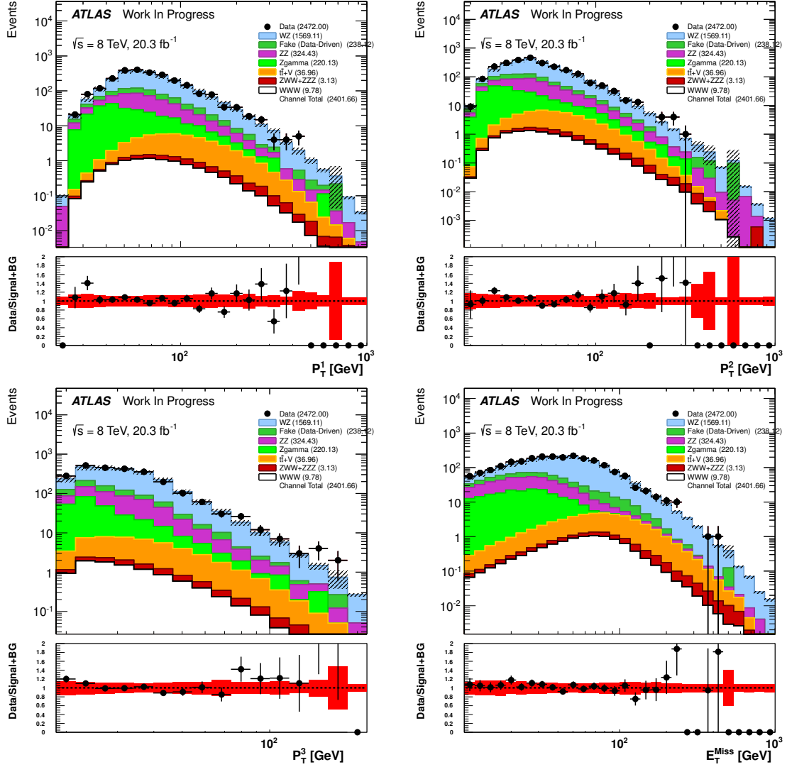
Figure 5.18: Distributions showing the observed data compared to the background estimate at event pre-selection. From top to bottom and left to right, these distributions are: the leading, sub-leading, and minimum lepton p_T (ordered by their p_T ), E_T^{\text{miss}} .
