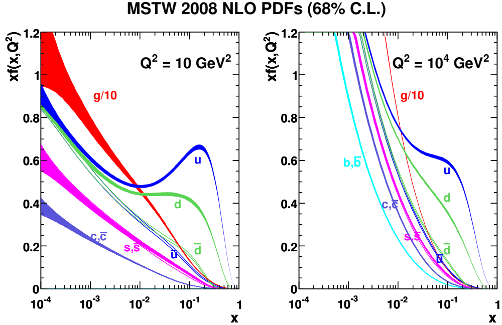
Figure 2.2: Plot of xf_i(x, Q^2) vs x for the MSTW 2008 NLO PDF sets [2] with 68% CL eigenvector uncertainties for two different scales, Q^2 = \mu_R^2 = \mu_F^2 . The peaks in the f_u and f_d distributions are due to the valence quark requirements in the proton. The sea quark PDF distributions are shown, as is the large gluon PDF, which is scaled down by a factor of 10. At high Q^2 , the sea quark PDFs become more important, as do the contribution from heavy quarks.
