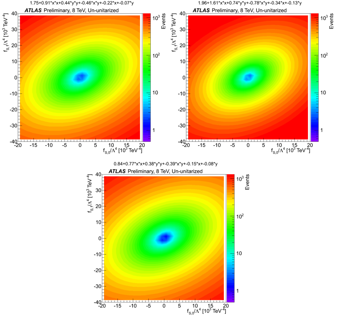
Figure 5.40: Non-unitarized aQGC signal yield predictions in the 0 SFOS (Top Left), 1 SFOS (Top Right), and 2 SFOS (Bottom Middle) fully-leptonic signal regions as a function of f_{S,0}/\Lambda^4 and f_{S,1}/\Lambda^4 using the functional form in Eq. (5.57). The functional form is shown above the plot.
