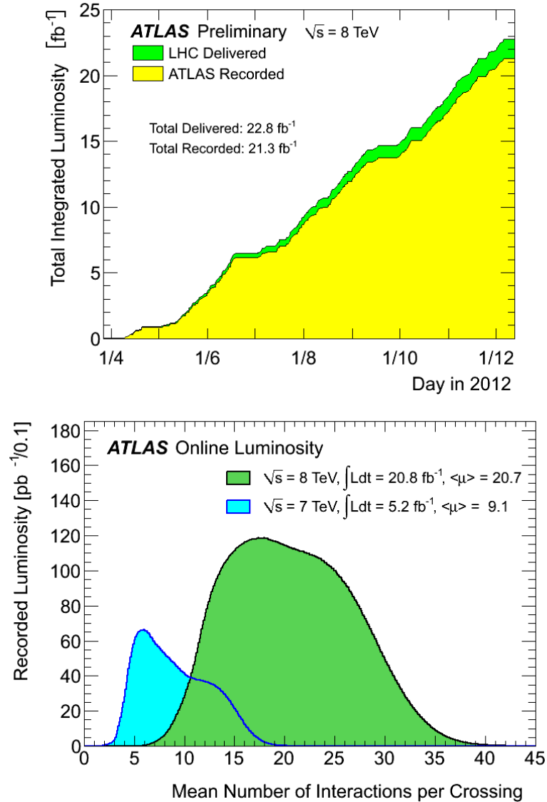
Figure 3.5: (Top) The integrated luminosity as a function of time in 2012. The amount delivered by the LHC is shown in green while the amount recorded by ATLAS is overlaid in yellow. More than 93 % of the integrated luminosity delivered by the LHC in 2012 was recorded by ATLAS. (Bottom) The distribution of pileup interactions, parameterized as the mean number of interactions per crossing, \langle \mu \rangle , recorded by ATLAS in 2011 and 2012.
