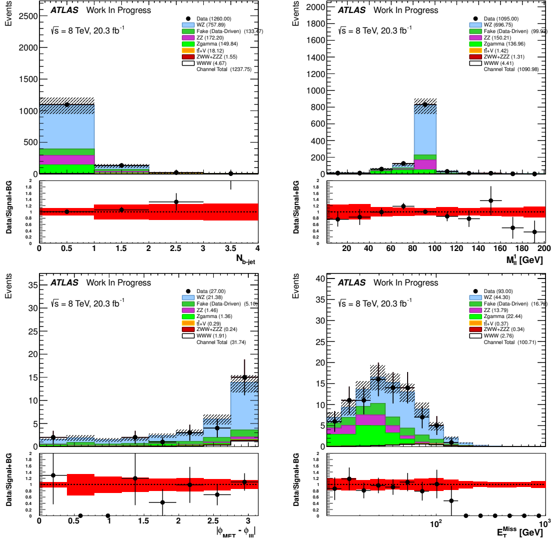
Figure 5.30: Distributions showing data compared to the signal plus background estimate in the 1 SFOS region at each stage of the selection before the cuts are applied to the given distribution. Plots should be read clockwise starting from the top left. Referring to Table 5.20, the top left plot is shown before cut number 2 is applied, followed by cuts number 3, 4, and 5.
