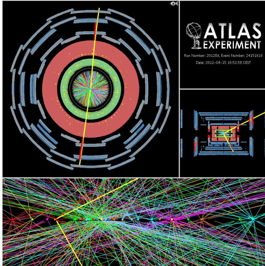
Figure 3.2: An event display of 20 pileup interactions in a single bunch crossing. The resulting tracks are shown, along with two high energy muons extrapolated back to a single primary vertex. The upper left shows a cross-section of the whole detector in the transverse plane, the upper right shows the detector viewed along the r - z plane, and the bottom portion is zoomed in to the length of the bunch crossing. The average bunch crossing length at the LHC is around 10 cm [1].
