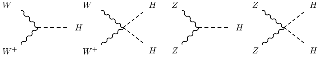
Figure 2.5: Feynman diagrams of the Higgs couplings with the W and Z gauge bosons.
