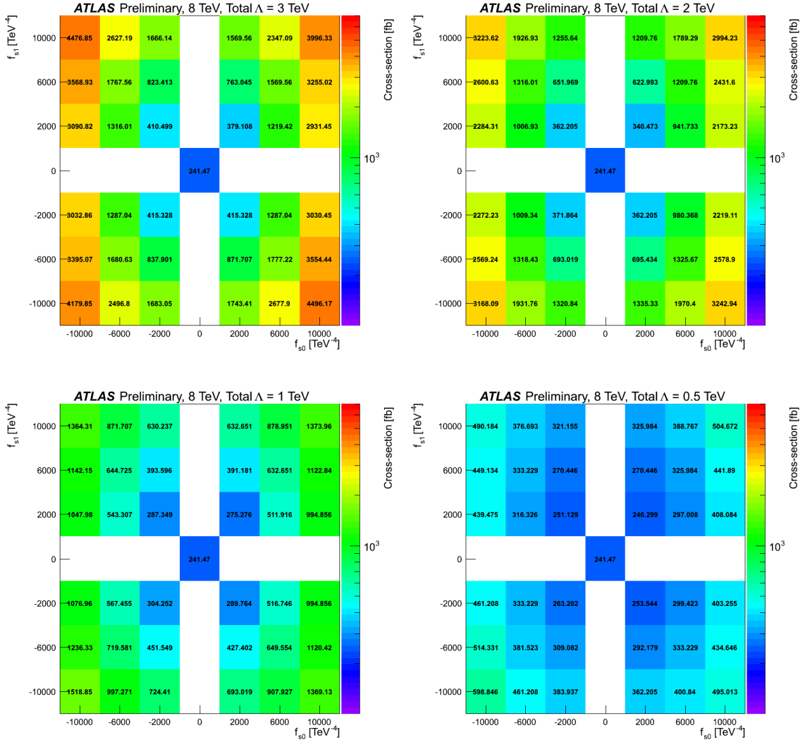
Figure 5.3: Total cross-section for unitarized aQGC signal samples as a function of f_{S,0}/\Lambda^4 vs f_{S,1}/\Lambda^4 . Four different values of the unitarization scale, \Lambda , are chosen: 3 TeV (Top Left), 2 TeV (Top Right), 1 TeV (Bottom Left), and 0.5 TeV (Bottom Right). The total SM cross-section is shown at f_{S,0}/\Lambda^4 = f_{S,1}/\Lambda^4 = 0 for comparison. Those points that are white have not been evaluated.
