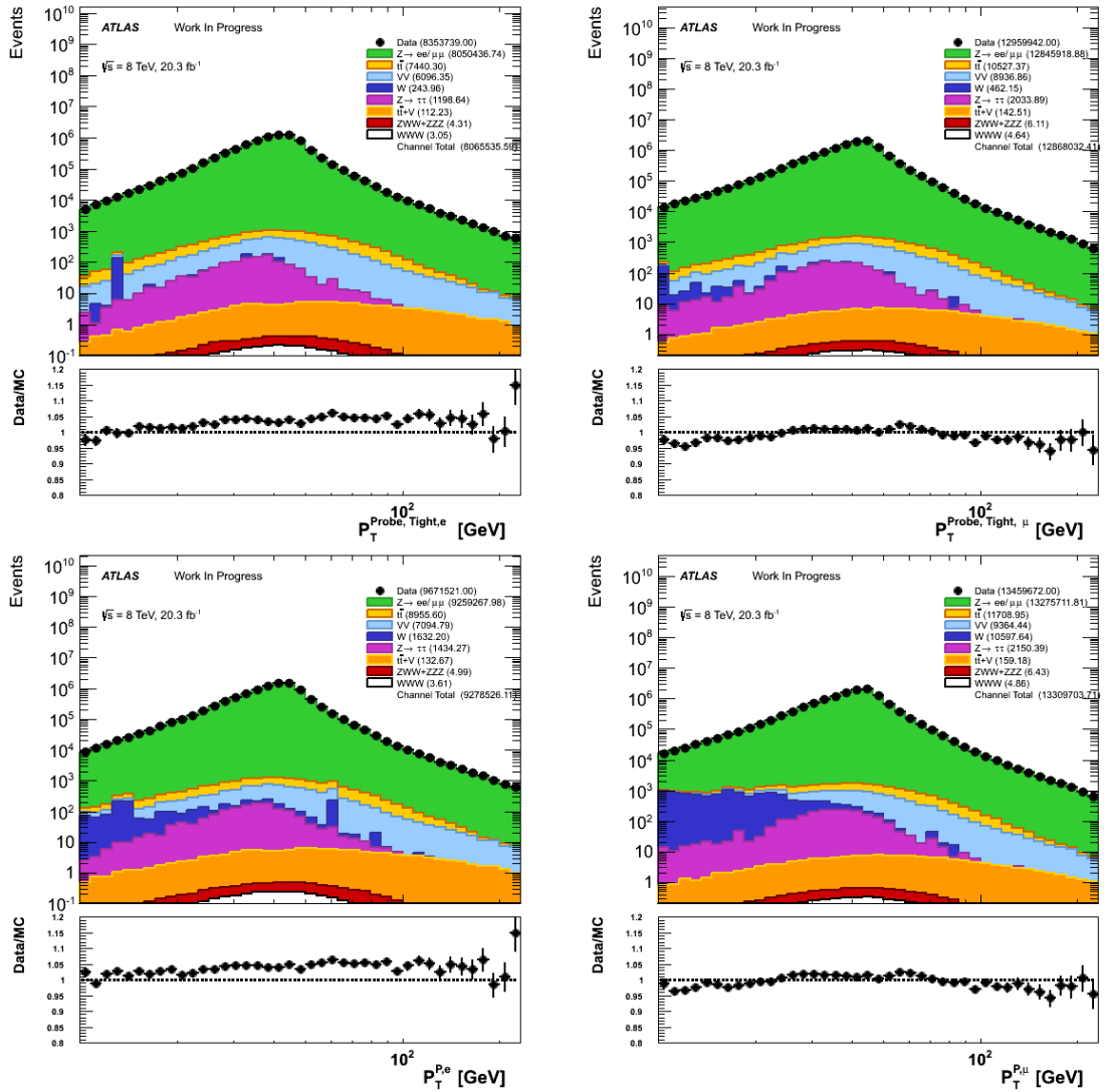
Figure 5.13: Probe lepton p_T distributions in SFOS tag and probe control regions used to derive the real rates. The electron (left) and muon (right) distributions are shown when the probe lepton is either tight (top) or tight plus loose (bottom).
