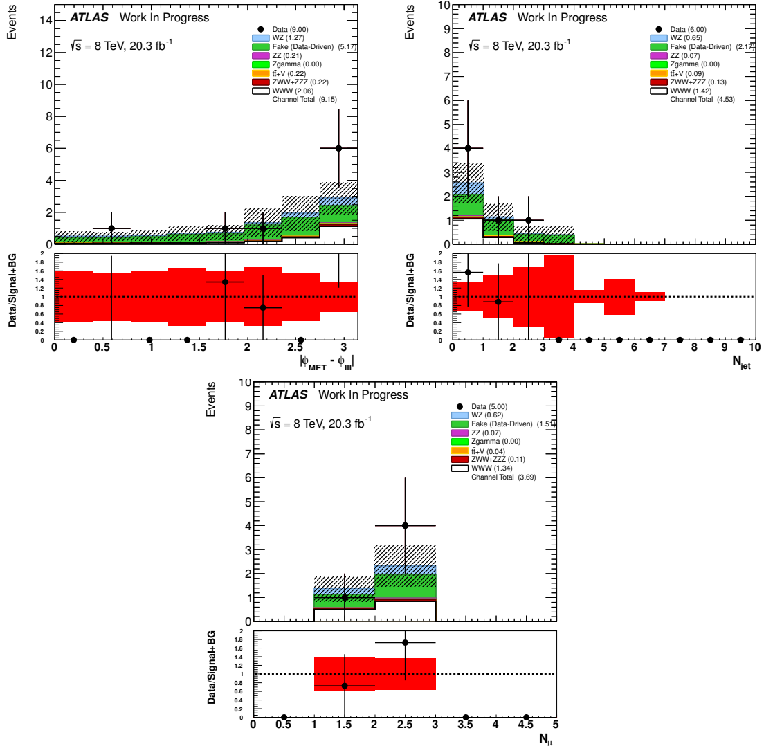
Figure 5.29: Distributions showing data compared to the signal plus background estimate in the 0 SFOS region at each stage of the selection before the cuts are applied to the given distribution. Plots should be read clockwise starting from the top left. Referring to Table 5.18, the top left plot is shown before cut number 5 is applied, followed by cut number 6. The bottom middle plot is shown after all cuts have been applied.
