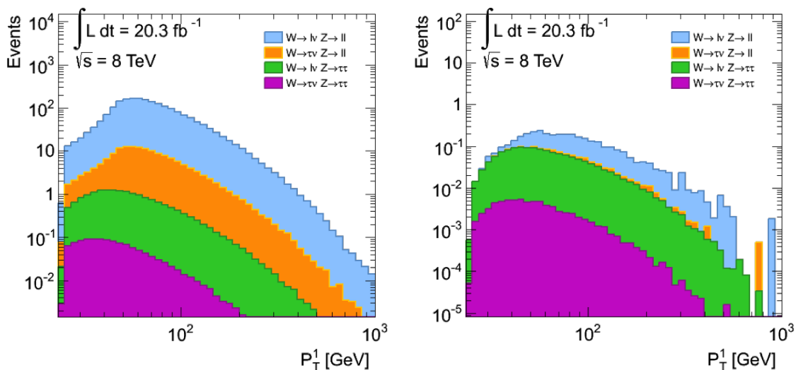
Figure 5.12: Plots of the different branching fractions of the WZ process as a function of the leading lepton p_T at pre-selection (left) and after also applying a requirement that events have 0 SFOS lepton pairs (right). The individual decays of W and Z are split up into whether they decay into taus ( \tau ) or into electrons and muons (denoted l ). The taus also subsequently decay. The contributions from WZ \rightarrow l\nu ll and WZ \rightarrow \tau\nu ll after applying the 0 SFOS selection are due purely to charge mis-identification.
