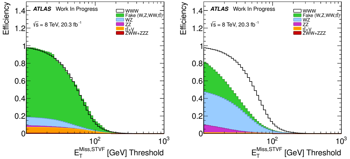
Figure 5.22: Signal and background efficiencies for the selection, E_T^{\text{miss}} > X , as a function of the E_T^{\text{miss}} selection threshold, X , in both the 0 SFOS (left) and pre-selection (right) regions.
