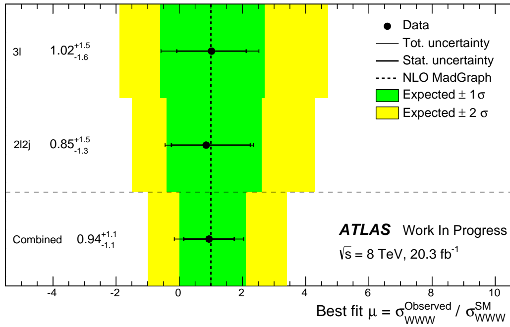
Figure 6.6: The expected and observed best fit signal strength, \mu , and uncertainties for the individual fully-leptonic and semi-leptonic measurements as well as for the combination of both channels.
