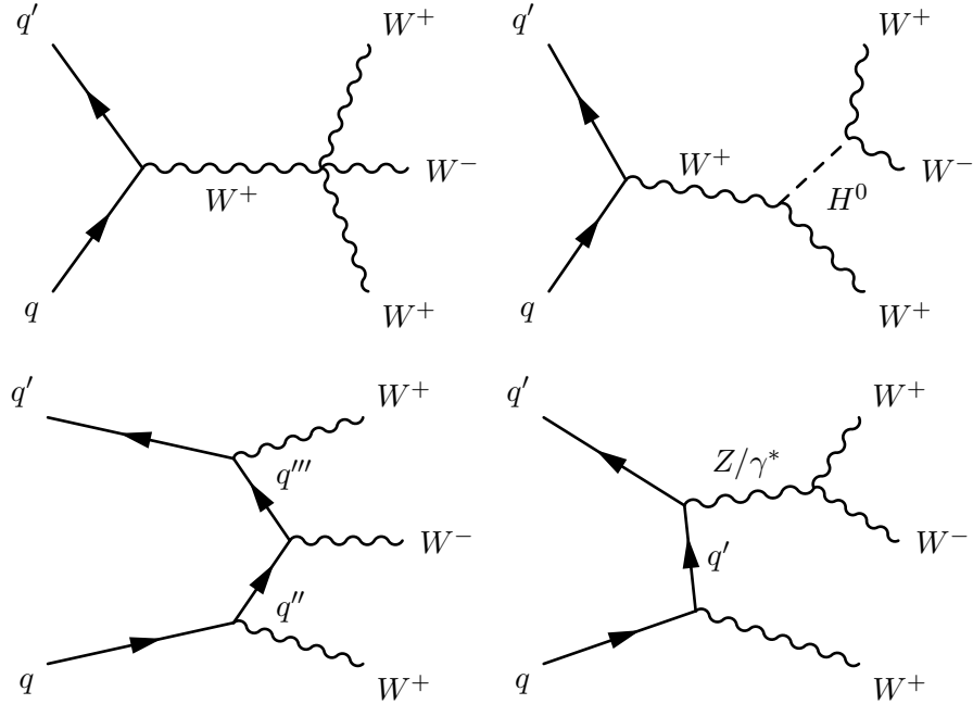
Figure 2.7: The tree level Feynman diagrams for WWW production. The incoming fermion lines in each diagram consist of an up-type quark (anti-quark) and down-type anti-quark (quark). In this case, the charge of the initial state quarks is assumed to sum to +1, leading to the same charge in the final state. It is also possible for the initial and final states to sum to -1 via charge conjugation.
