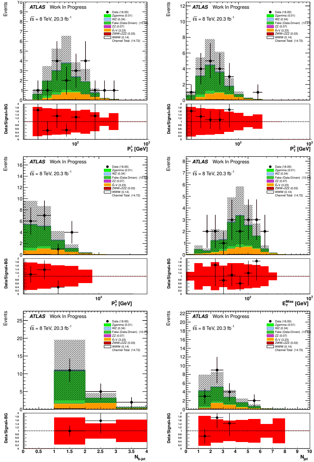
Figure 5.17: Distributions in a control region designed to study the data-driven fake lepton background estimate.
