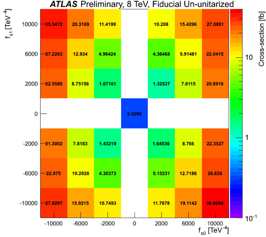
Figure 5.37: Fiducial cross-sections for the non-unitarized aQGC signal samples as a function of f_{S,0}/\Lambda^4 vs f_{S,1}/\Lambda^4 . The fiducial SM cross-section is shown at f_{S,0}/\Lambda^4 = f_{S,1}/\Lambda^4 = 0 for comparison. Regions that are white have not been evaluated.
