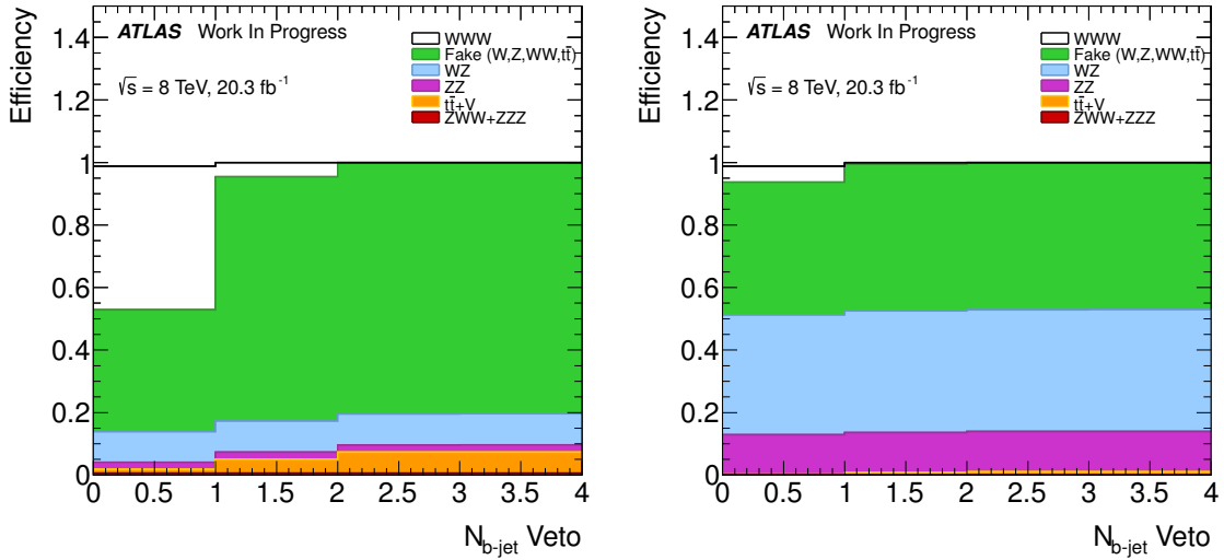
Figure 5.24: Signal and background efficiencies for the selection, N_{b-Jet} \leq X , as a function of the N_{b-Jet} selection threshold, X , in both the 0 SFOS (left) and pre-selection (right) regions.
