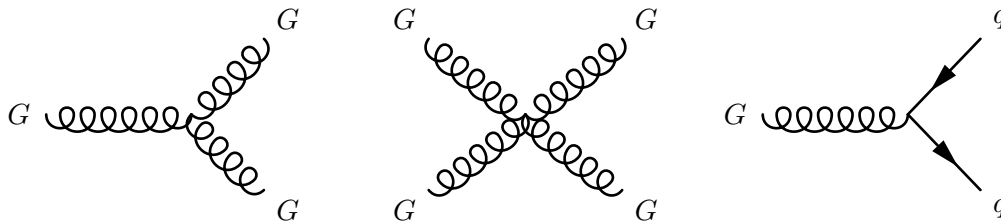
Figure 2.1: Feynman diagrams of QCD describing the interactions between gluon and quark fields. The gluons and quarks can in general have different colors.
