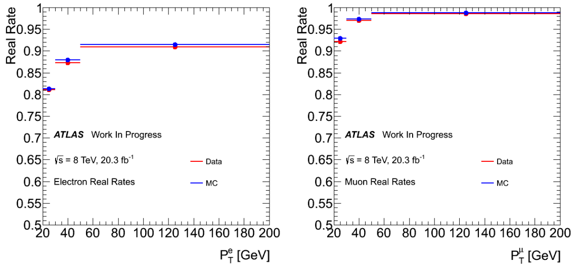
Figure 5.14: Real lepton rates as a function of p_T as measured in data (red) and MC (blue) for electrons (left) and muons (right).
