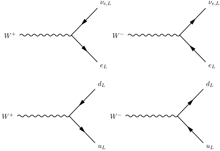
Figure 2.4: Feynman diagrams of the couplings of the W boson to the first generation of leptons (top) and quarks (bottom). The quark generations can mix while the lepton generations do not.
