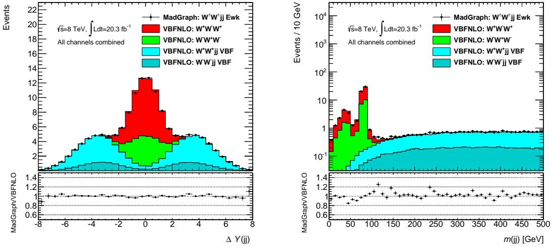
Figure 6.1: Comparison of the difference in the rapidity separation of the leading jets, |\Delta y_{jj}| , and the di-jet invariant mass, m_{jj} , between VBFNLO and MadGraph LO events with two same-sign leptons and two jets in the final state.
