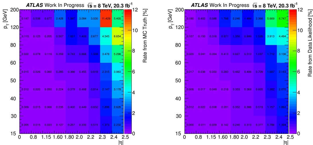
Figure 5.8: Electron charge mis-identification rates as a function of the electron p_T and \eta extracted using the MC truth method (left) and the likelihood method in data (right).
