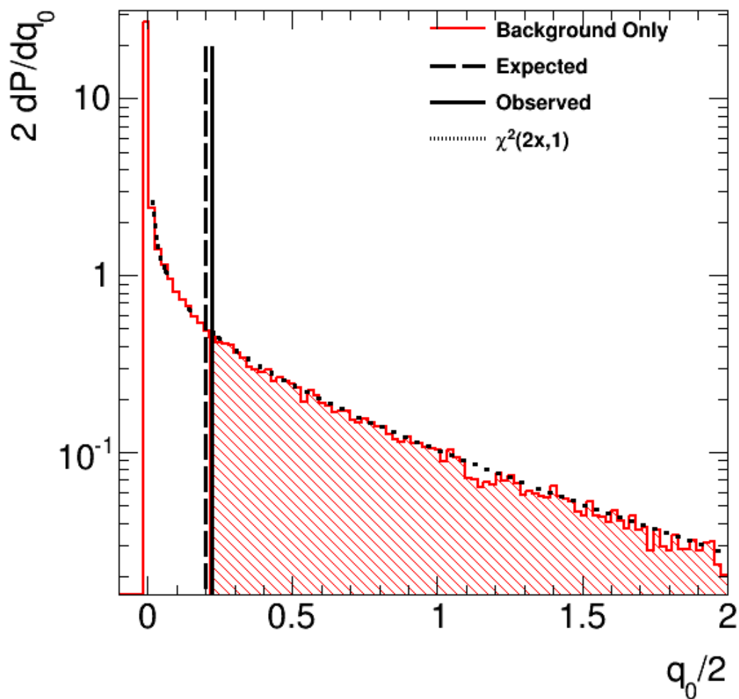
Figure 5.34: Probability distribution of the background-only hypothesis as a function of q_0 for the combination of all three channels. The probability distributions are determined using MC. The solid black line represents the observed value of q_0 seen in the data. The shaded area above this line represents the null p-value or the integral of the background hypothesis in the signal-like region. The dotted black curve shows a \chi^2 distribution for 1 degree of freedom with which it can be seen is a good approximation of the the background-only PDF.
