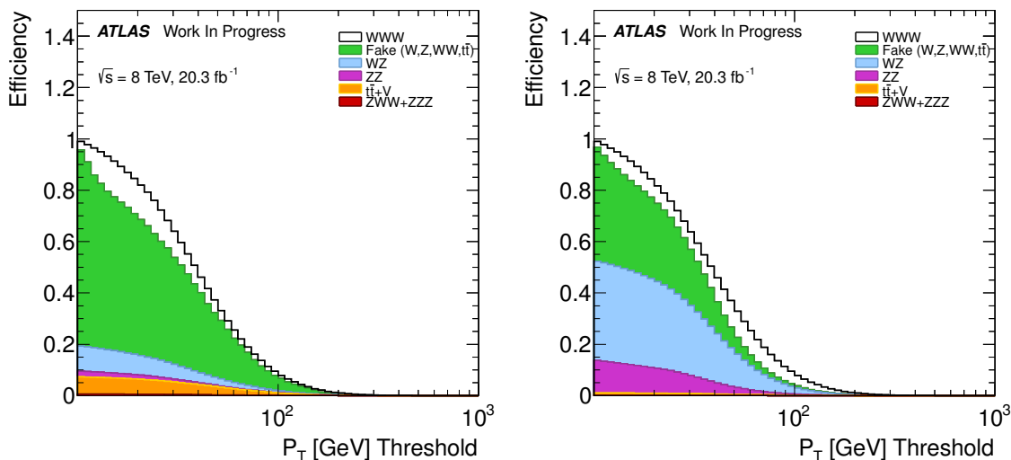
Figure 5.26: Signal and background efficiencies for the selection, Lepton p_T > X , as a function of the p_T selection threshold, X , in both the 0 SFOS (left) and pre-selection (right) regions.
