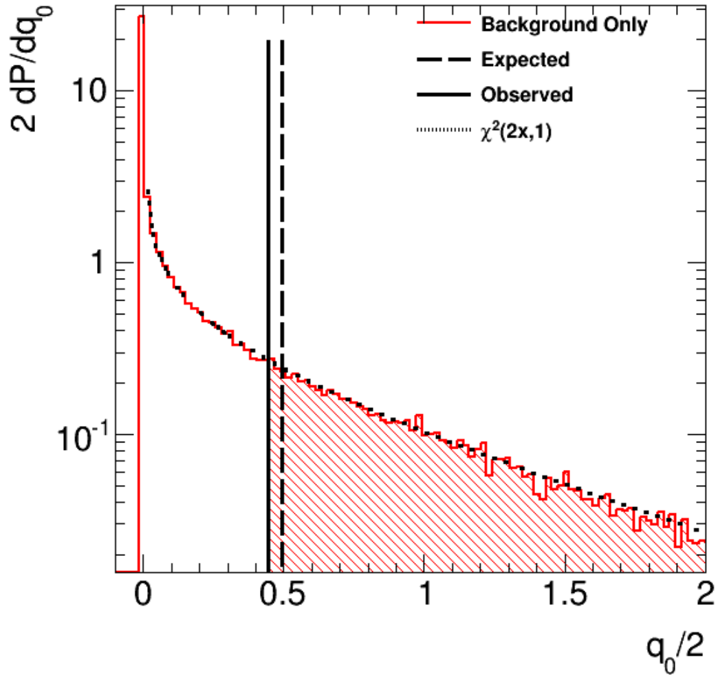
Figure 6.4: PDF of the background only hypothesis as a function of q_0 for the combination of the fully-leptonic and semi-leptonic channels. PDFs are determined using toy MC. The dashed black line represents the expected value of q_0 while the solid black line represents the observed value of q_0 seen in the data. The shaded area to the right of this line represents the null p-value or the integral of the background hypothesis in the signal-like region. The dotted black curve shows a \chi^2 distribution for 1 degree of freedom with which it can be seen is a good approximation of the the background only PDF.
