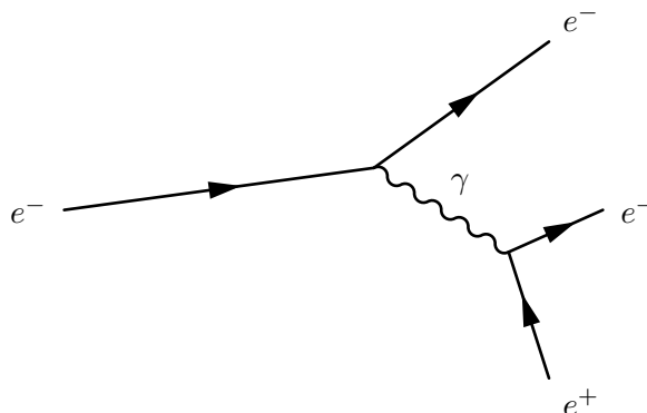
Figure 5.7: Feynman diagram showing combination of bremsstrahlung and pair-production processes that lead to electron charge mis-identification. In this case, we start with an electron and end with two electrons and a positron. For electron charge mis-identification to occur, the positron would have to be the only final state particle that is selected.
