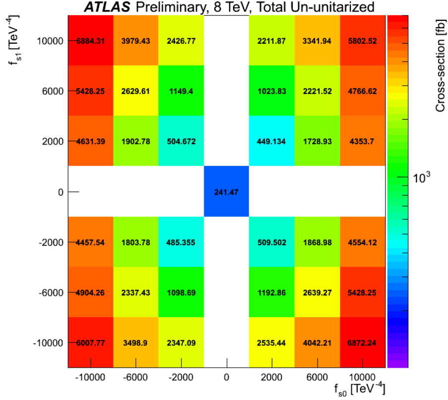
Figure 5.2: Total cross-section for non-unitarized aQGC signal samples as a function of f_{S,0}/\Lambda^4 vs f_{S,1}/\Lambda^4 . The total SM cross-section is shown at f_{S,0}/\Lambda^4 = f_{S,1}/\Lambda^4 = 0 for comparison. Those points that are white have not been evaluated.
