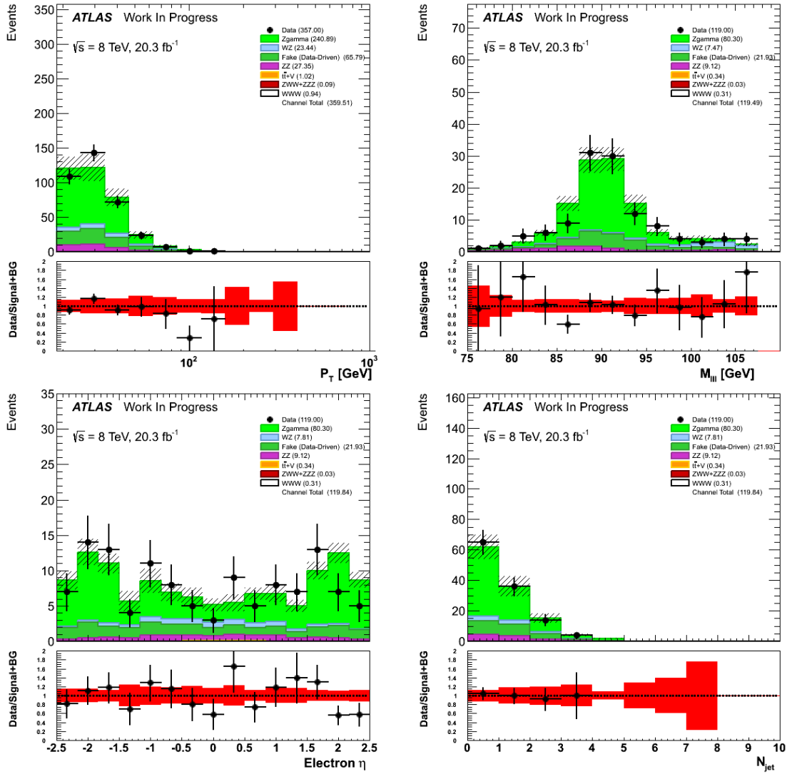
Figure 5.6: Three lepton Z\gamma control region. Distribution are shown for the lepton p_T , three lepton invariant mass ( m_{ll} ), electron \eta , and jet multiplicity.
