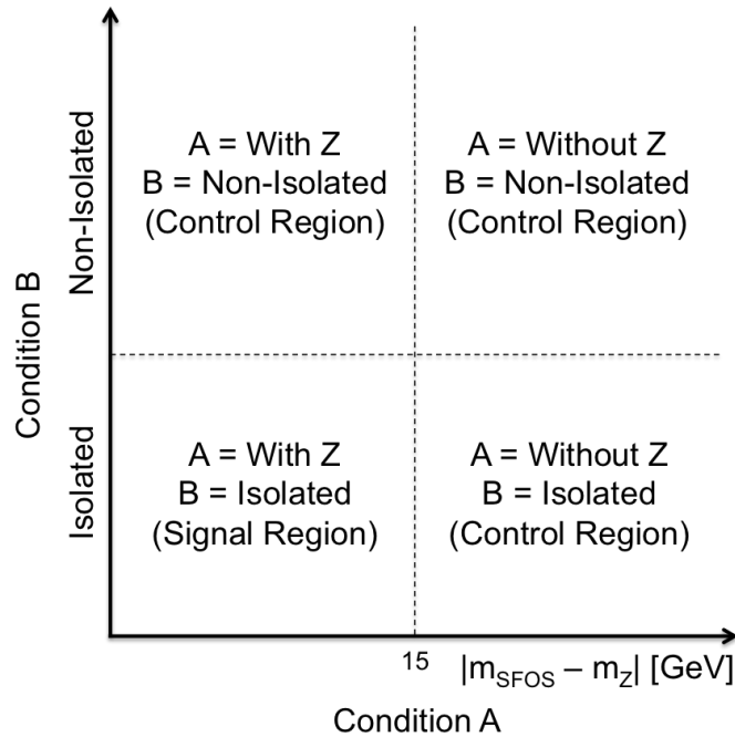
Figure 5.4: Diagram of the four different regions used in the 2D sideband method as defined from cuts on the 2D plane of isolation versus the Z boson SFOS mass parameter.
