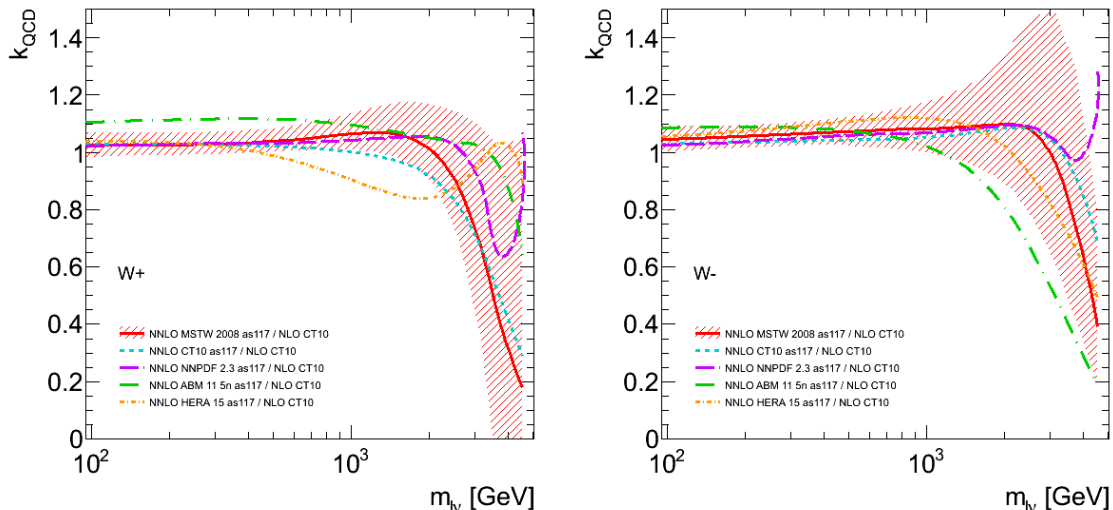
Figure 2.3: Plot of k_{\text{QCD}} = \sigma(\text{NNLO})/\sigma(\text{NLO}) for charged Drell-Yan production using various PDF sets as a function of the invariant mass of the W when it decays leptonically, m_{l\nu} , as studied for the background estimate in a search for leptonically decaying exotic W' bosons [3, 4]. Several different PDFs are compared: MSTW 2008 [2] (solid red line), CT10 [5] (narrow dashed blue line), NNPDF 2.3 [6] (wide dashed purple line), ABM 11 [7] (wide dashed-dotted green line), and HERA 1.5 [8] (narrow dashed-dotted orange line). Ratios are shown of the various PDFs at NNLO with respect to the CT10 PDF set at NLO. All PDF sets use a strong coupling constant of \alpha_s = 0.117 . The 90% CL uncertainty on the MSTW 2008 NNLO PDF set is also shown (hashed red band).
