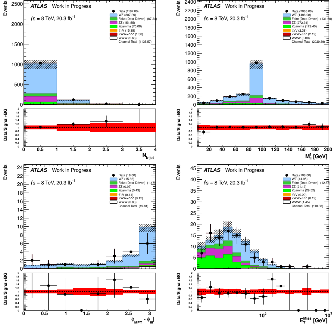
Figure 5.32: Distributions showing data compared to the signal plus background estimate in the 2 SFOS region at each stage of the selection before the cuts are applied to the given distribution. Plots should be read clockwise starting from the top left. Referring to Table 5.22, the top left plot is shown before cut number 2 is applied, followed by cuts number 3, 4, and 5.
