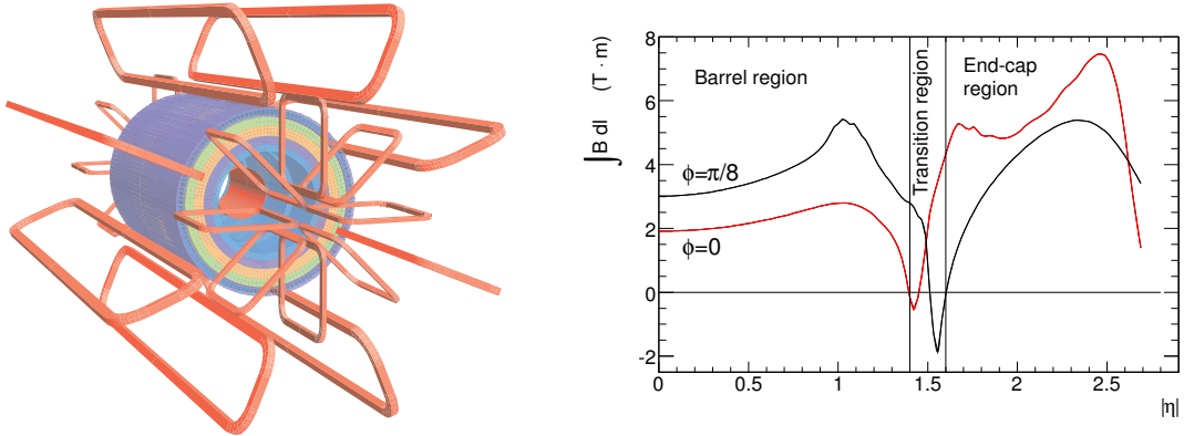
Figure 4.14: (Left) Diagram of MS toroid magnet geometry shown in red. The tile calorimeter is also shown. (Right) Predicted field strength of the MS magnet system as a function of |\eta| for \phi = 0 in red and \phi = \pi/8 in black.
