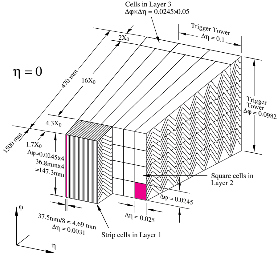
Figure 4.8: A diagram of one ECAL barrel module covering 22.5^\circ in azimuth. When inside the detector, it is oriented as indicated by the axes.
