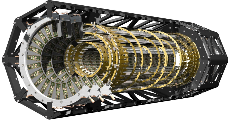
Figure 4.5: A cut-out diagram of the ATLAS pixel detector showing the arrangement of the pixel modules (green) in three layers of the barrel and three layers of one end-cap system. Some of the support structure is also shown.
