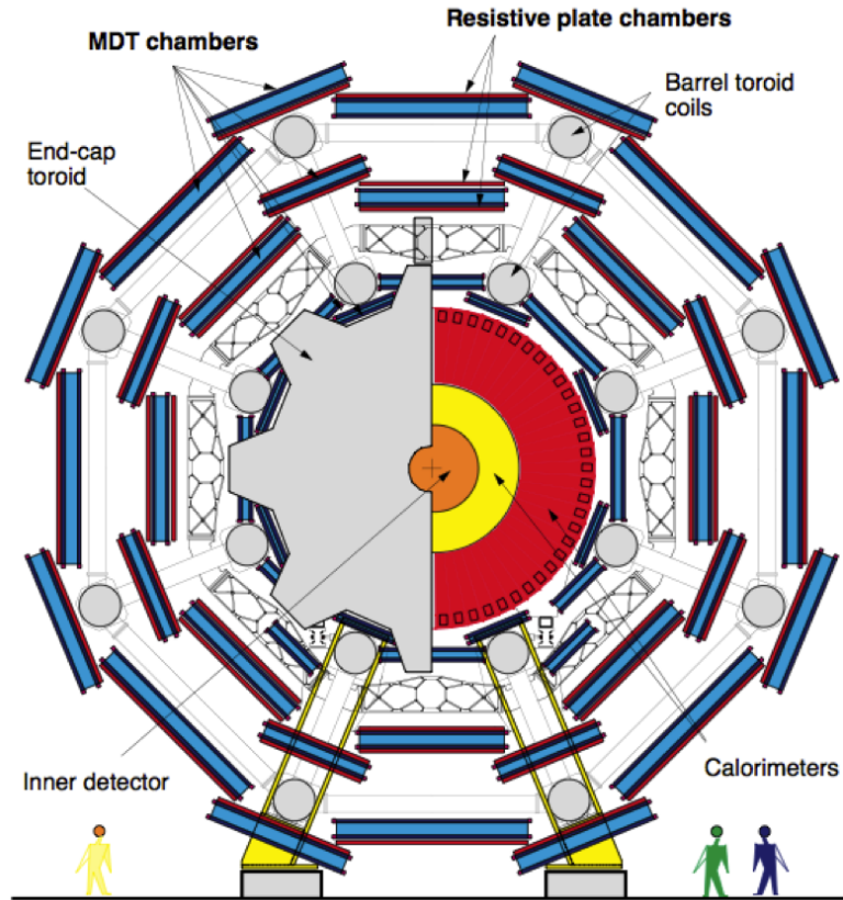
Figure 4.12: A cross-section of the MS in the transverse ( r - \phi ) plane viewed from one end of the detector. The MDT chambers, RPCs, and barrel and end-cap toroids of the MS system are clearly labeled. The barrel toroid coils extend in to and out of the page while only half of the end-cap toroid is shown to reveal the ID and calorimeter systems. The LHC beam pipe runs through the center.
