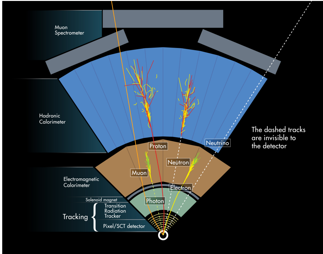
Figure 4.2: A diagram of one wedge of the ATLAS detector as viewed from looking down the LHC beam line. The sub-detector components are shown along with the particles that typically come from the collision. The paths of the particles are shown to indicate how each particle interacts with the detector.
