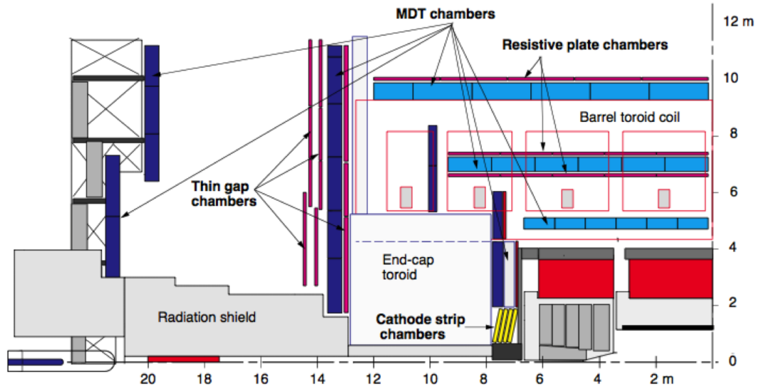
Figure 4.13: One quadrant of the MS as viewed in the R - z plane. The MDT chambers, RPCs, TGCs, CSCs are clearly indicated, as are the the end-cap and barrel toroids. Support structures, shielding and the calorimeter and ID systems are also drawn. The LHC beam pipe runs from left to right along the bottom.
