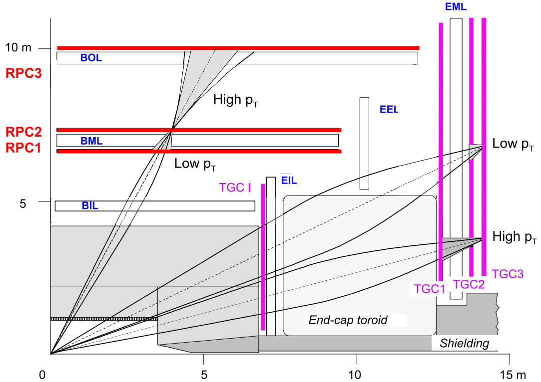
Figure 4.18: Layout of the trigger components for one quadrant in the r - z plane. RPC and TGC chambers are clearly labeled. Possible muon trajectories are seen for low and high p_T roads formed by the trigger algorithm (see Sec. 4.4).
