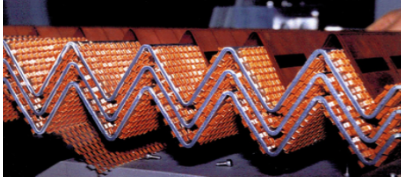
Figure 4.7: Photo of three ECAL sampling layers showing its accordion-like structure. In the picture, the horizontal directions corresponds to the radial direction when the detector is in position, which is the direction the LHC products would follow.
