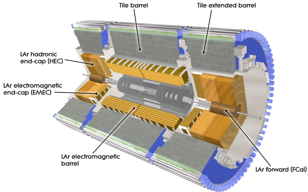
Figure 4.6: Diagram of ATLAS calorimeter system with cut-out portion to allow a view of the nested sub-components.
