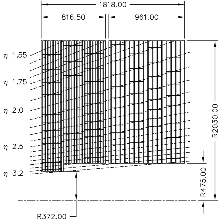
Figure 4.10: A schematic showing one quadrant of the HEC system in the R - z plane. The dashed lines indicate the pointing direction achieved by the segmentation of the readouts. Dimensions are in mm.
