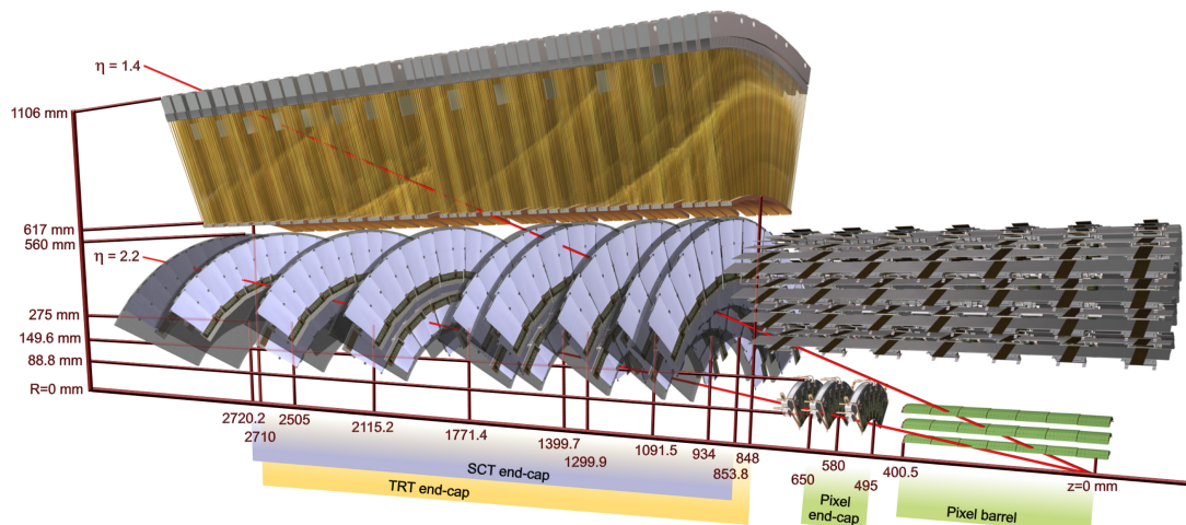
Figure 4.4: Diagram of the ATLAS Inner Detector (ID) showing a wedge of the end-cap system as well as a part of the SCT and Pixel barrel systems. The detector systems are clearly labeled. The LHC beam pipe is axial to the system but is not shown. Trajectories of two charged tracks with a p_T = 10 GeV are shown along \eta = 1.4 and \eta = 2.2 as indicated by the solid bright red lines.
