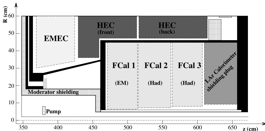
Figure 4.11: A schematic showing the end-cap of the ECAL, the two HEC modules, and the three FCAL modules, as well as additional shielding, in one quadrant of the ATLAS detector, as viewed in the R - z plane. The R -direction is shown with a larger scale than in the Z -direction.
