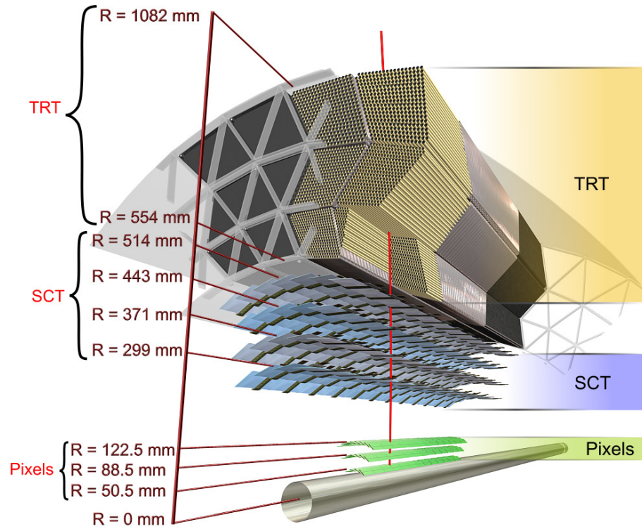
Figure 4.3: Diagram of the ATLAS Inner Detector (ID) showing a wedge of the barrel system. The three detector systems are clearly labeled. The LHC beam pipe is axial to the system and is shown at the bottom of the diagram.
