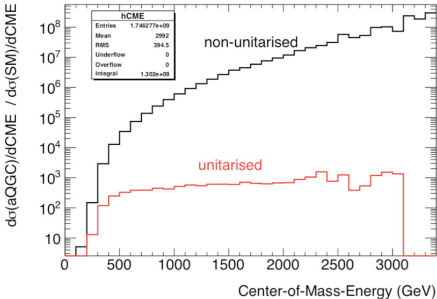
Figure 2.10: The unitarized and non-unitarized differential cross sections as a function of \sqrt{s} for the EFT prediction with f_{S,0}/\Lambda^4 = 6 \times 10^{-7} \text{ GeV}^{-4} divided by the SM values. The form-factor function from Eq. (2.43) with n = 1 and \Lambda_U = 180 \text{ GeV} is used for unitarization. The choice of parameters here serves merely as a demonstration.
