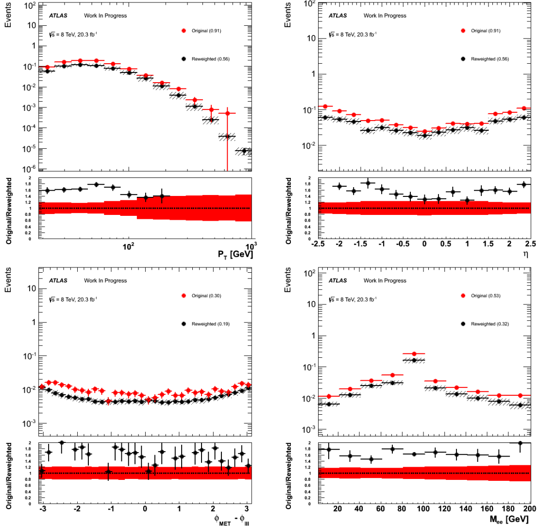
Figure 5.11: Validation of the charge mis-ID rates comparing MC ZZ \rightarrow l\ell ee ( \ell = e, \mu ) samples re-weighted with the charge mis-ID rates measured in the MC Z \rightarrow ee sample to the original MC predictions. Distribution of lepton p_T , \eta , \Delta\phi(3l, E_T^{Miss}) , and the Same-sign di-electron invariant mass.
