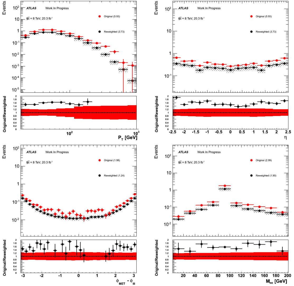
Figure 5.10: Validation of the charge mis-ID rates comparing MC WZ \rightarrow \ell e e ( \ell = e, \mu ) samples re-weighted with the charge mis-ID rates measured in the MC Z \rightarrow ee sample to the original MC predictions. Distribution of lepton p_T , \eta , \Delta\phi(3l, E_T^{Miss}) , and the Same-sign di-electron invariant mass.
