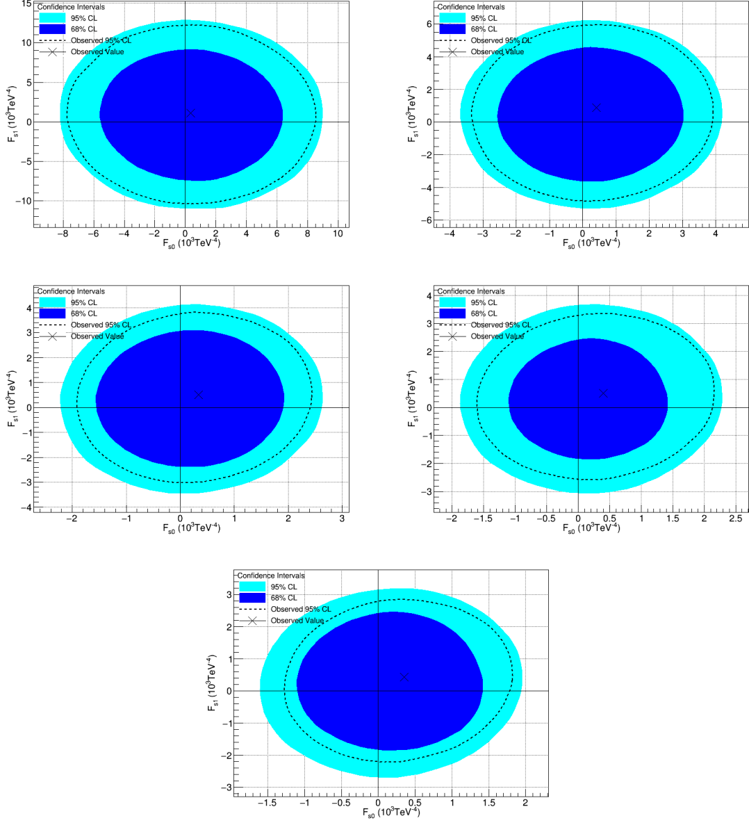
Figure 6.7: Two-dimensional limits at 95% CL as a function of f_{S,0}/\Lambda^4 vs f_{S,1}/\Lambda^4 on the combination of the fully-leptonic and semi-leptonic channels for the non-unitarized case (Top Left) and three different choices of the unitarization scale, \Lambda_U : 3 TeV (Top Right), 2 TeV (Middle Left), 1 TeV (Middle Right), and 0.5 TeV (Bottom Center).
