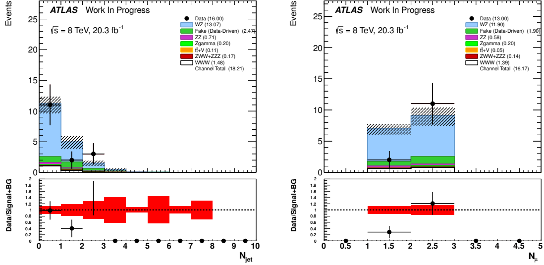
Figure 5.31: Distributions showing data compared to the signal plus background estimate in the 1 SFOS region at each stage of the selection before the cuts are applied to the given distribution. Referring to Table 5.20, the left plot is shown before cut number 6 is applied. The right plot is shown after all cuts have been applied.
