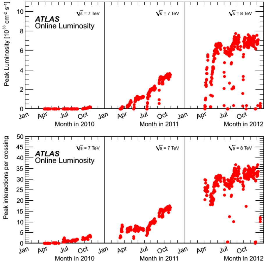
Figure 3.4: (Top) The peak luminosity from the LHC as a function of time for 2010, 2011, and 2012 data-taking periods and (Bottom) the peak number of pileup interactions as a function of time as recorded by ATLAS. The peak luminosity and pileup interactions have both increased since the LHC began operation in 2010. The gaps in recorded values are due to technical stops and long shutdowns for maintenance and upgrade work.
