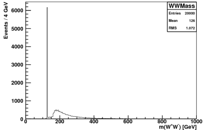
Figure 2.8: Invariant mass distribution of two opposite-sign W bosons in WWW events at truth level. The Higgs mass peak is clearly visible around 125 GeV.
