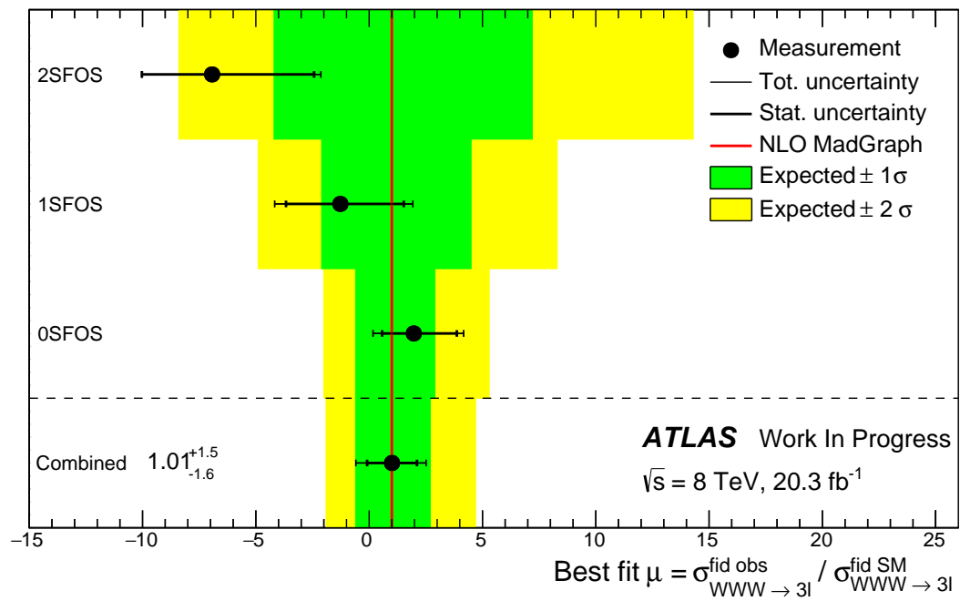
Figure 5.36: The expected and observed best fit signal strength, \mu , and uncertainties for each of the fully-leptonic signal regions and for the combination of the three regions.
