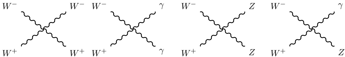
Figure 2.6: Feynman diagrams of EW QGC couplings
