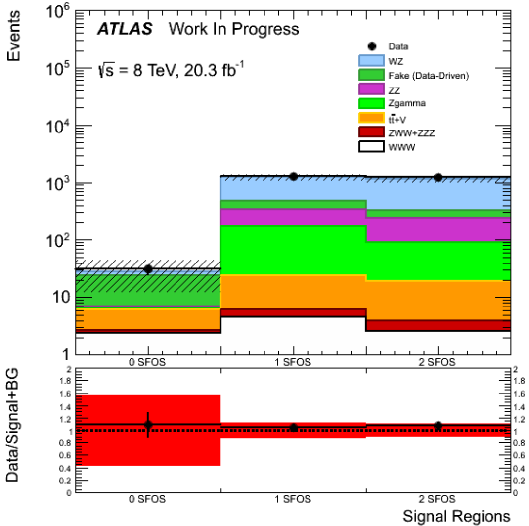
Figure 5.20: Yields at event pre-selection in the 0, 1 and 2 SFOS regions. The most important systematic uncertainties (discussed in section 5.6) are shown, namely from the fake estimates and the uncertainties on the WZ and ZZ k-factors.
