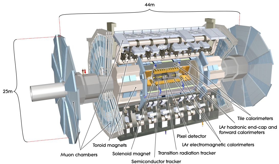
Figure 4.1: A diagram of the ATLAS detector where the detector has been artificially opened up to reveal the LHC beam line and the various sub-detector components within. The sub-detector components are labeled as such.
