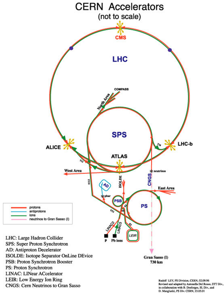
Figure 3.3: Diagram of the different accelerators in the CERN accelerator complex [9]. Those relevant for the LHC are the LINAC2, PSB, PS, SPS, and the LHC itself. The ATLAS detector is labeled at the bottom of the LHC ring.
