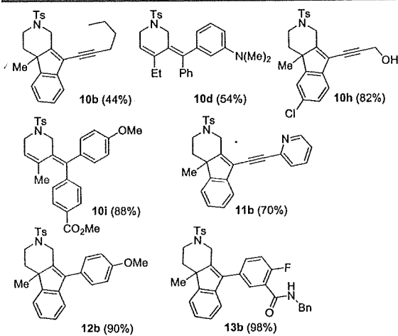
Figure 1. Cross-coupling products of vinyl iodides.
