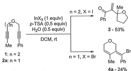
Scheme 1. Divergent Cyclization Catalyzed by In(III)
