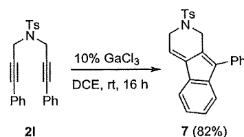
Scheme 2. Diphenyldiyne Cycloisomerization
