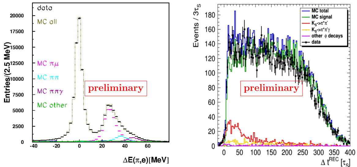
Figure 3. Left: distribution of \Delta E(\pi, e) = E_{\text{miss}} - p_{\text{miss}} for all selected events after normalization procedure. Due to a non-registered neutrino in the decay, the \Delta E(\pi, e) for K_S \rightarrow \pi e \nu events takes value to zero. Right: spectrum of selected events in \phi \rightarrow K_S K_L \rightarrow \pi^\pm l^\mp \nu 3\pi^0 decay as a function of time interval \Delta t .
