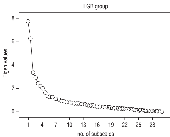
Figure 2. Scree plot for the whole sample (LGB) – analysis with an SMNE scale
