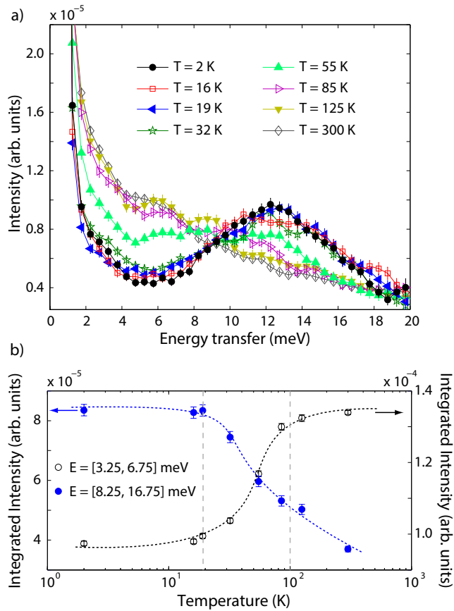
FIG. 8. (a) Neutron scattering intensity vs energy transfer for various temperatures shown for [0, 0, L] = [-2, 12] r.l.u. and [H, H, 0] = [0.1, 0.5] r.l.u., using the E_i=25 meV data from CNCS. (b) Temperature dependence of the integrated scattering intensity associated with the formation of the spin gap at E = [3.25, 6.75] meV (black curve), and integrated intensity at the resonant excitation energy E = [8.25, 16.75] meV (blue curve), are shown to characterize the magnetic excitation in Fig. 7. The spin gap and the related spin excitation at 12 meV start to form below |\Theta_{CW}| \sim 85 K and appear to be fully developed below T_g , consistent with the evolution of the static spin correlations. Lines are guides to the eye.
