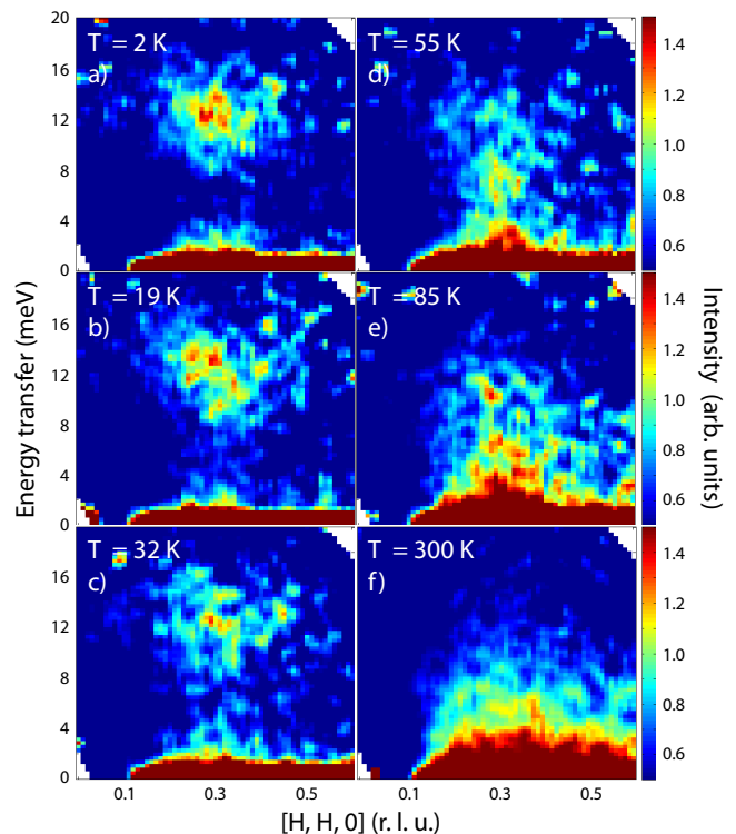
FIG. 7. Temperature evolution of the resonant spin excitation as measured on CNCS. Inelastic scattering intensity for an integration range of L = [-2, 12] r.l.u. and [H, -H, 0] = [-0.2, 0.2] r.l.u. is shown for (a), T = 2 K, (b) T = 19 K, (c) T = 32 K, (d) T = 55 K, (e) T = 85 K, and (f) T = 300 K. A spin gap of \sim 9 meV gradually opens below \sim 85 K and is fully developed below the freezing temperature T_g \sim 19 K. The gap correlates with the short-range static spin correlations shown as in Figs. 2 and 3. Note that the data have only been corrected for detector efficiency.
