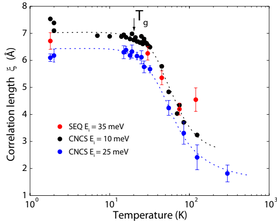
FIG. 3. The correlation length within the plane of the bilayers extracted from cuts through the elastic scattering at \mathbf{Q}=(1/3, 1/3, L) for both the SEQUOIA and the CNCS data. The short-range spin correlations gradually develop at temperatures as high as the Curie Weiss temperature at \sim 100 K and increase to their maximum value of \xi \sim 6.5 - 7.5 Å below the freezing temperature T_g . There is no sharp anomaly at T_g , in contrast to the observed cusp in the ZFC susceptibility, typical for this family of materials. Note that the difference in absolute values of the correlation length from CNCS data for E_i = 10 and 25 meV is a result of the coarser \mathbf{Q} -resolution at higher incident energy and a different binning range in L . For details of the integration and fitting, see text. The error bars are \pm 1\sigma .
