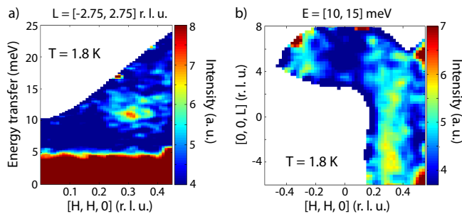
FIG. 6. Two-dimensional resonant spin excitation observed on SEQUOIA at 1.8 K. (a) Inelastic scattering integrated over L = [-2.75, 2.75] and [H, -H, 0] = [-0.2, 0.2] r.l.u. is shown. A gapped spin excitation positioned at \mathbf{Q} = (1/3, 1/3, L) is observed at \sim 12 meV. It has a bandwidth of \sim 8 meV. (b) Constant energy slice within the [H, H, L] scattering plane, integrated from E = [10, 15] meV. The resonant spin excitation is well localized at \mathbf{Q} = (1/3, 1/3, L) and has a clear two-dimensional, rod-like character. Its \mathbf{Q} -width is comparable to the width of the diffuse elastic scattering.
