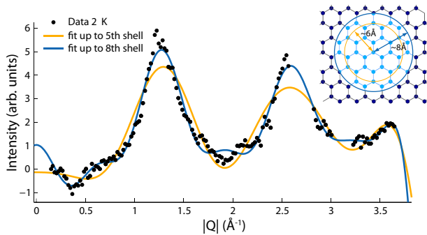
FIG. 4. Powder-averaged elastic neutron data for \text{LuCoGaO}_4 at T = 1.8 K as measured on CNCS with E_i = 10 meV. Fits to Eqn. 1 show good agreement with short-range, two-dimensional magnetic correlations extending beyond the 5th nearest neighbor shell at \sim 6 Å. The best fit to the data is obtained including magnetic correlations extending up to the 8th nearest neighbor shell at \sim 8 Å, fully consistent with the correlation length determined from the lineshape analysis in Fig. 3. A high temperature, 300 K data set has been subtracted from the data as paramagnetic background, and scattering from the sample holder at Q \sim 2.7 and \sim 3.15 Å has been excluded from the data and fit. The top right figure illustrates how the magnetic correlations are built up in the quasi two-dimensional shell model. 16
