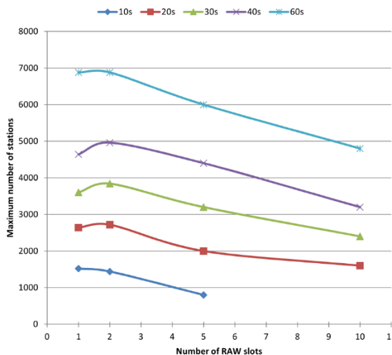
Figure 3: Maximum number of stations for 16 TIM groups
