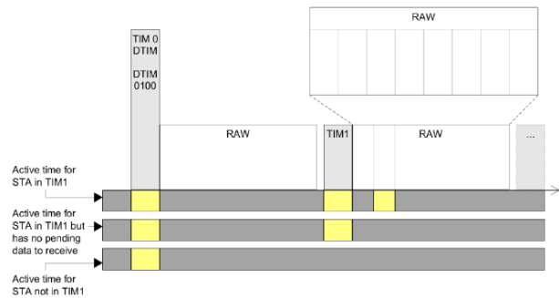
Figure 2: Timeline between beacon intervals. Almost all time between beacons is used as RAW period.
