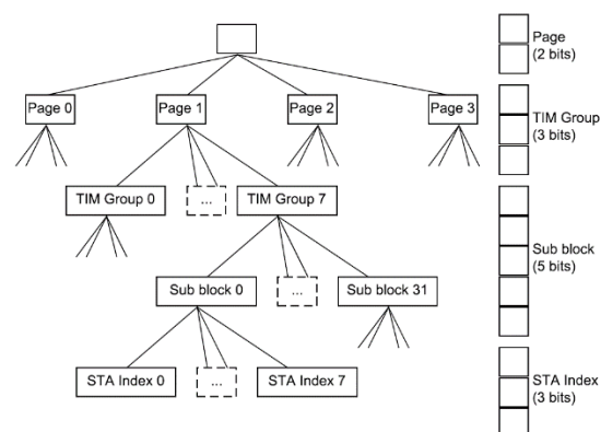
Figure 1: Hierarchical structure of STAs based on AIDs assigned by the AP
