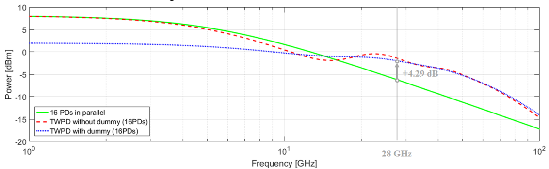
Figure 4: Simulated output power of the different structures when each PD generates 2 mA peak-to-peak current (2V reverse voltage)
