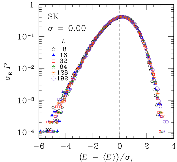
FIG. 7: (Color online) Scaled ground-state energy distributions for several system sizes for the one-dimensional Ising chain with \sigma = 0.00 (MF phase, SK model). The dashed vertical line is a guide to the eye to illustrate the skewness of the distribution. The data show little spread in the tails suggesting a weaker dependence on L than for larger values of \sigma .
