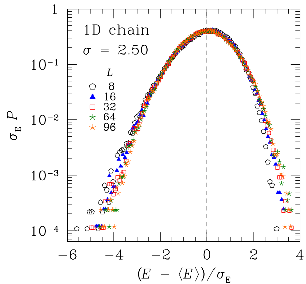
FIG. 8: (Color online) Scaled ground-state energy distributions for several system sizes for the one-dimensional Ising chain with \sigma = 2.50 (SR phase). The dashed vertical line is a guide to the eye to illustrate the skewness of the distribution. The data show a moderate dependence on the system size.
