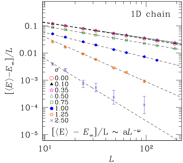
FIG. 10: (Color online) Mean [(\langle E \rangle - E_\infty)/L] as a function of system size L for several values of \sigma . The data are expected to decay as a power of the system size with an exponent \omega . Note that for the SK limit \omega \approx 2/3 at T = 0 in agreement with other predictions (Refs. 43, 7, 11, and 8) [see Fig. 11 for \omega(\sigma) ] and that for \sigma = 2.5 we obtain \omega = 2.29(17) .
