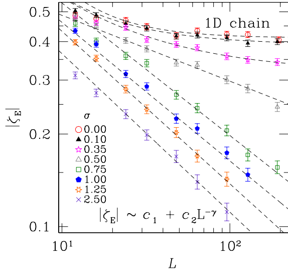
FIG. 9: (Color online) Skewness \zeta_E as a function of system size L for several values of \sigma . For \sigma < 0.5 (MF phase) the data scale as \zeta_E \sim c_1 + c_2 L^{-\gamma} with c_1 > 0 [Eq. (6)] thus tending to a constant in the thermodynamic limit. For \sigma \geq 0.5 the skewness decays with a power-law behavior, i.e., c_1 = 0 (fits done for L \geq 64 ). Note that for \sigma > 1 , for which T_c = 0 , \gamma \approx 0.5 in agreement with the results for the ladder system presented in Sec. III.
