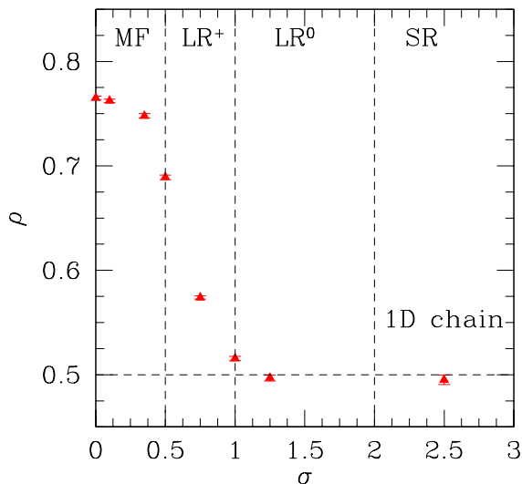
FIG. 13: (Color online) Exponent for the energy fluctuations \rho as a function of \sigma [see Eq. (2)]. For \sigma \rightarrow 0 \rho \approx 3/4 in agreement with Refs. 45, 11, and 7. For \sigma \rightarrow \infty , \rho \rightarrow 1/2 , as predicted by the central limit theorem, and in agreement with the results on the ladder system presented in Sec. III B.
