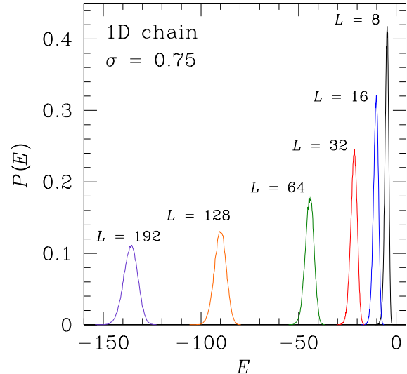
FIG. 5: (Color online) Unscaled energy distributions for several system sizes for the one-dimensional Ising chain with \sigma = 0.75 ( \text{LR}^+ phase).
