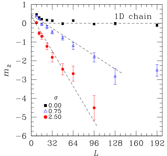
FIG. 15: (Color online) Coefficient m_2 to the quadratic correction term in the modified Gumbel distribution, Eq. (22), as a function of system size for several values of the power-law exponent \sigma . The data show that m_2 converges to a value close to zero for the SK model in the thermodynamic limit thus suggesting that the energy distributions of the SK model are possibly well described by a modified Gumbel distribution function in agreement with results from Ref. 7. For all \sigma > 0 , m_2 tends to a finite negative value in the thermodynamic limit. For large values of \sigma , m_2 dominates thus showing that in the SR universality class the limiting probability distribution is well described by a Gaussian. The dashed lines are guides to the eye.
